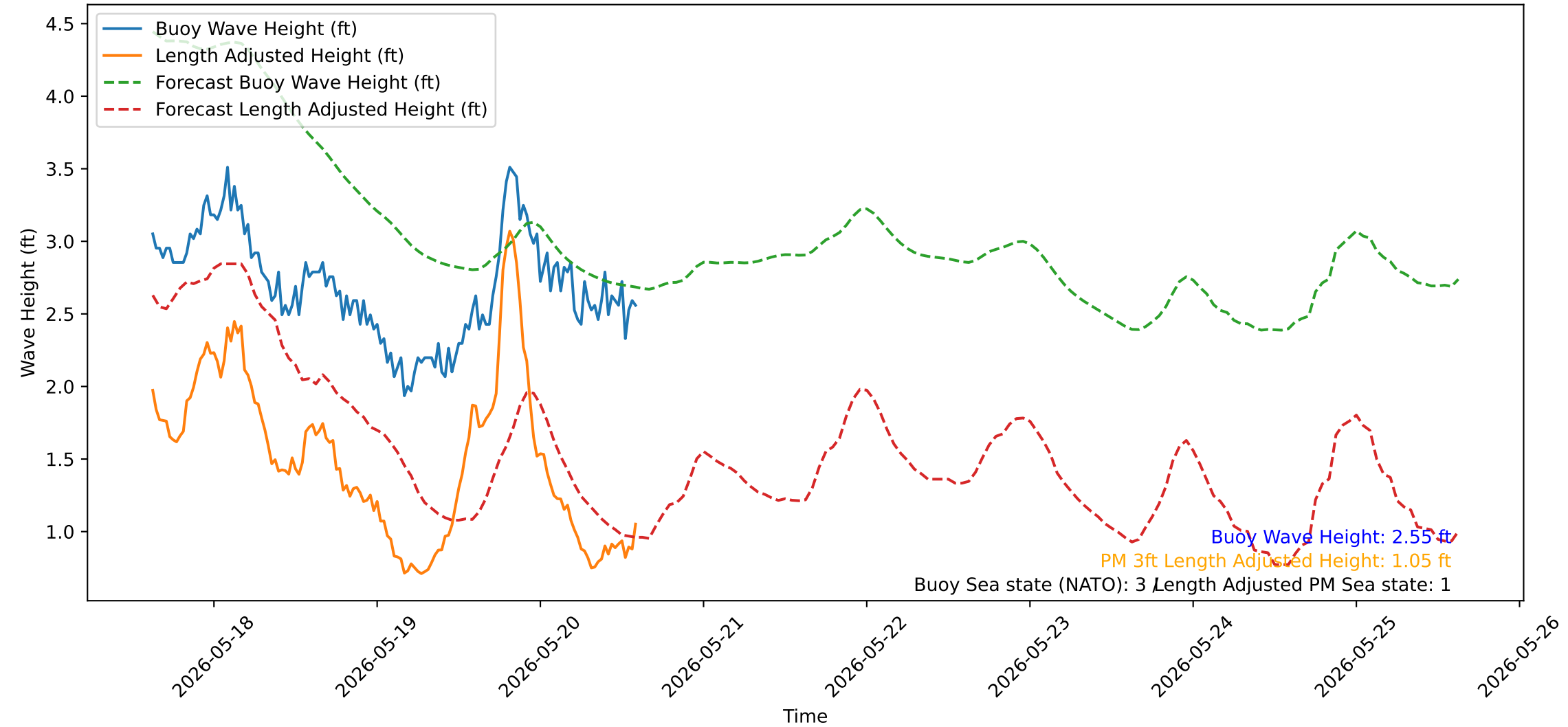
Wave Heights over Time for Red Beach at 2026-05-20 14:50:53
