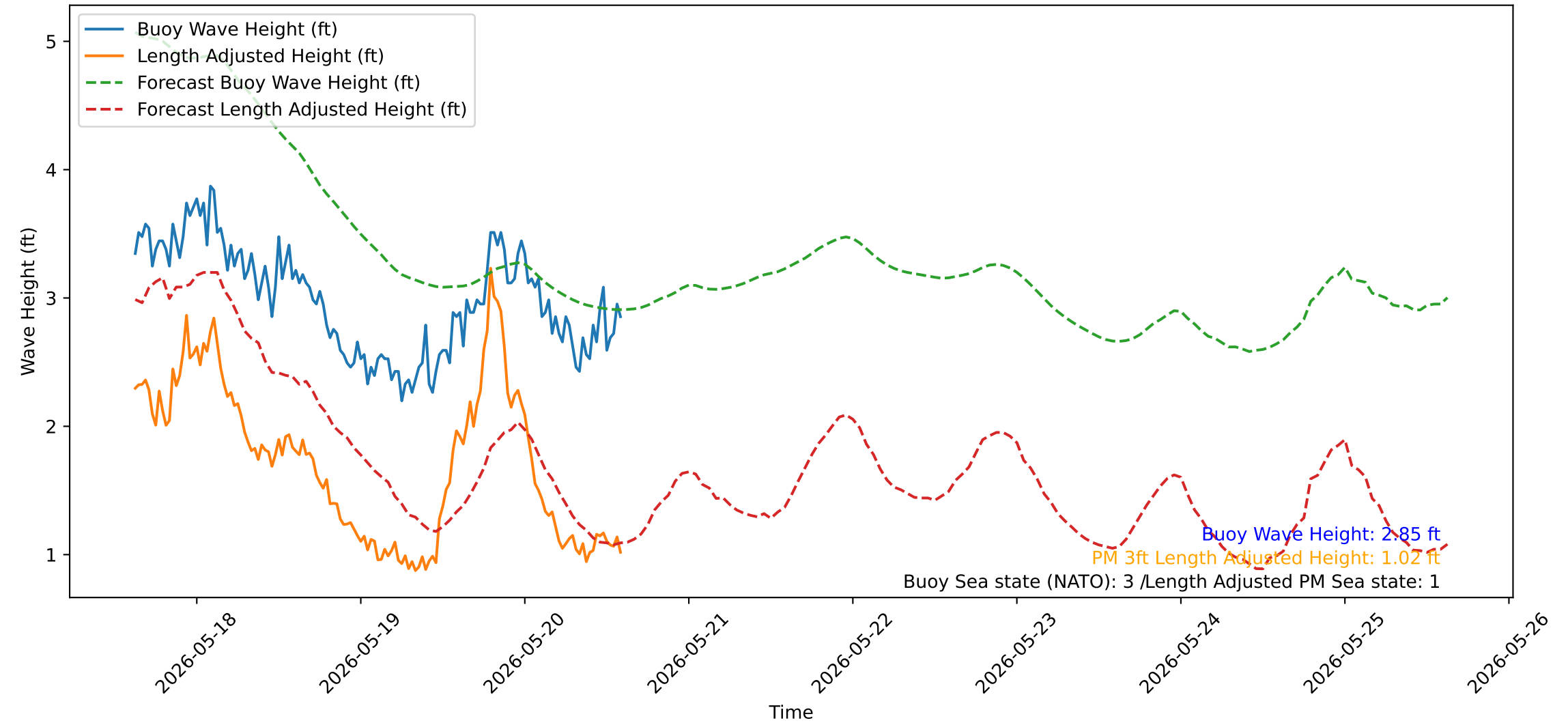
Wave Heights over Time for Oceanside Harbor at 2026-05-20 14:50:32
