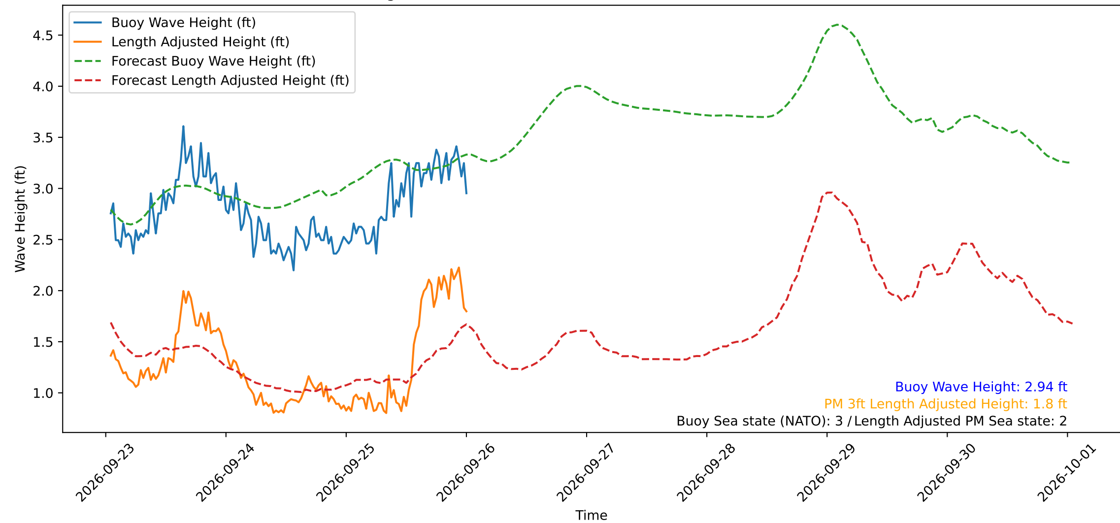
Wave Heights over Time for Oceanside Harbor at 2026-09-26 01:00:30
