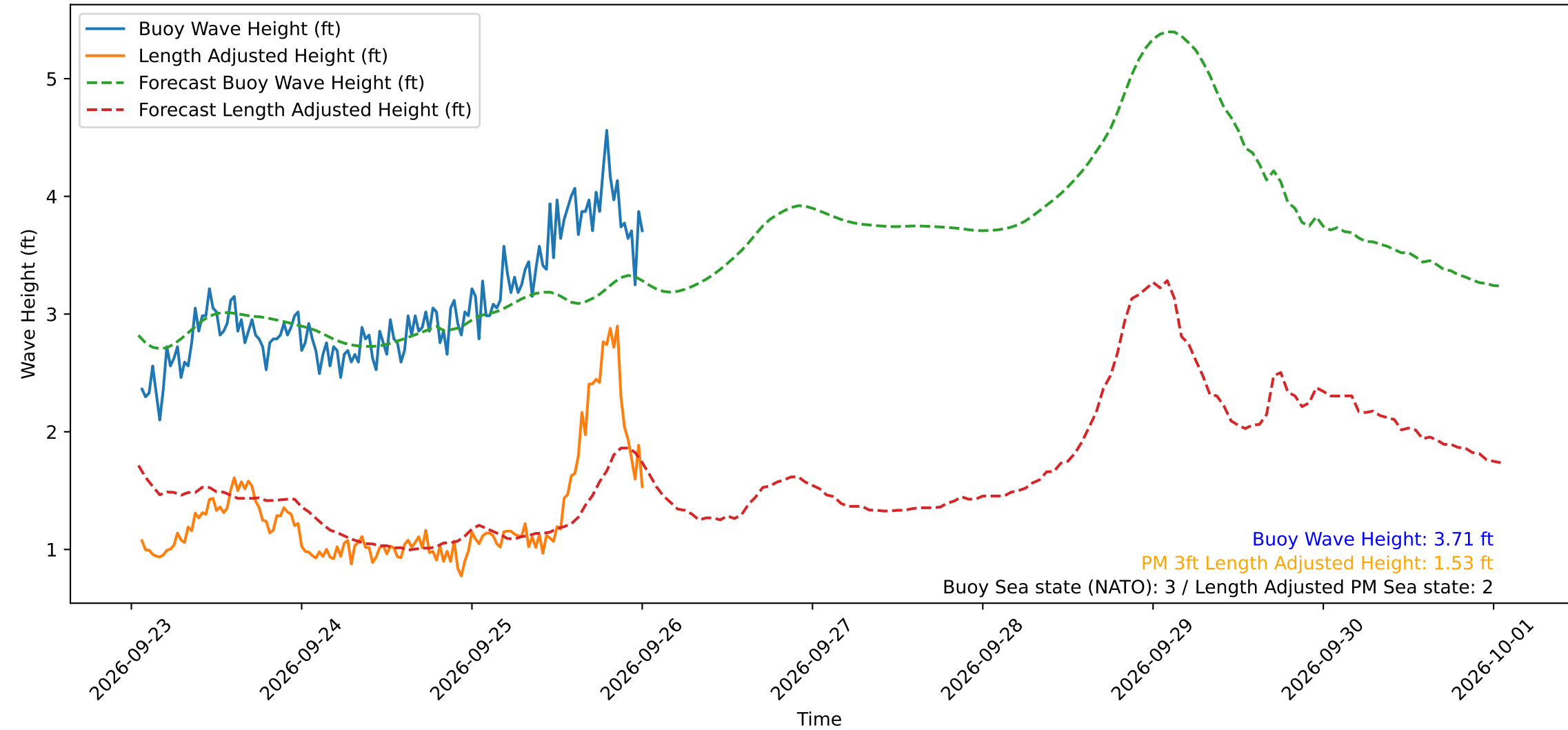
Wave Heights over Time for Green Beach at 2026-09-26 01:01:12
