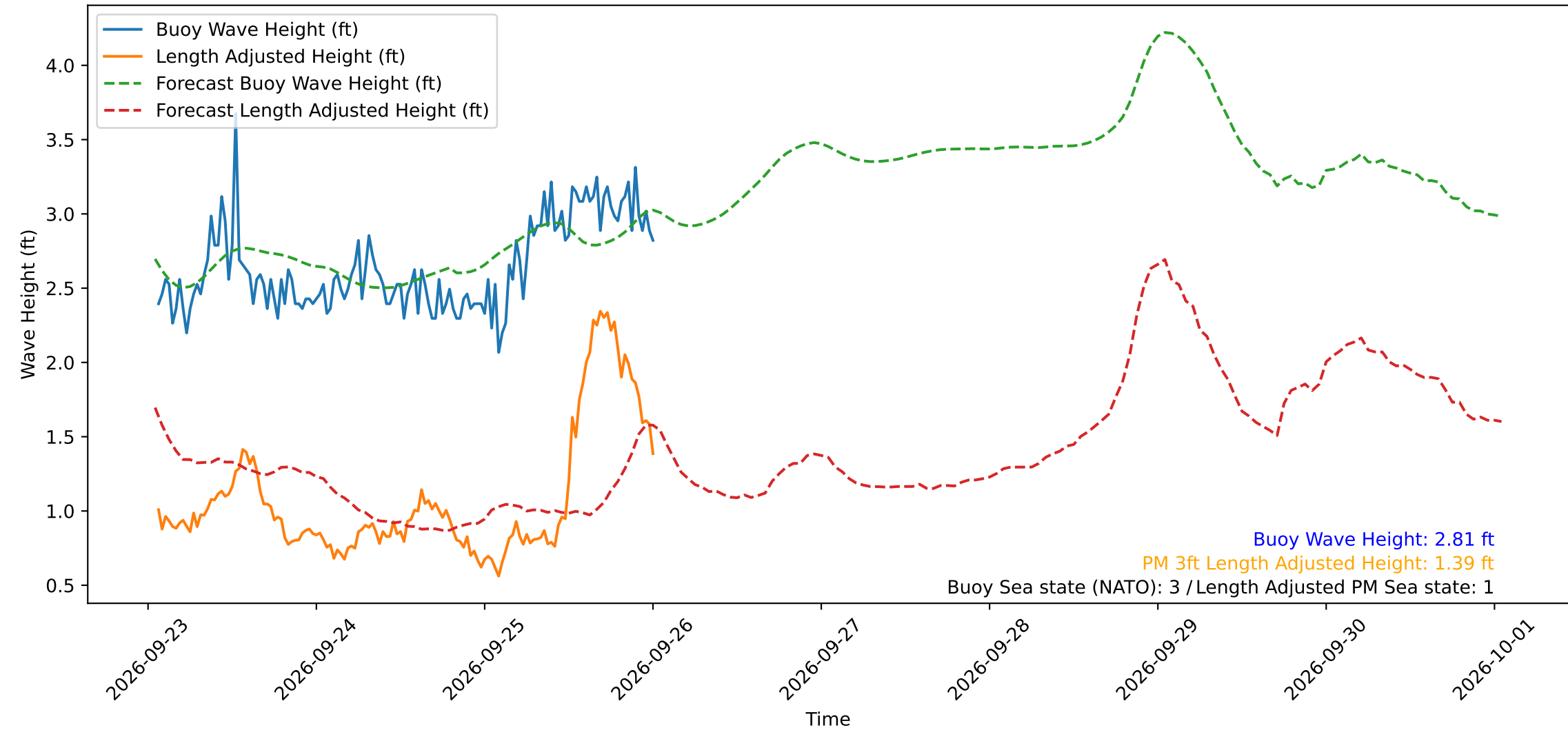
Wave Heights over Time for Red Beach at 2026-09-26 01:00:50
