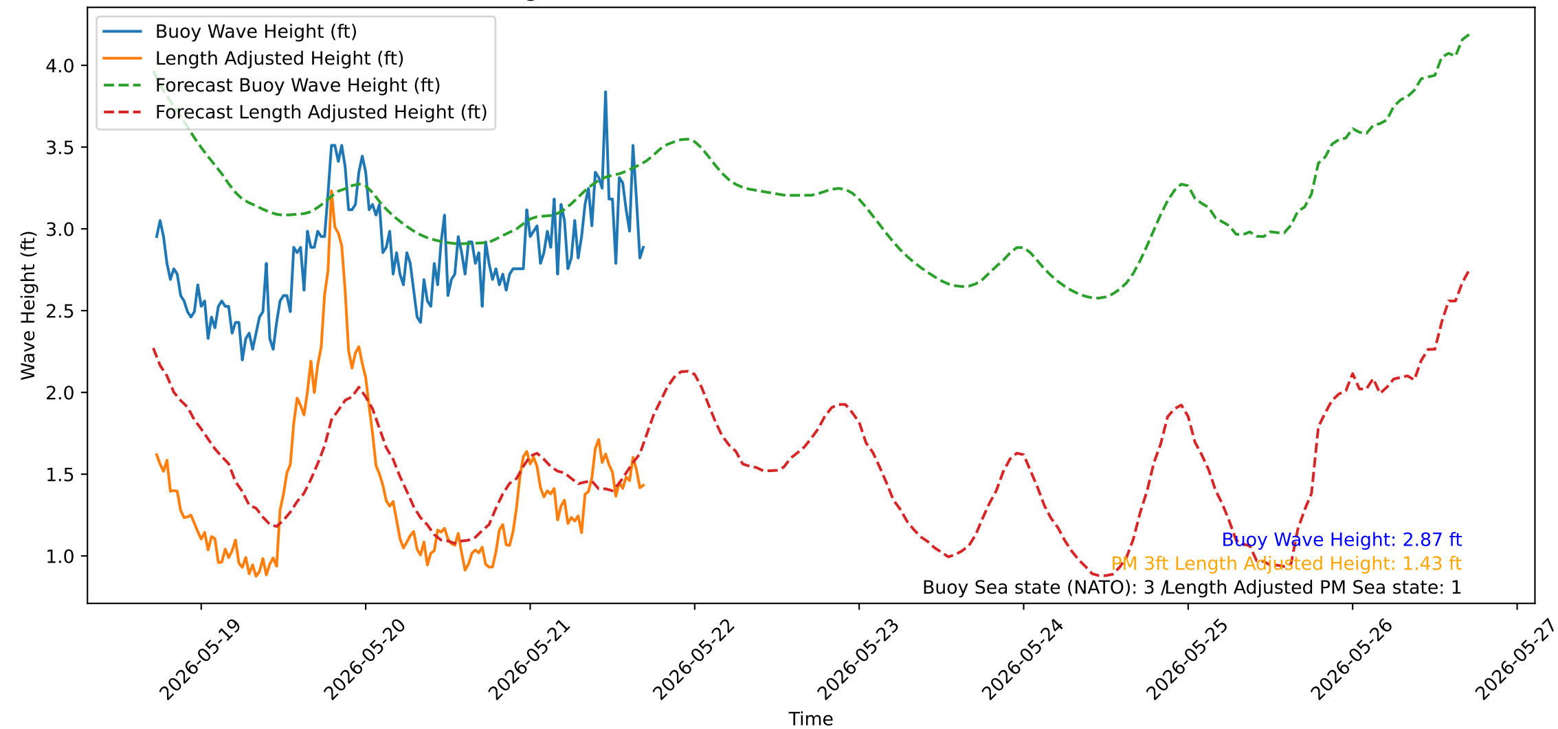
Wave Heights over Time for Oceanside Harbor at 2026-05-21 17:20:32
