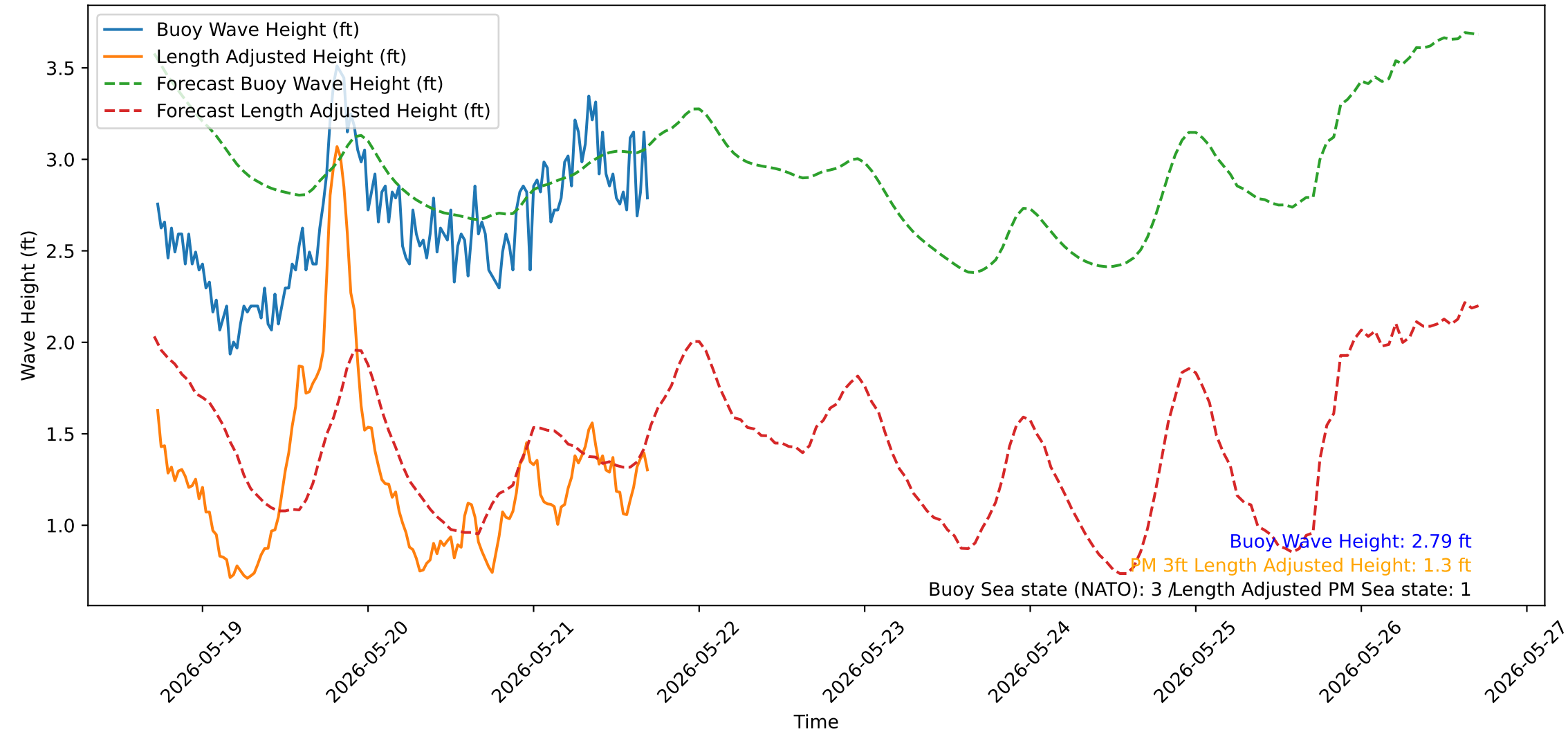
Wave Heights over Time for Red Beach at 2026-05-21 17:20:53
