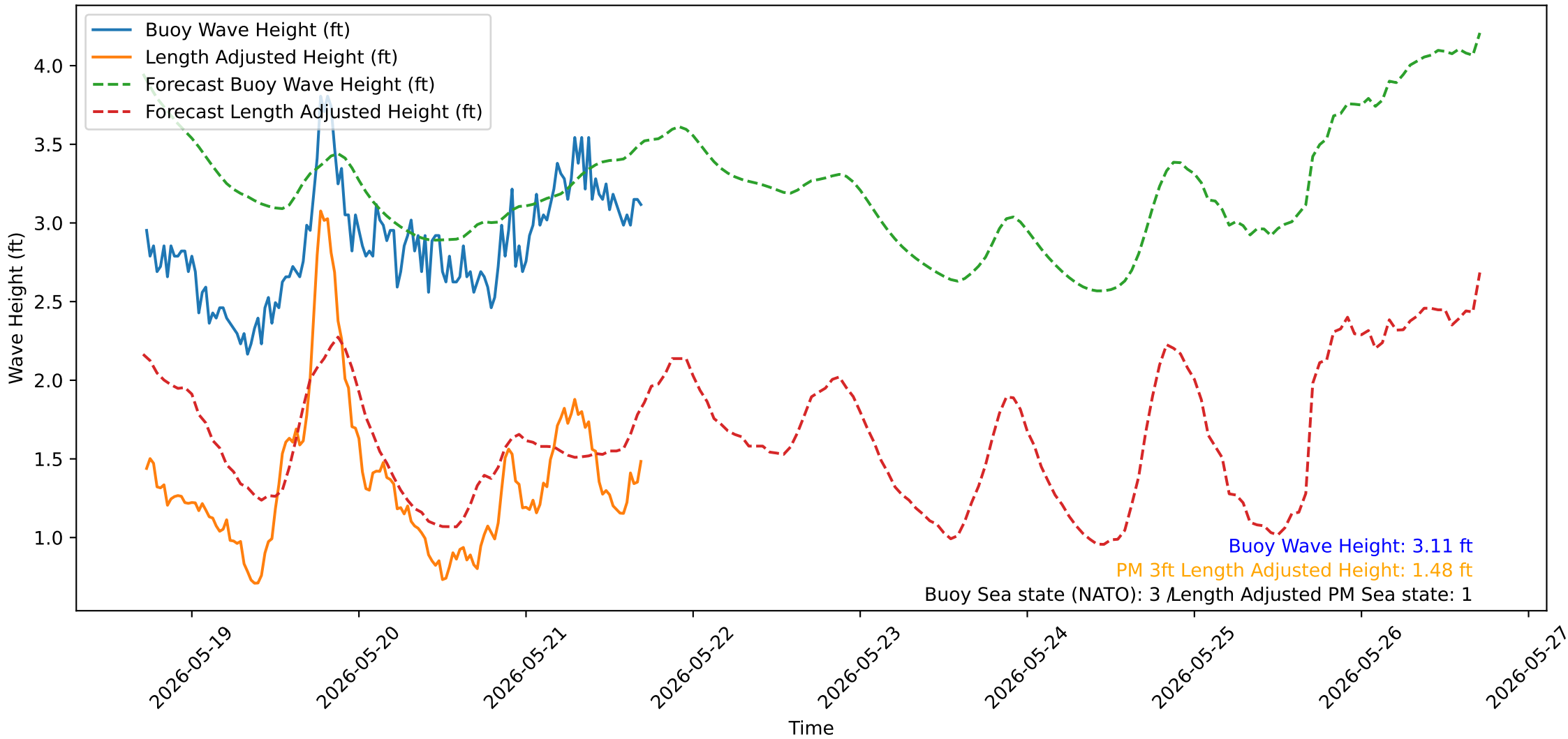
Wave Heights over Time for Green Beach at 2026-05-21 17:21:15
