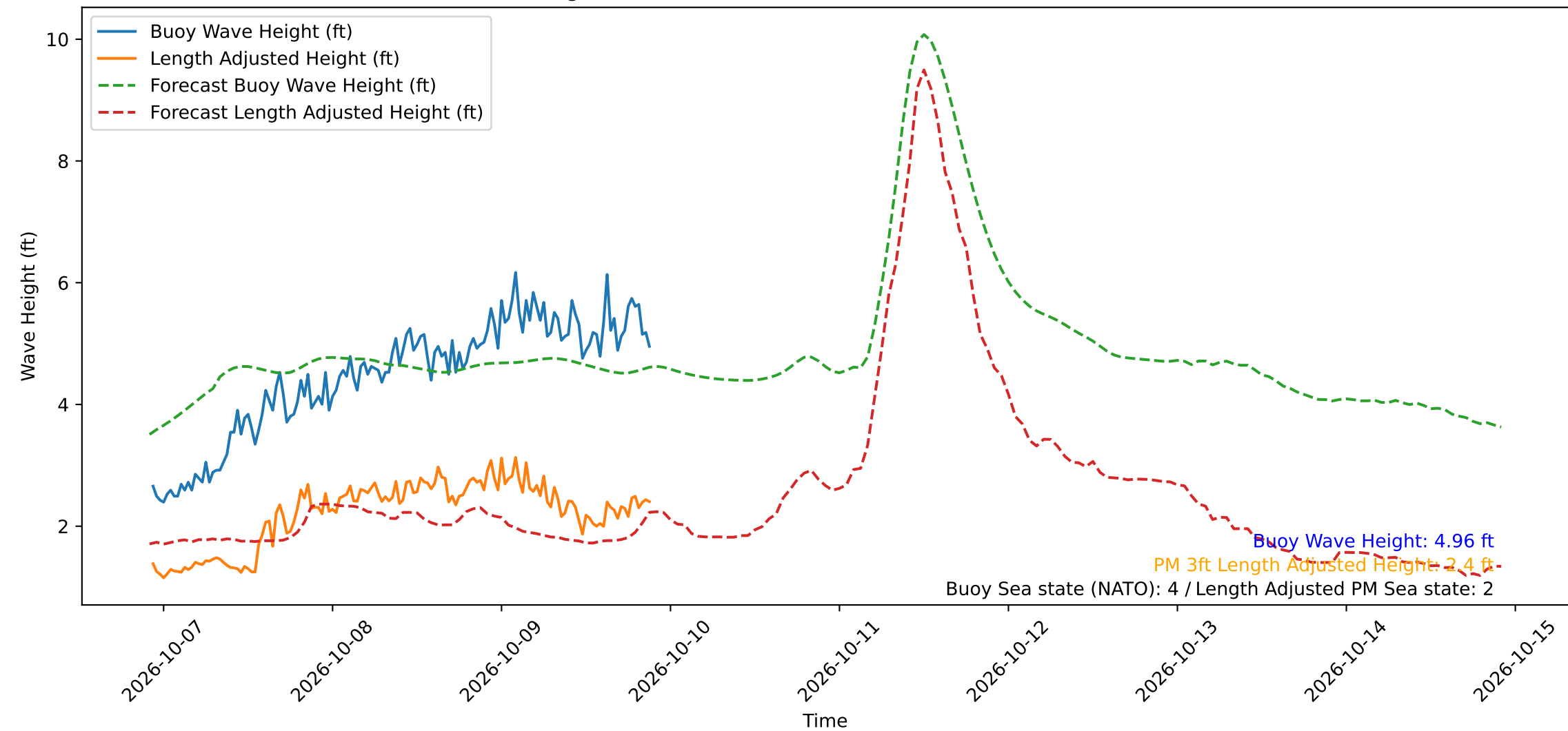
Wave Heights over Time for Green Beach at 2026-10-09 22:01:11
