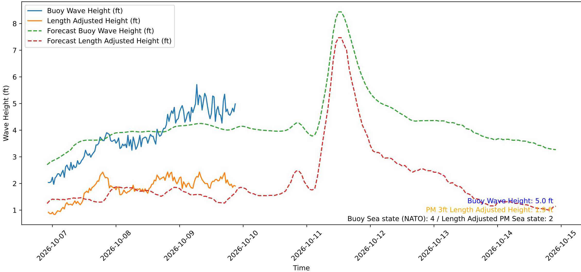
Wave Heights over Time for Red Beach at 2026-10-09 22:00:49
