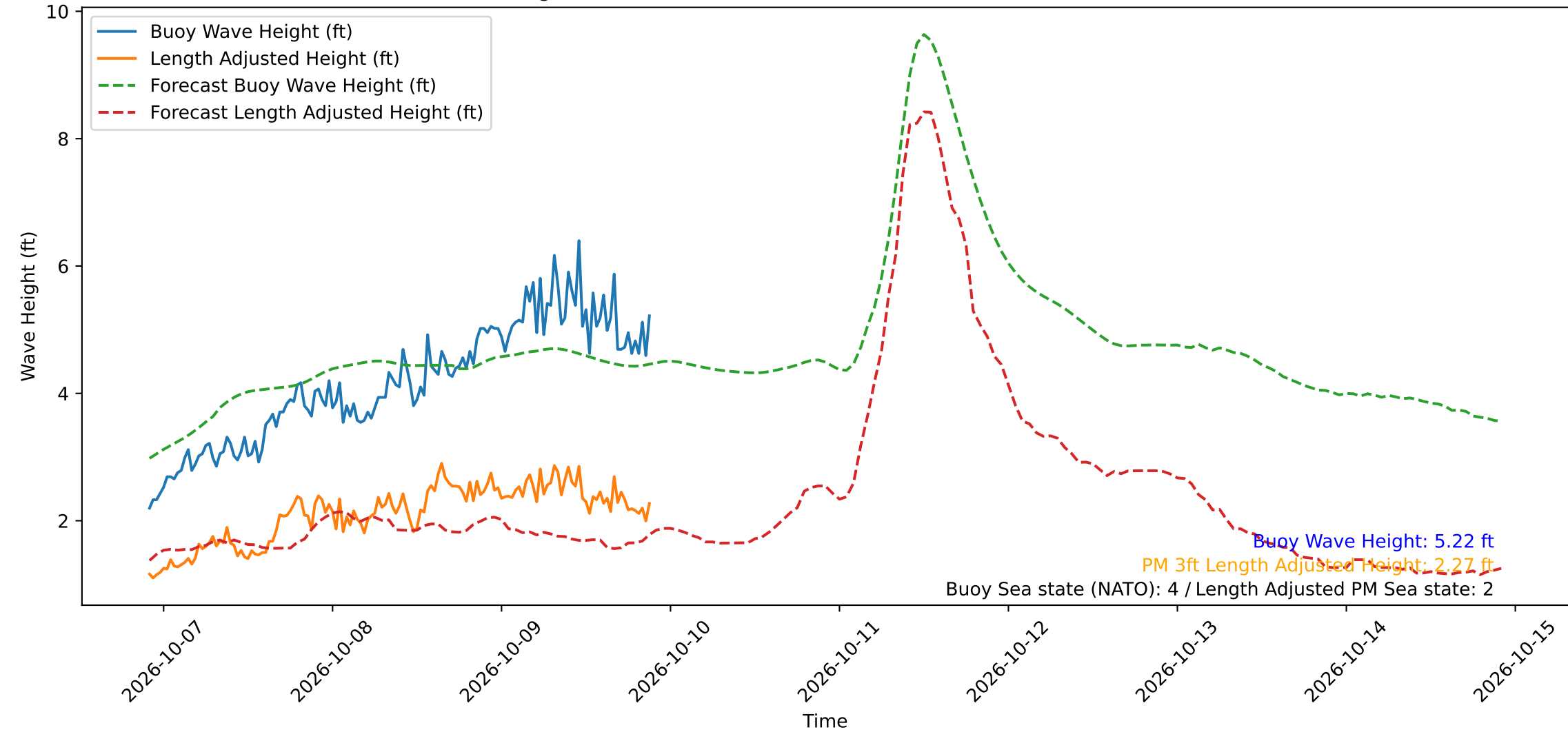
Wave Heights over Time for Oceanside Harbor at 2026-10-09 22:00:29
