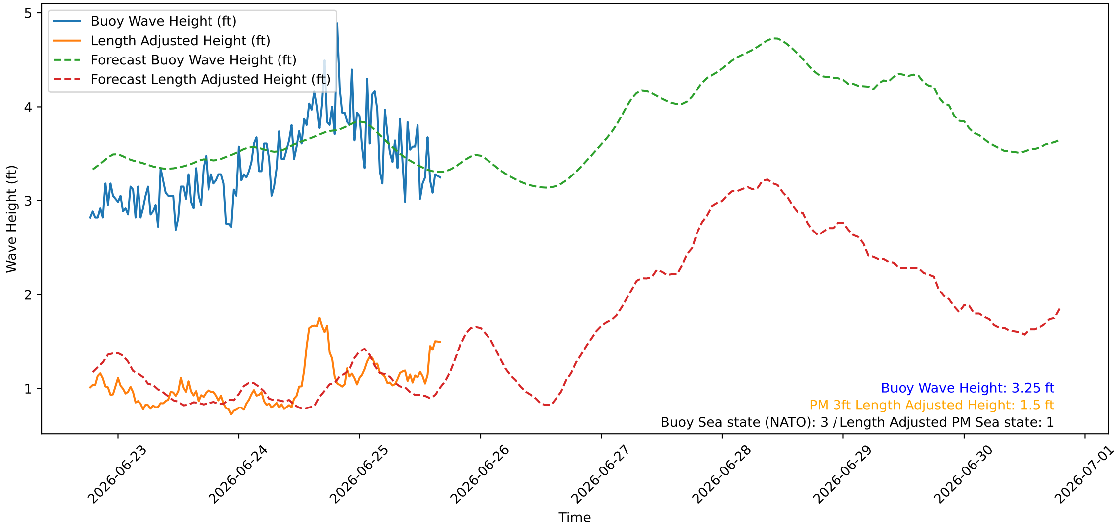
Wave Heights over Time for Oceanside Harbor at 2026-06-25 18:30:26
