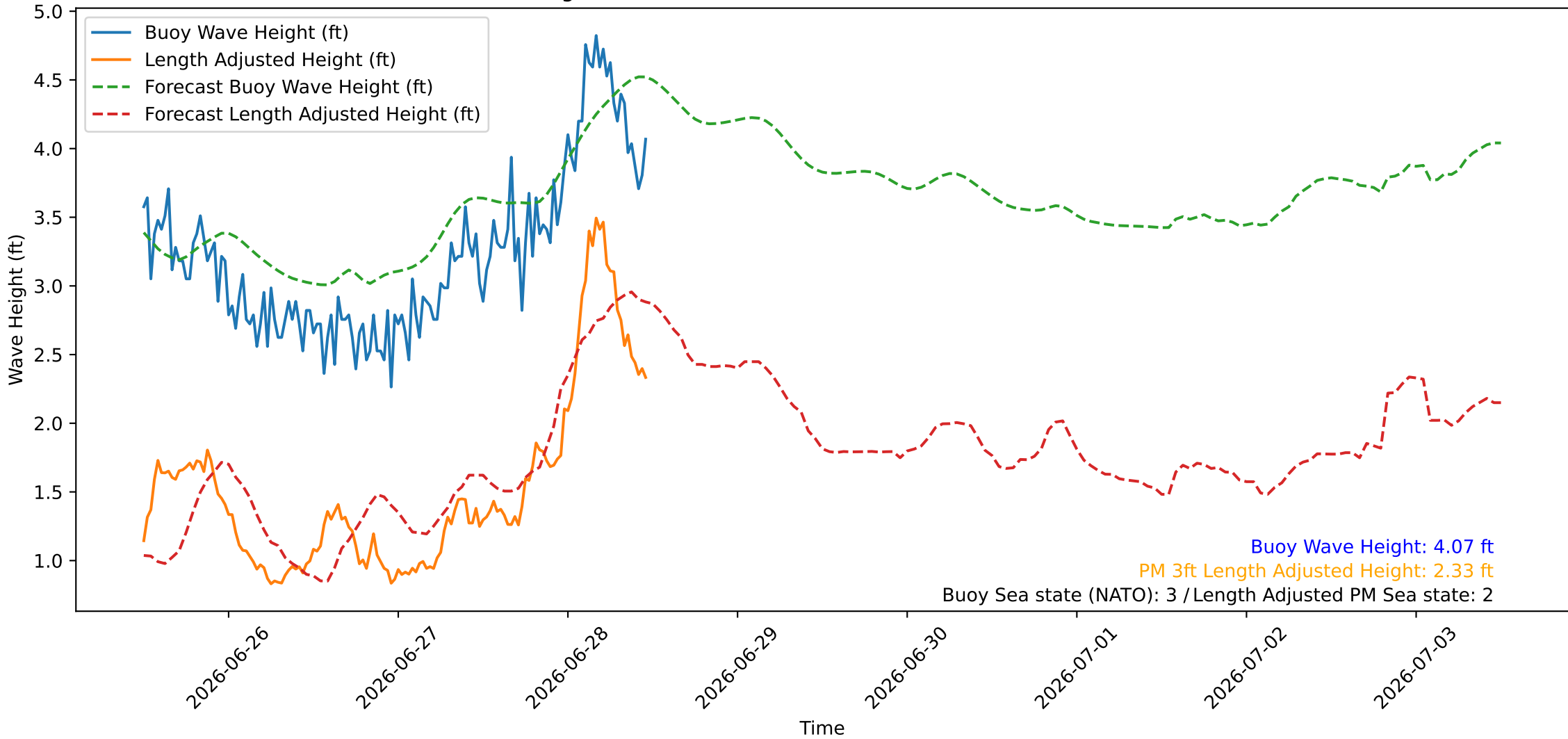
Wave Heights over Time for Green Beach at 2026-06-28 11:51:09
