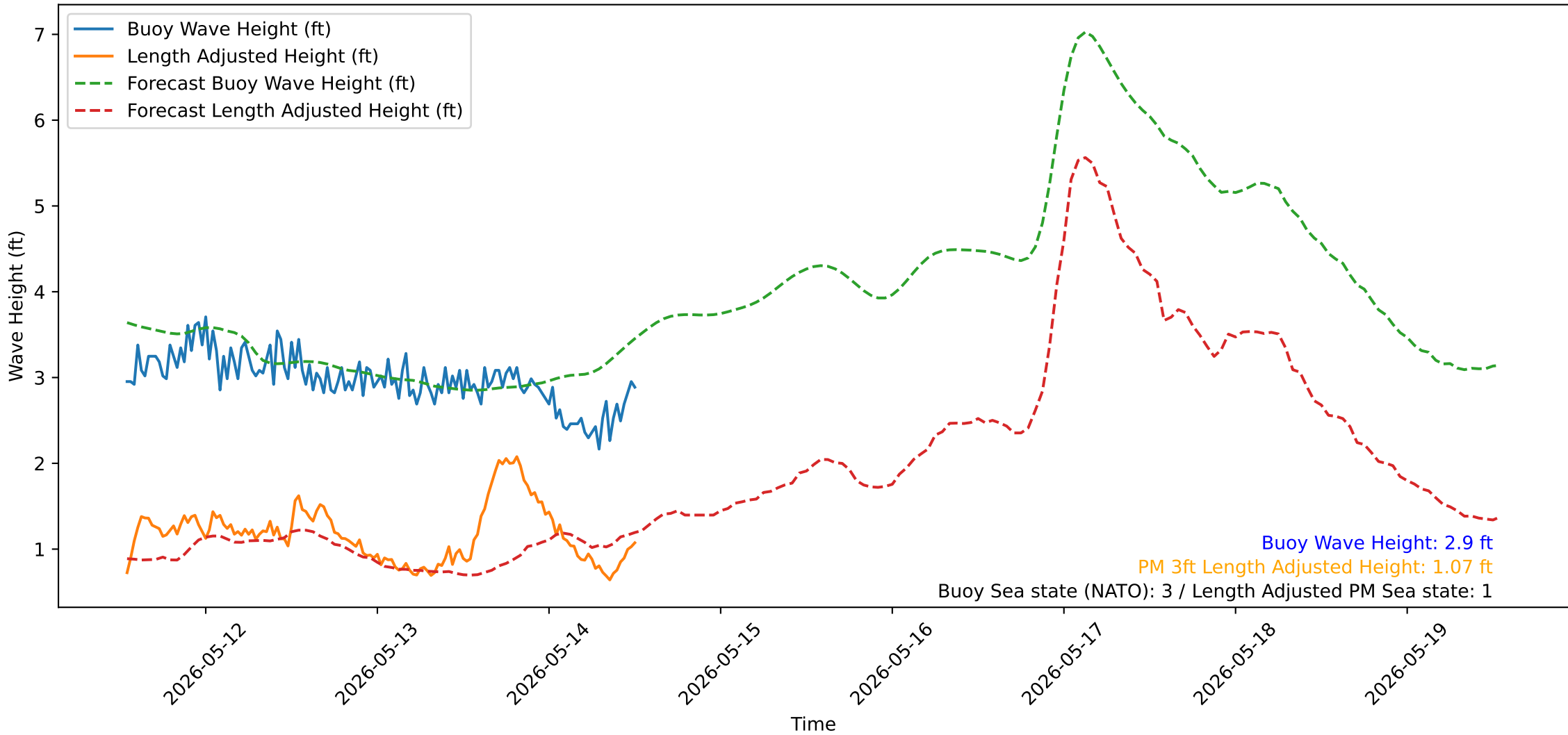
Wave Heights over Time for Oceanside Harbor at 2026-05-14 12:50:32
