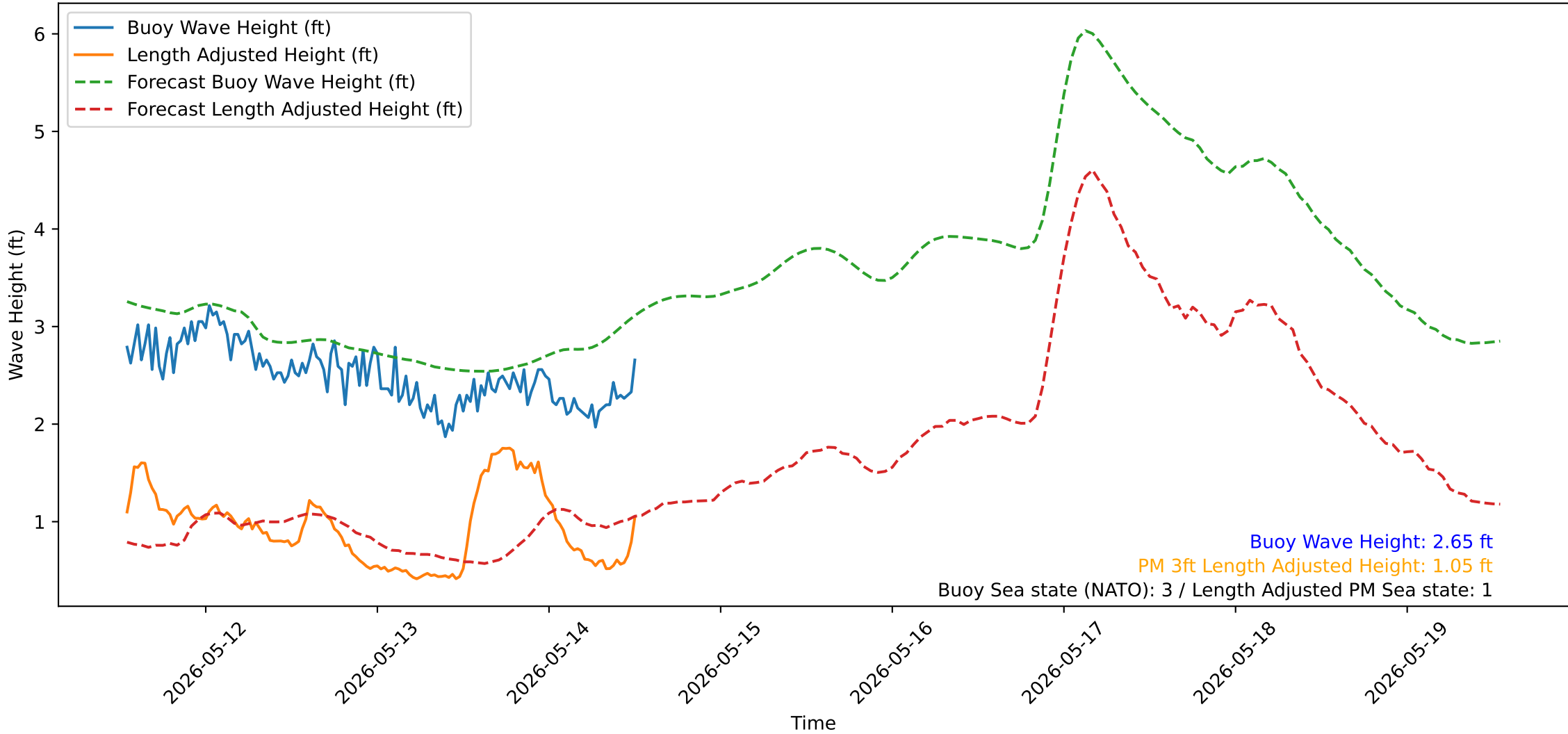
Wave Heights over Time for Red Beach at 2026-05-14 12:50:53
