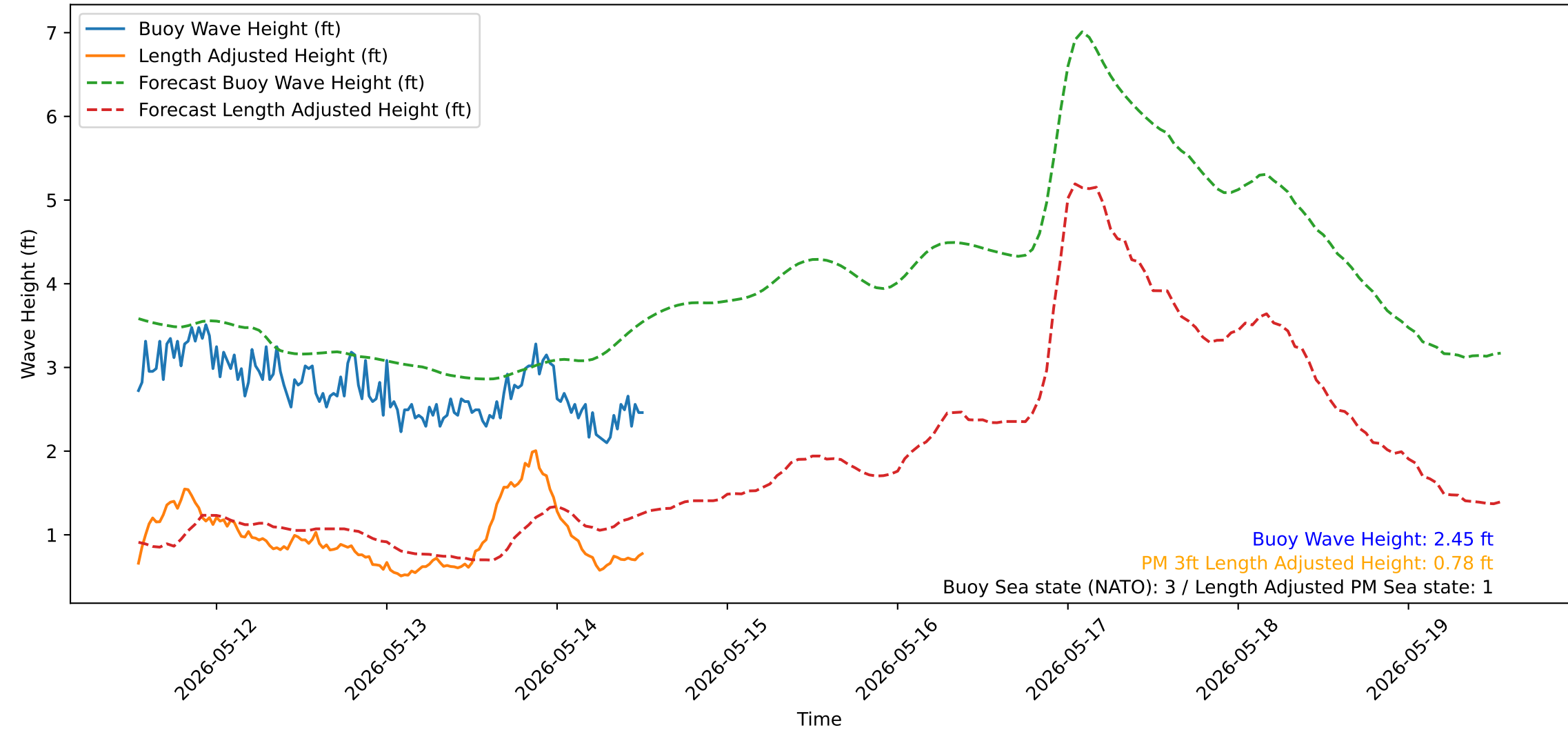
Wave Heights over Time for Green Beach at 2026-05-14 12:51:16
