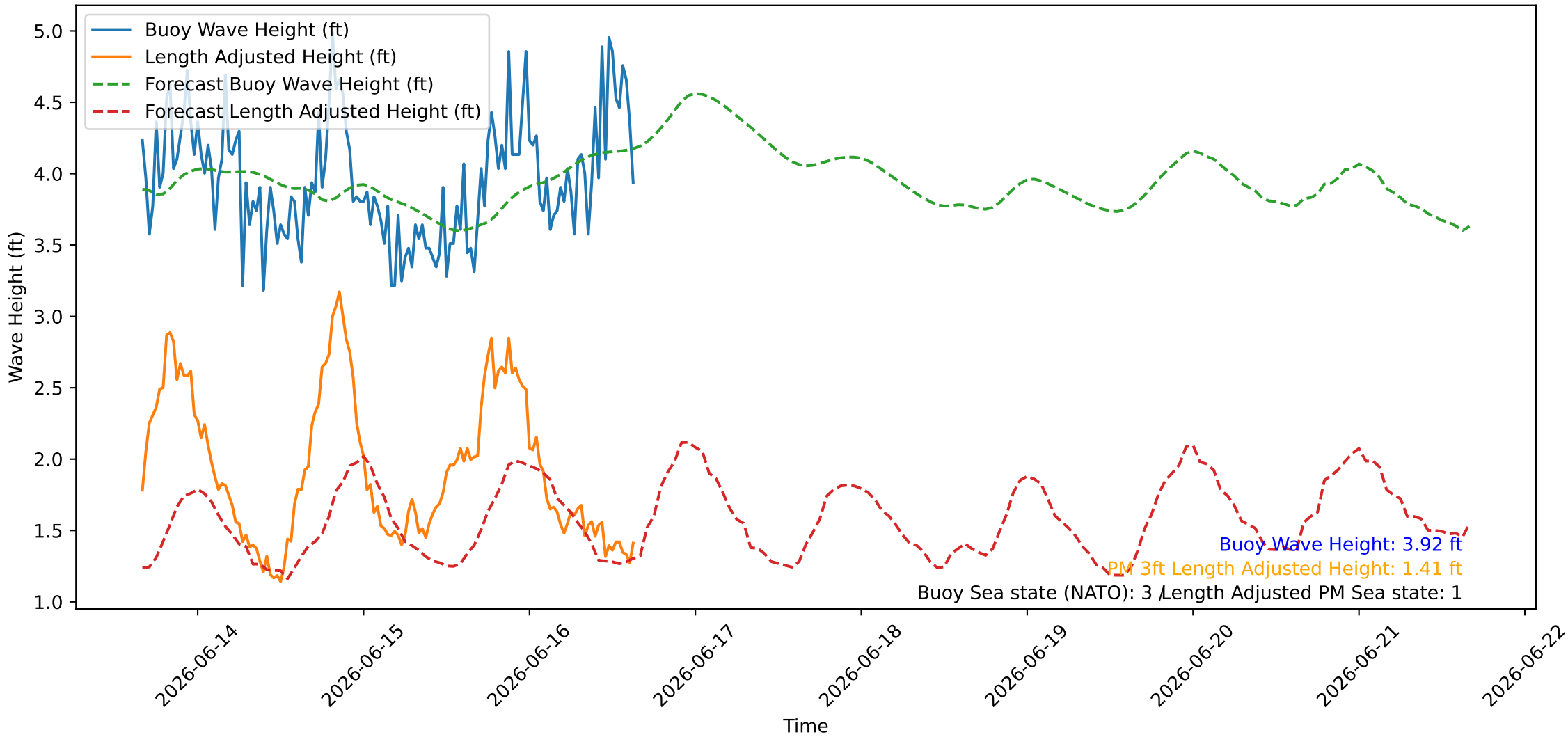
Wave Heights over Time for Oceanside Harbor at 2026-06-16 16:00:26
