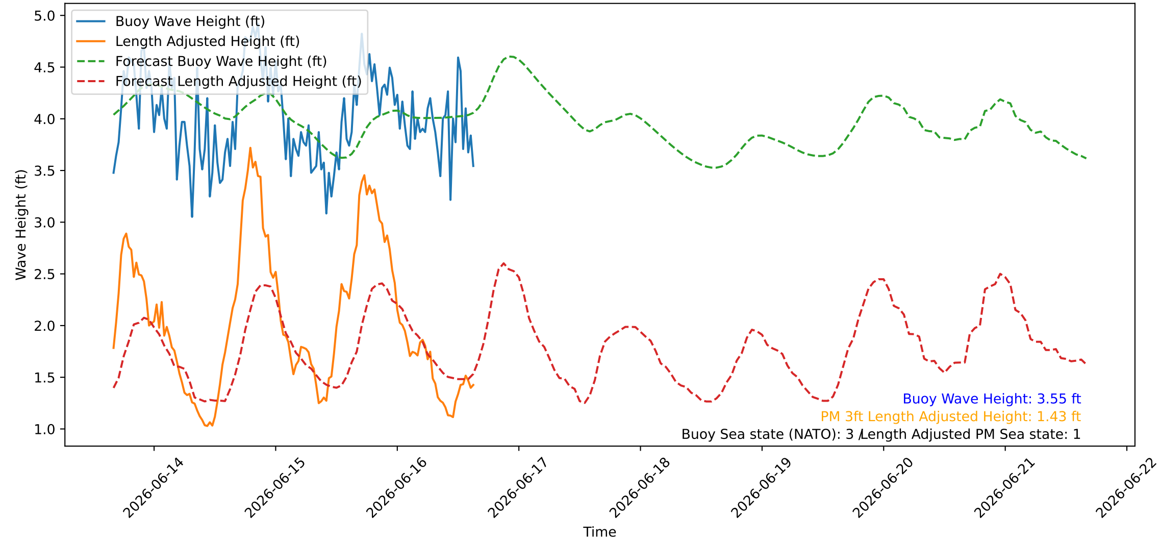
Wave Heights over Time for Green Beach at 2026-06-16 16:01:07
