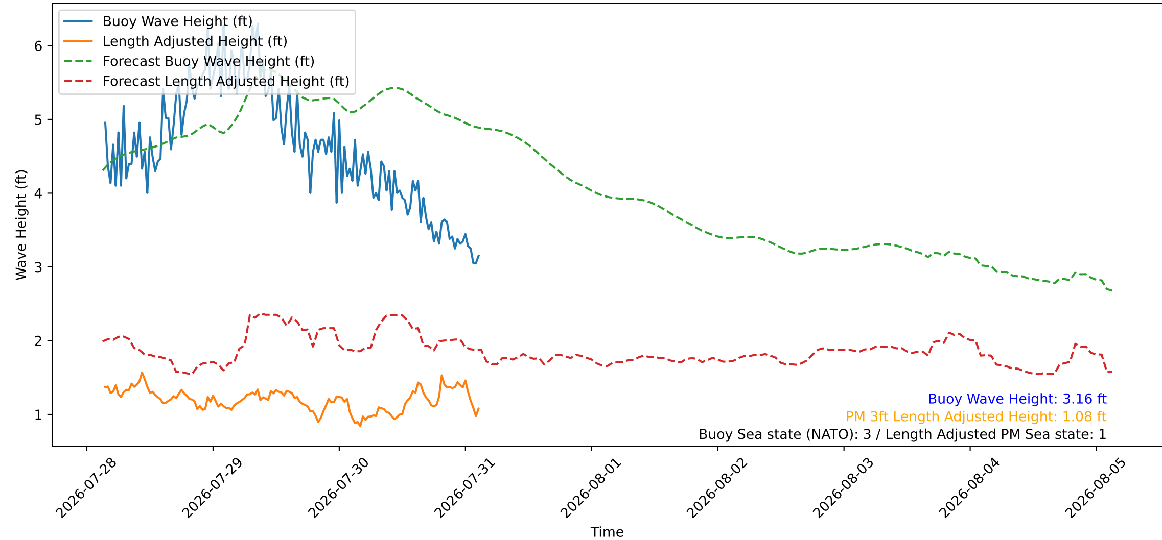
Wave Heights over Time for Green Beach at 2026-07-31 03:21:10
