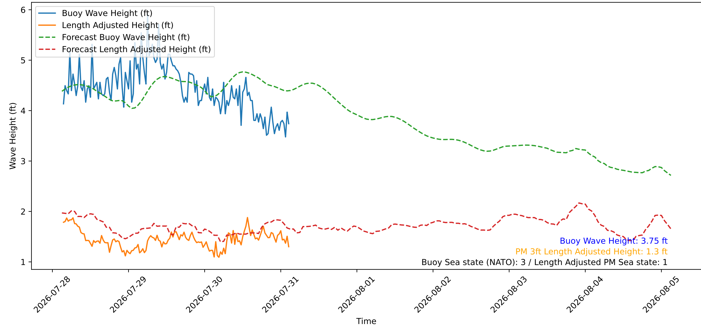
Wave Heights over Time for Oceanside Harbor at 2026-07-31 03:20:26
