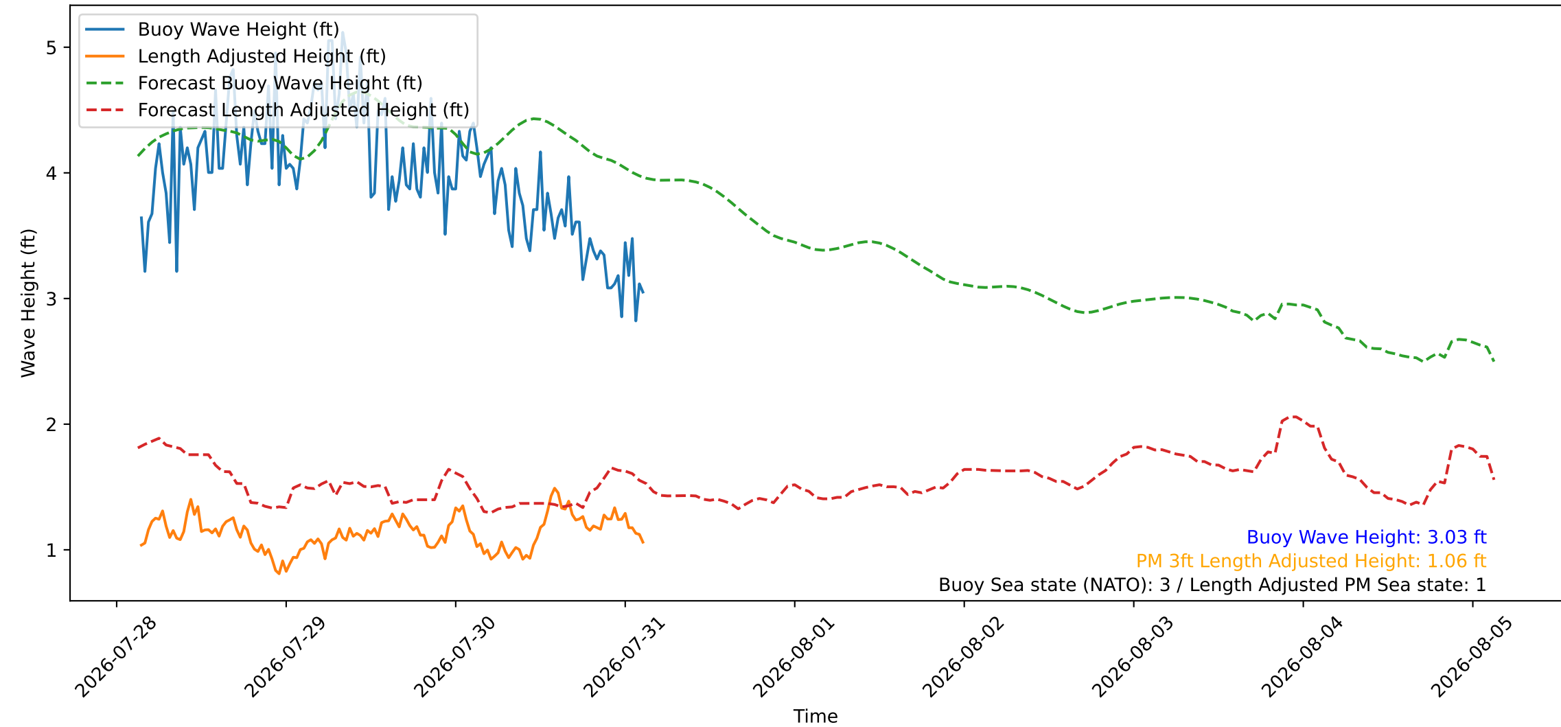
Wave Heights over Time for Red Beach at 2026-07-31 03:20:47
