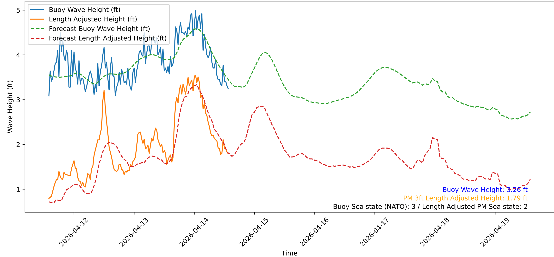
Wave Heights over Time for Green Beach at 2026-04-14 14:11:12
