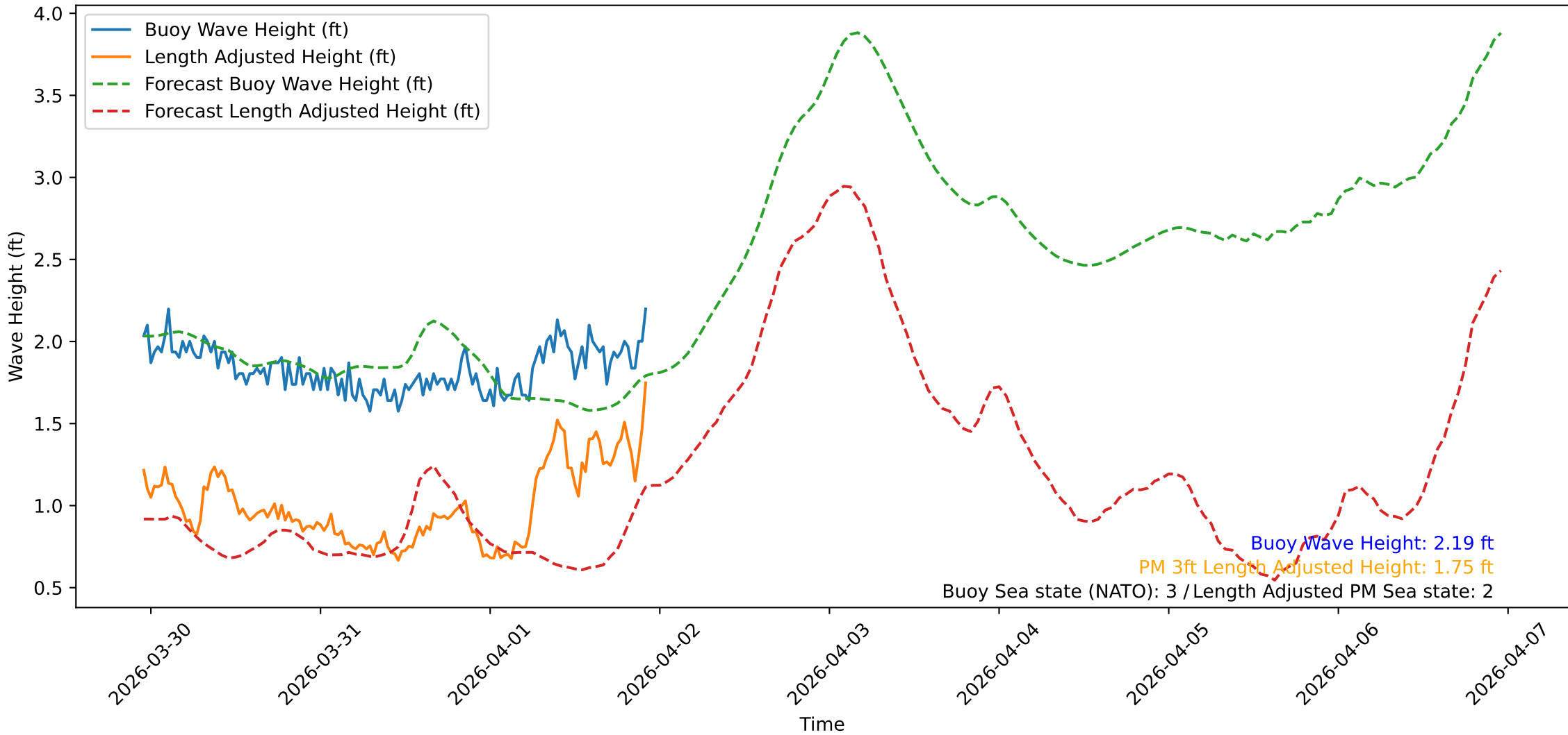
Wave Heights over Time for Oceanside Harbor at 2026-04-01 22:50:31
