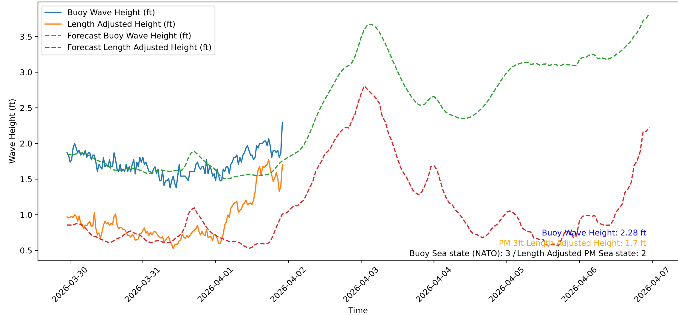
Wave Heights over Time for Red Beach at 2026-04-01 22:50:47
