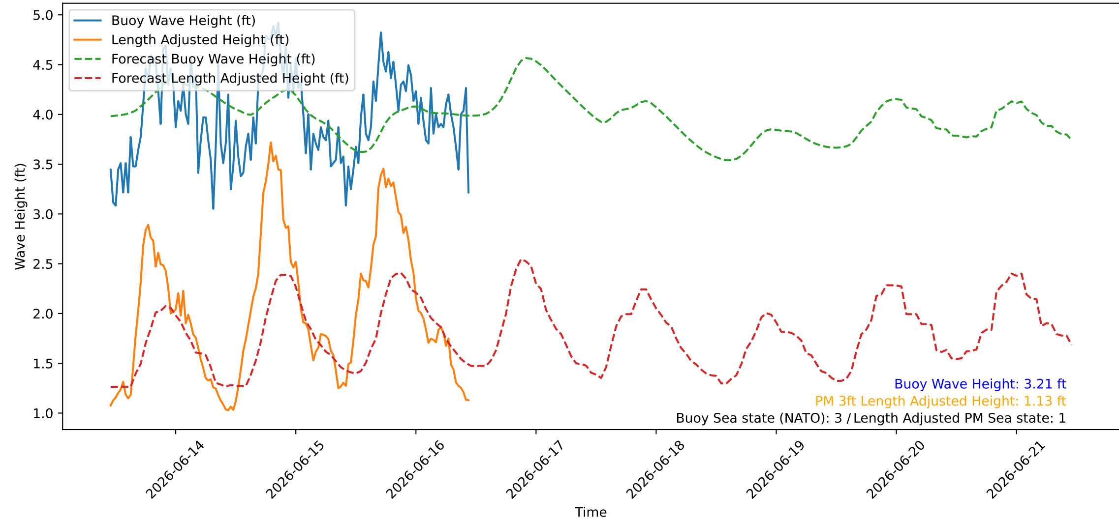
Wave Heights over Time for Green Beach at 2026-06-16 11:11:08
