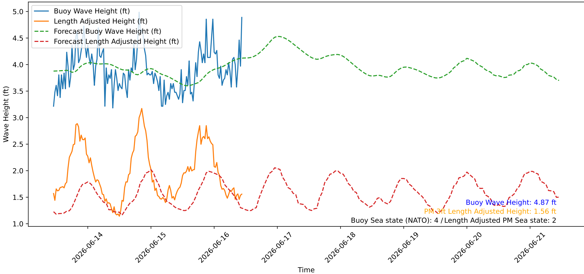
Wave Heights over Time for Oceanside Harbor at 2026-06-16 11:10:25
