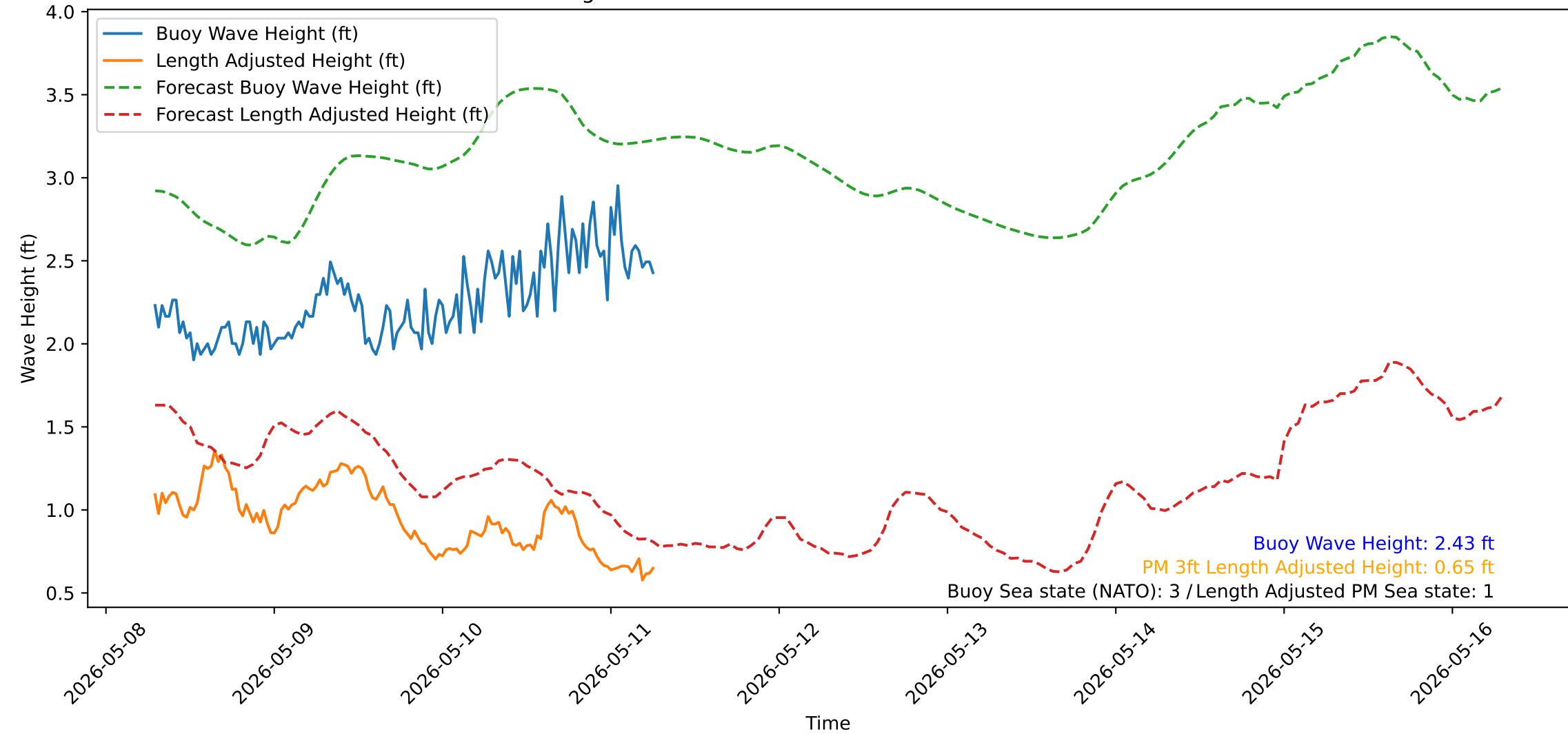
Wave Heights over Time for Red Beach at 2026-05-11 06:50:51
