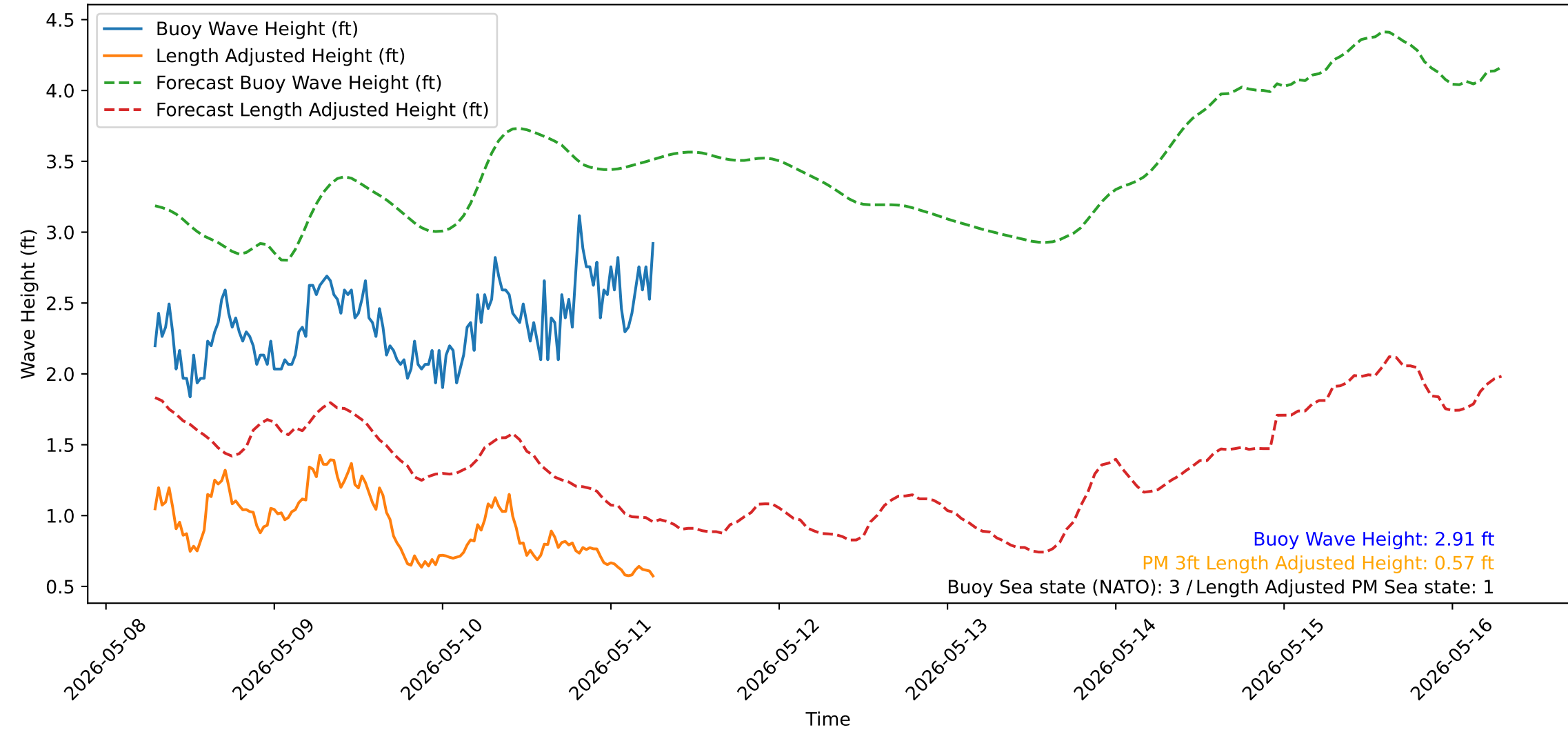
Wave Heights over Time for Green Beach at 2026-05-11 06:51:14
