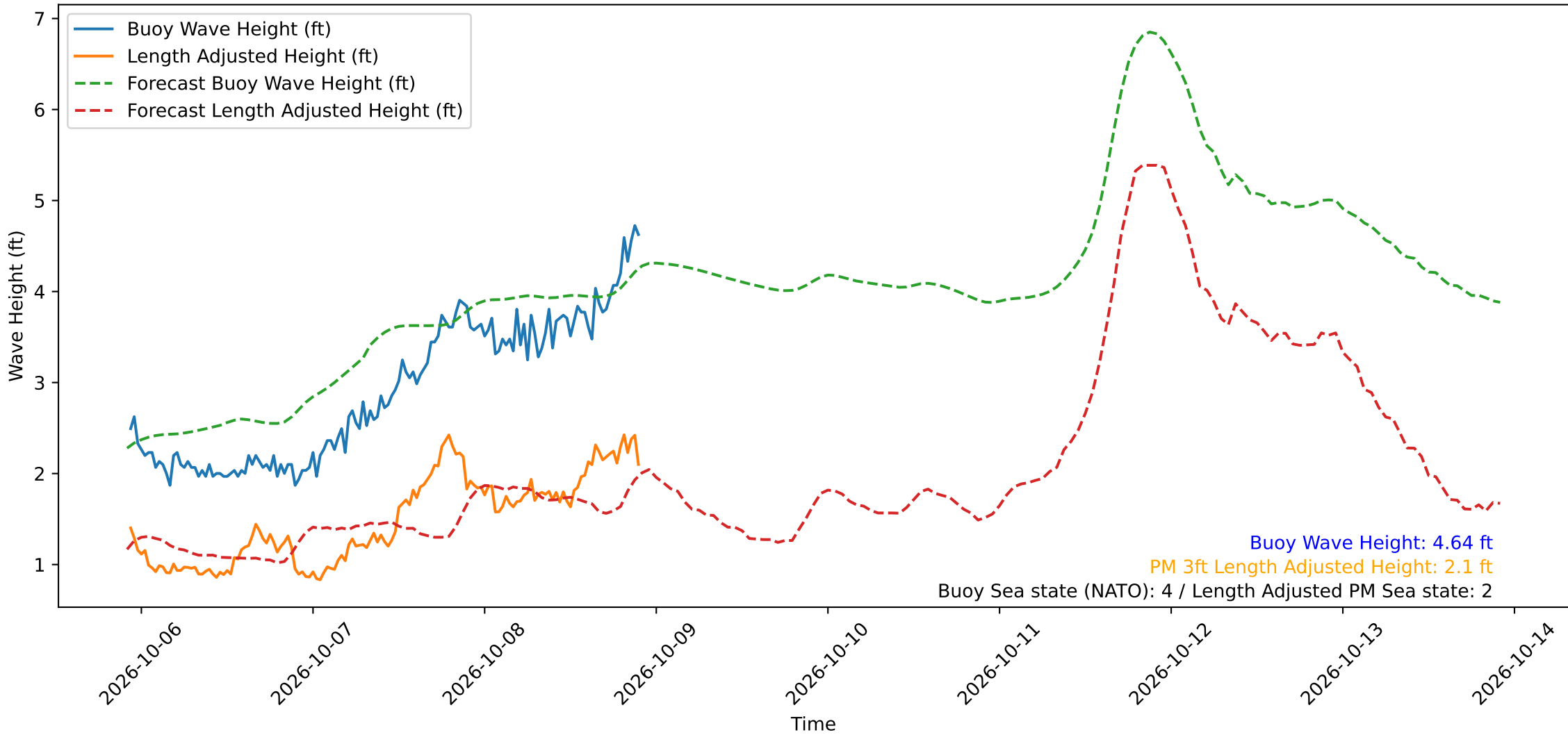
Wave Heights over Time for Red Beach at 2026-10-08 22:10:49
