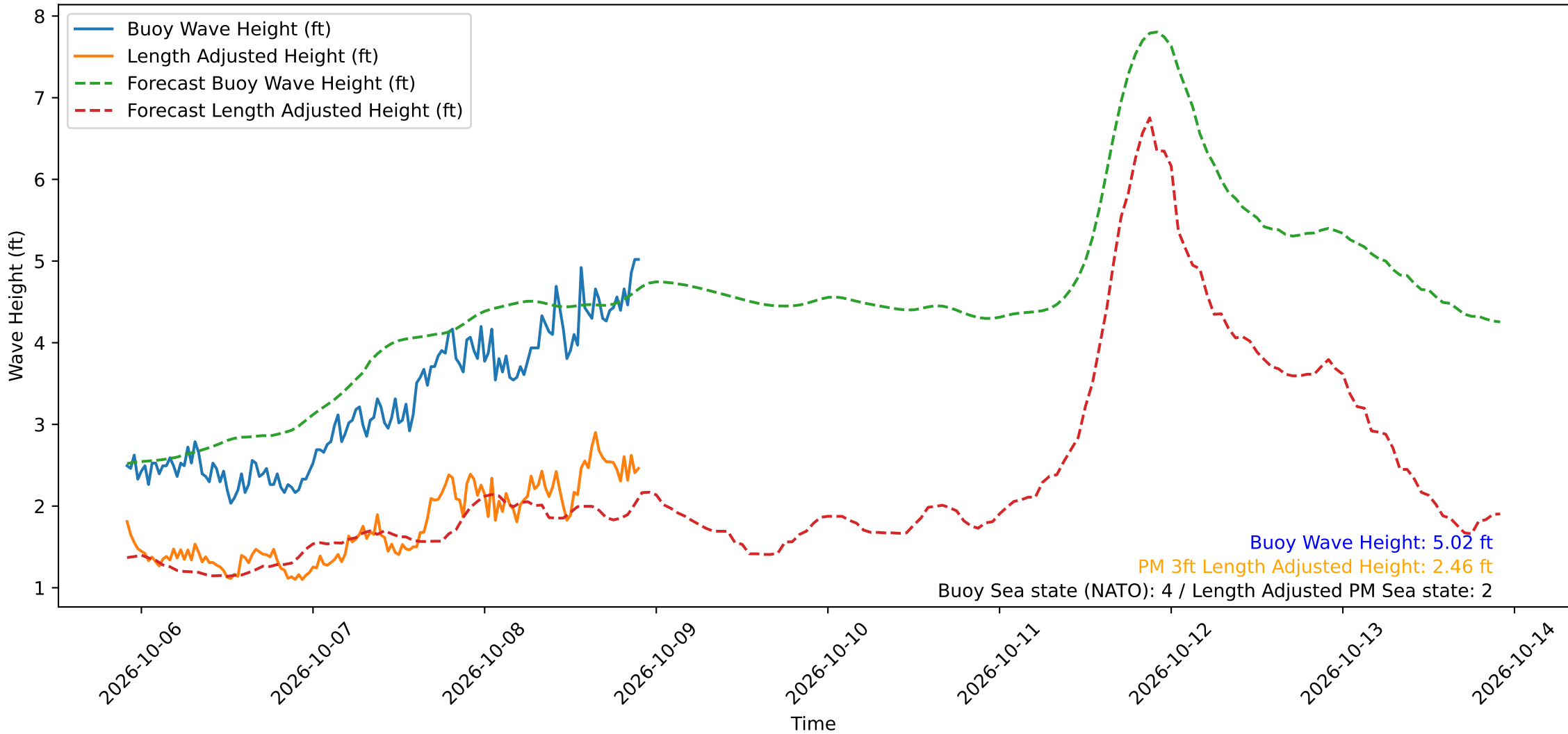
Wave Heights over Time for Oceanside Harbor at 2026-10-08 22:10:29
