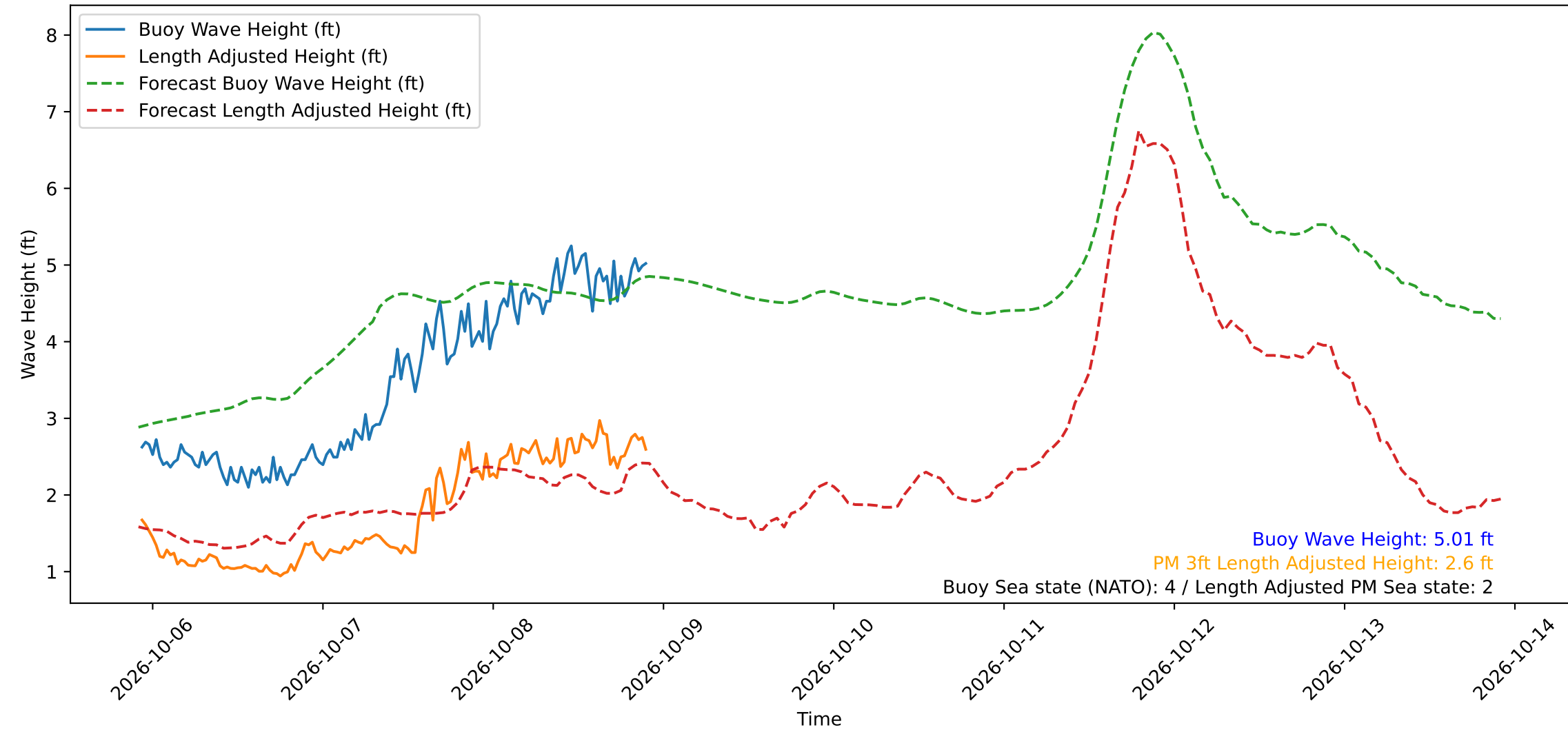
Wave Heights over Time for Green Beach at 2026-10-08 22:11:12
