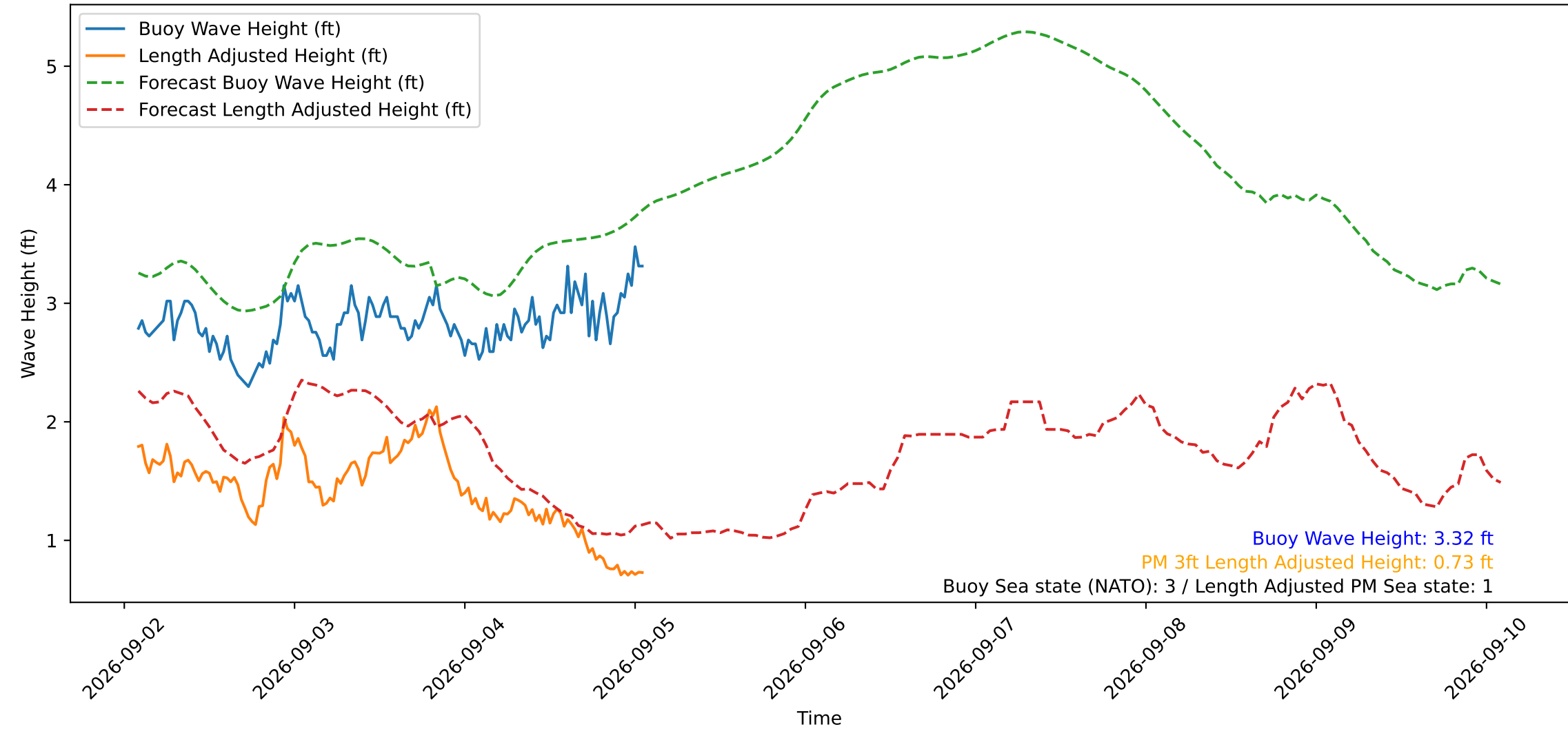
Wave Heights over Time for Red Beach at 2026-09-05 01:40:49
