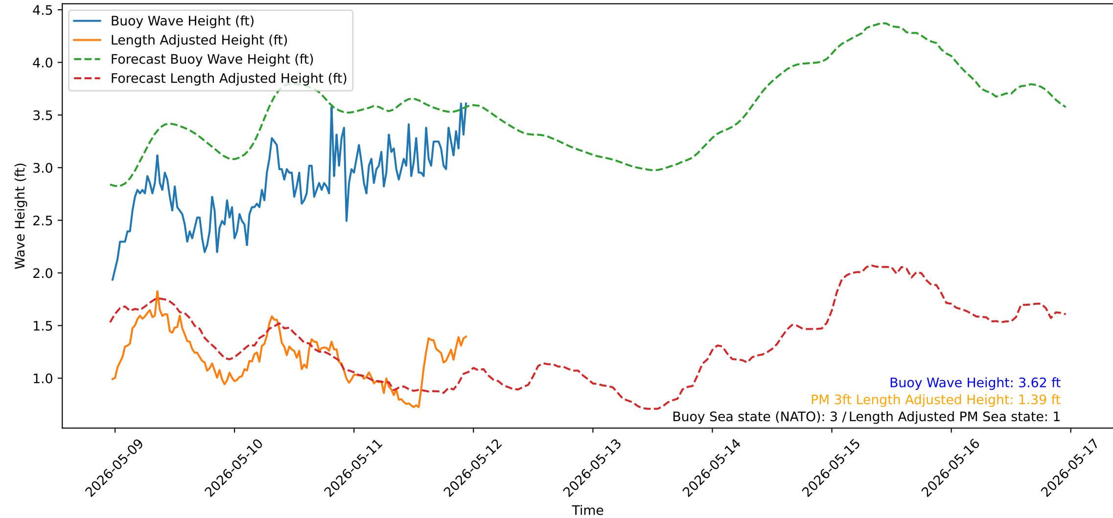
Wave Heights over Time for Oceanside Harbor at 2026-05-11 23:20:32
