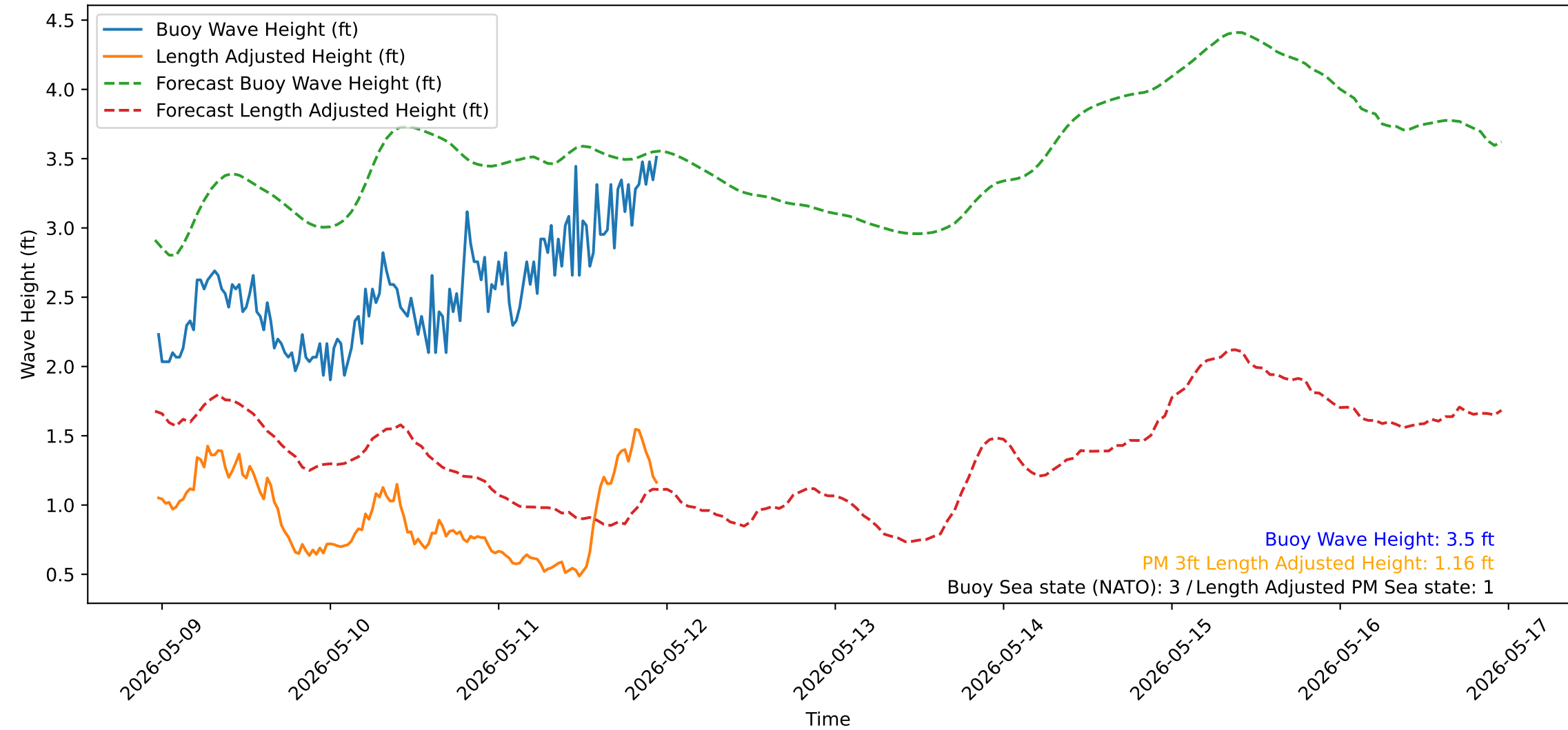
Wave Heights over Time for Green Beach at 2026-05-11 23:21:14
