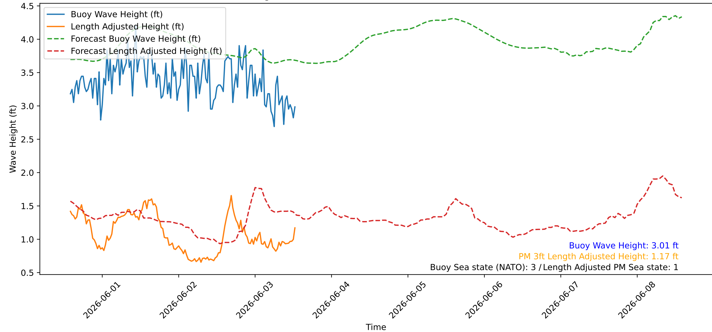
Wave Heights over Time for Red Beach at 2026-06-03 13:30:45
