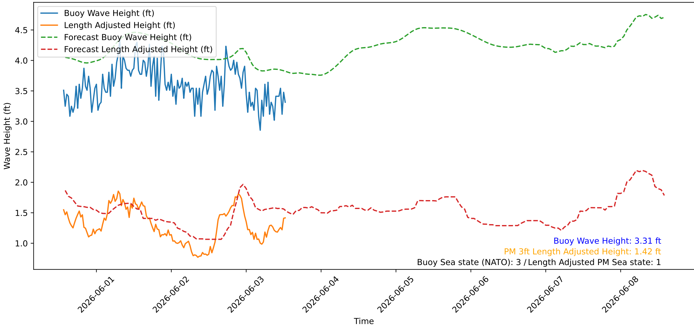
Wave Heights over Time for Green Beach at 2026-06-03 13:31:07
