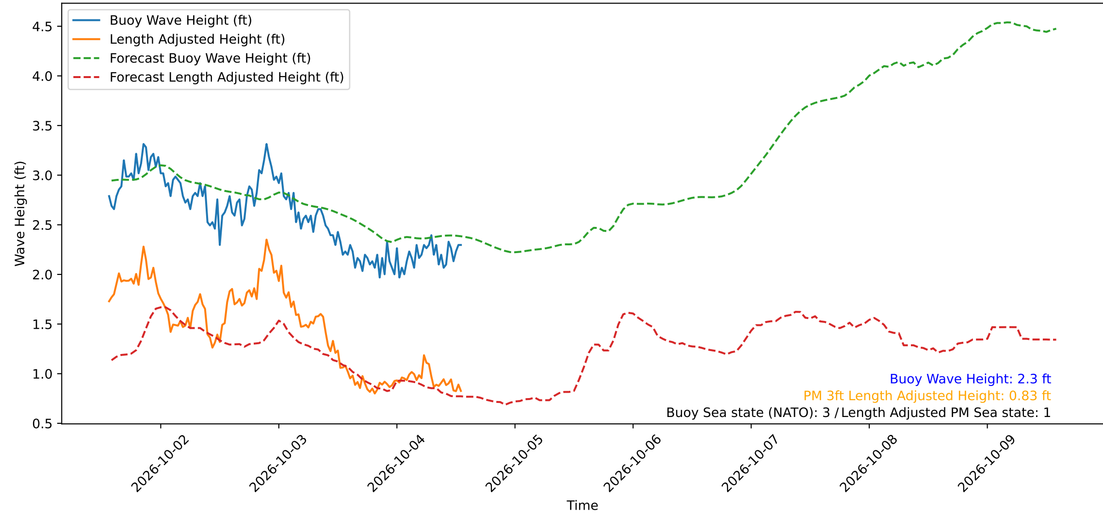
Wave Heights over Time for Oceanside Harbor at 2026-10-04 13:40:30
