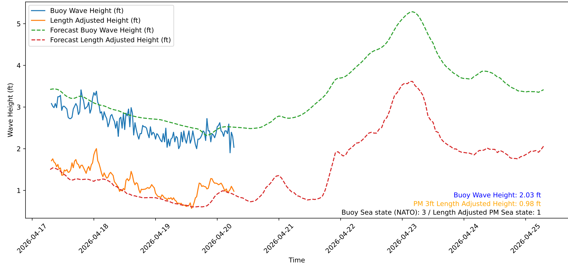
Wave Heights over Time for Oceanside Harbor at 2026-04-20 07:20:32
