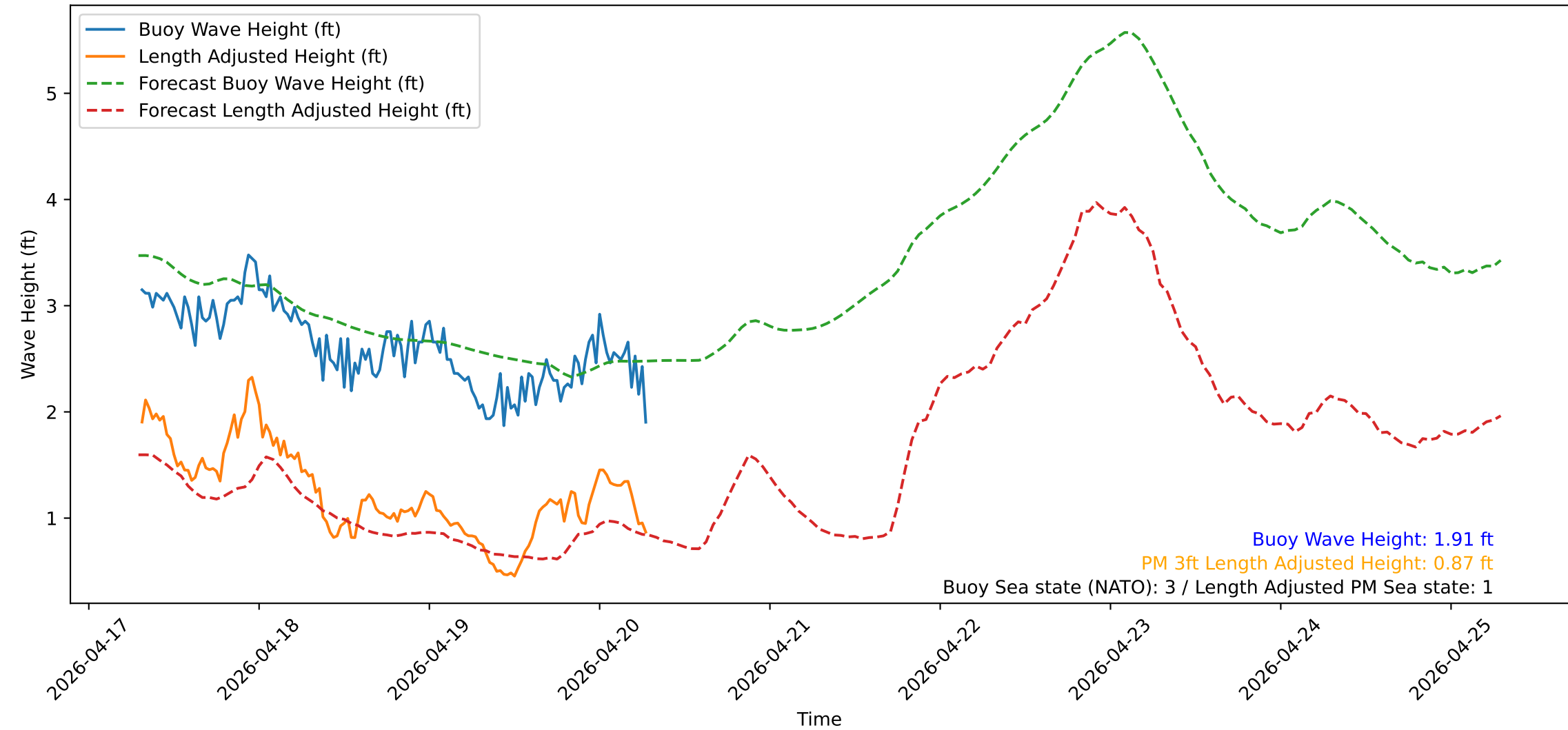
Wave Heights over Time for Green Beach at 2026-04-20 07:21:15
