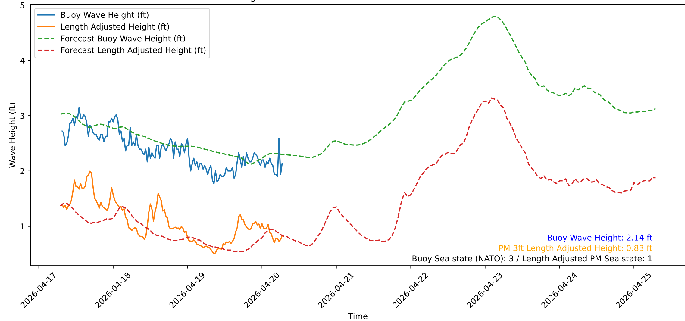
Wave Heights over Time for Red Beach at 2026-04-20 07:20:52
