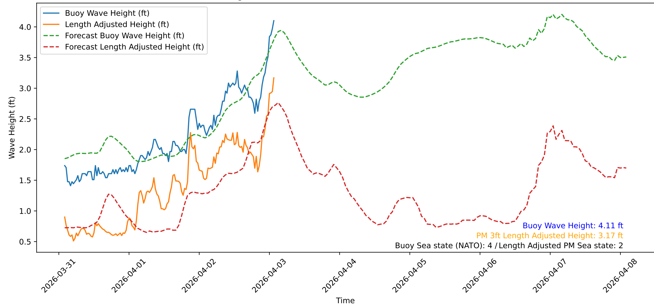
Wave Heights over Time for Green Beach at 2026-04-03 02:11:09
