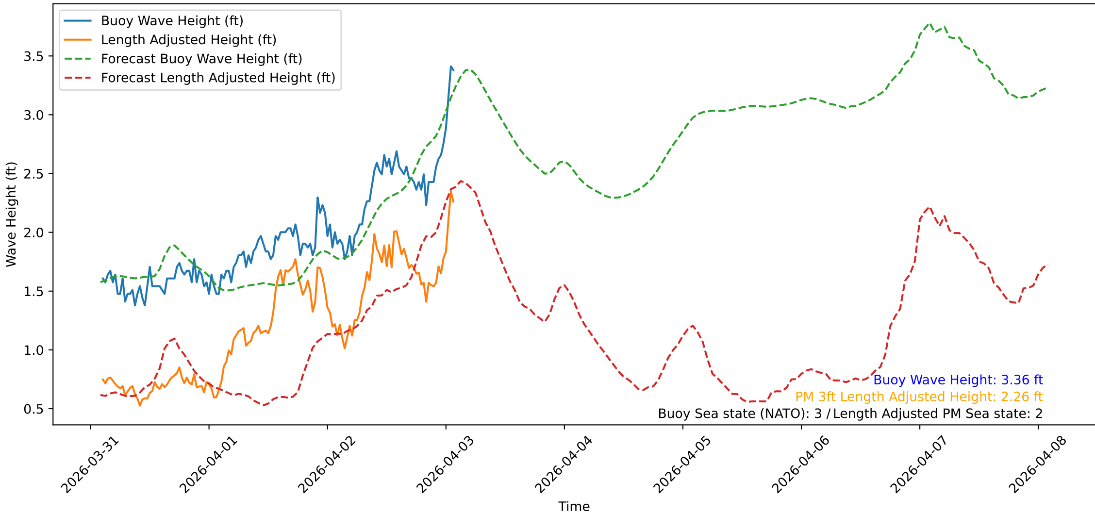
Wave Heights over Time for Red Beach at 2026-04-03 02:10:47
