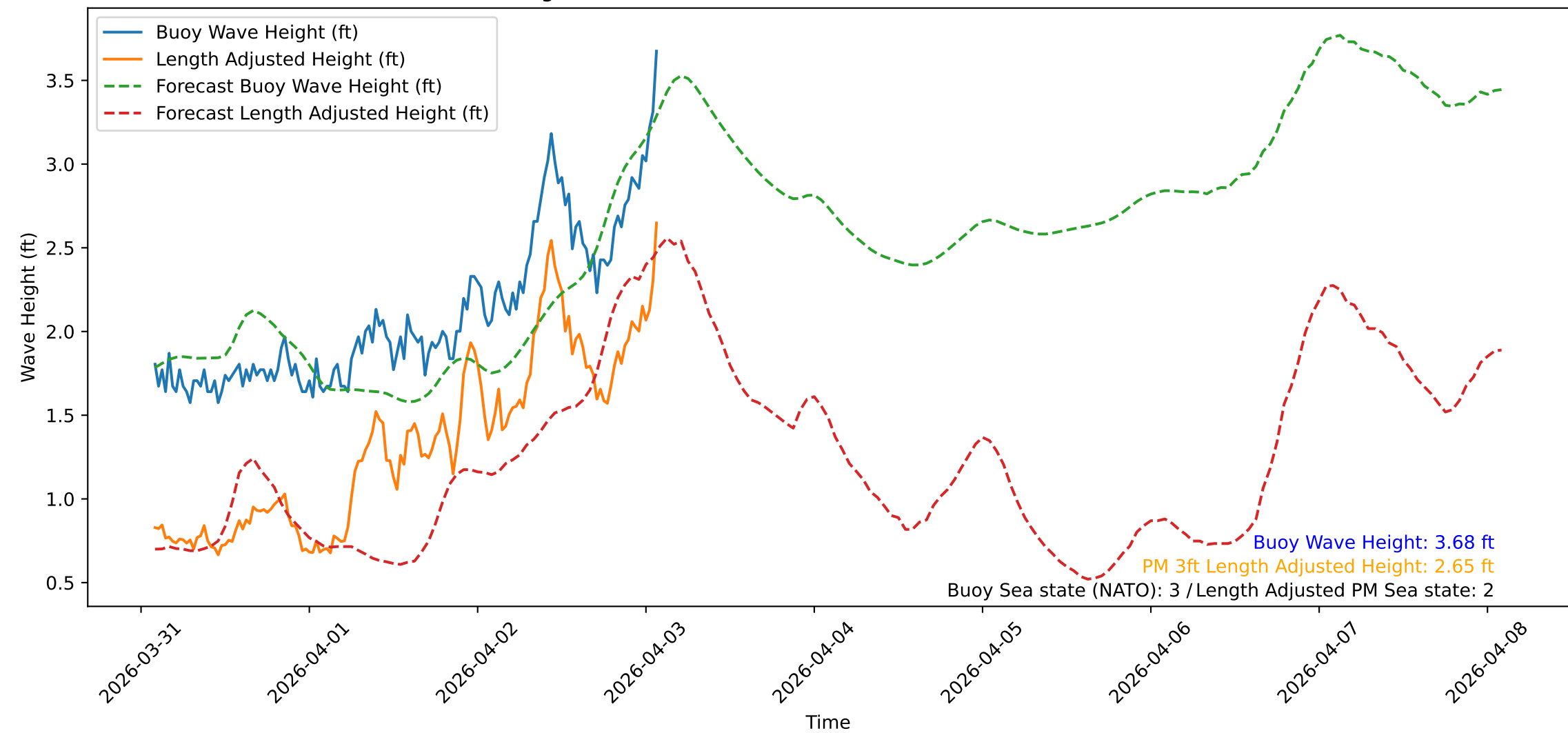
Wave Heights over Time for Oceanside Harbor at 2026-04-03 02:10:31
