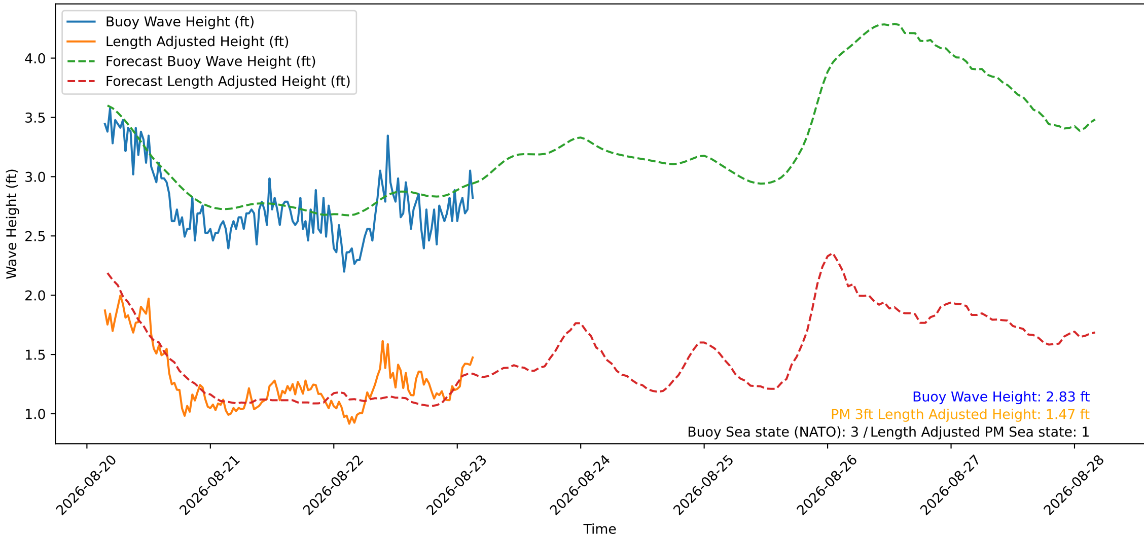
Wave Heights over Time for Oceanside Harbor at 2026-08-23 03:40:29
