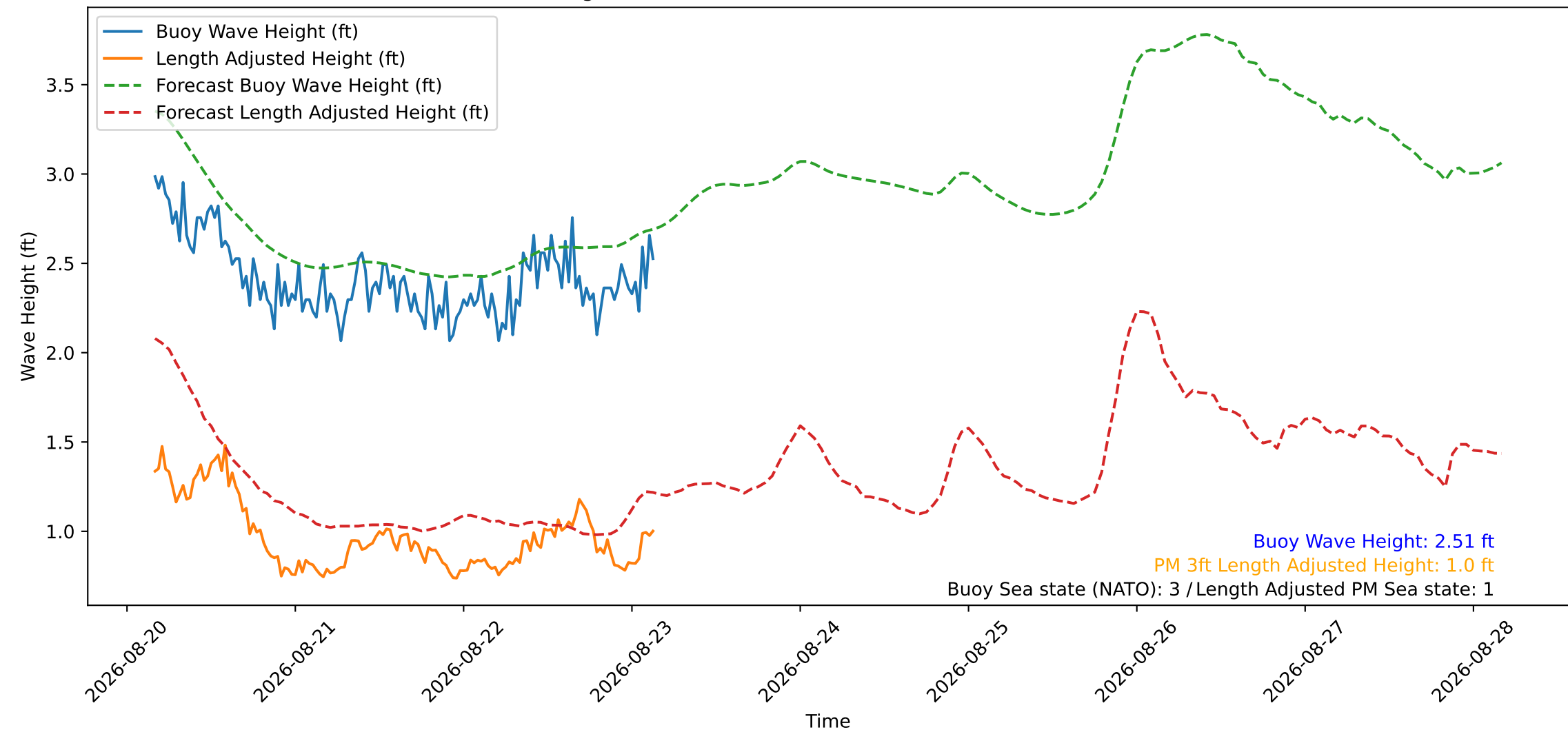
Wave Heights over Time for Red Beach at 2026-08-23 03:40:48
