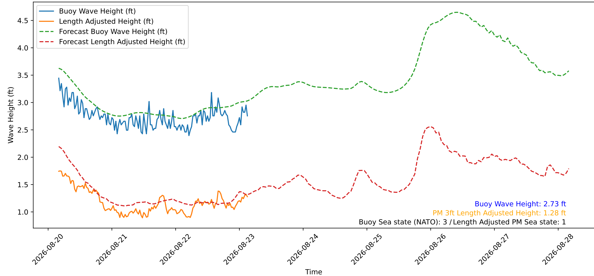
Wave Heights over Time for Green Beach at 2026-08-23 03:41:11
