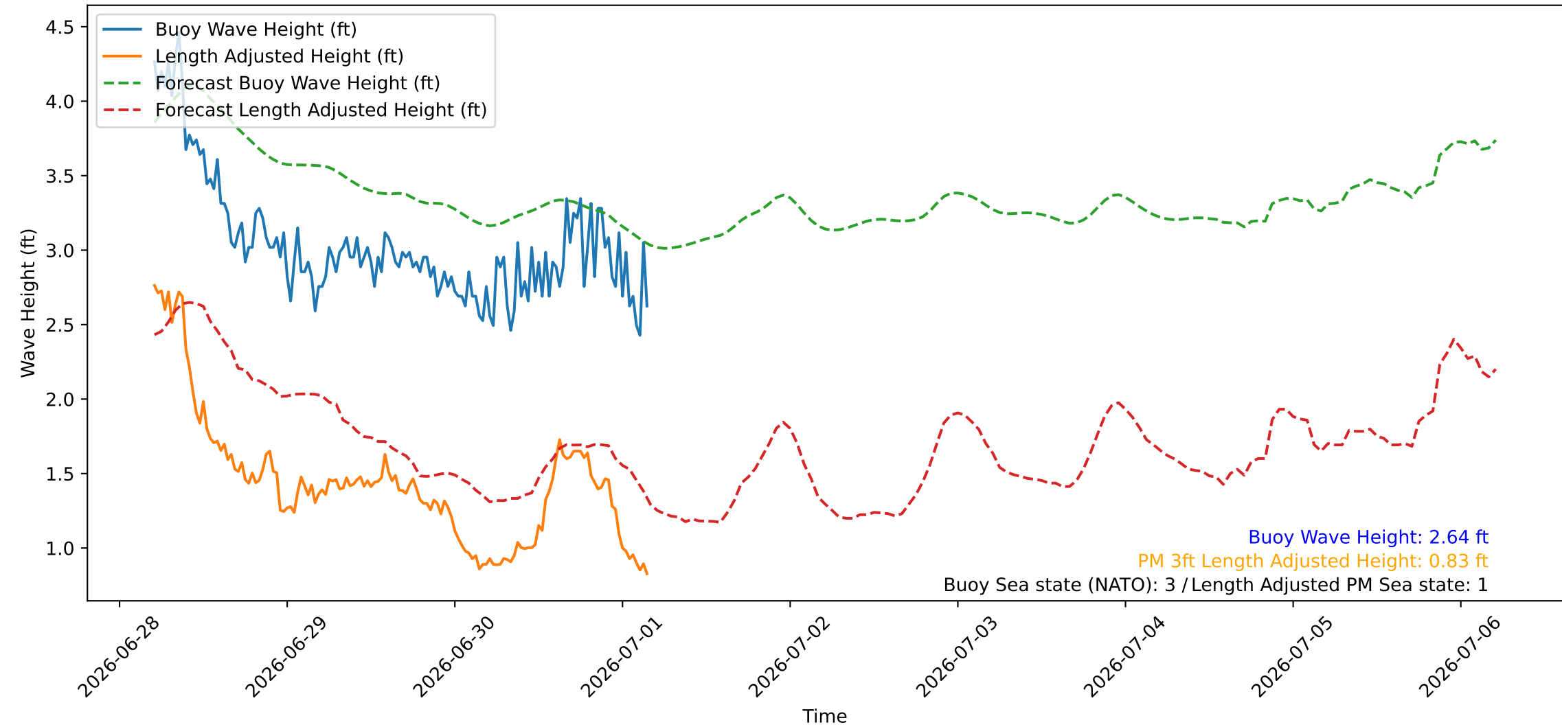
Wave Heights over Time for Red Beach at 2026-07-01 04:30:47
