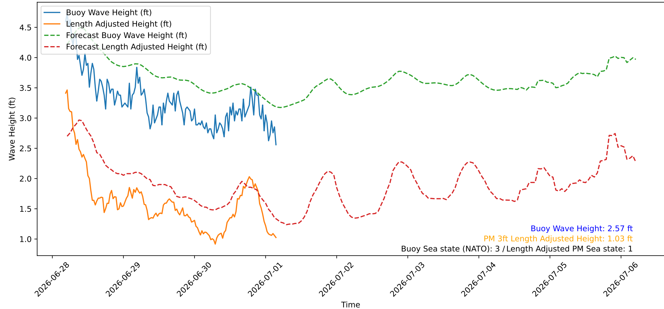
Wave Heights over Time for Green Beach at 2026-07-01 04:31:10
