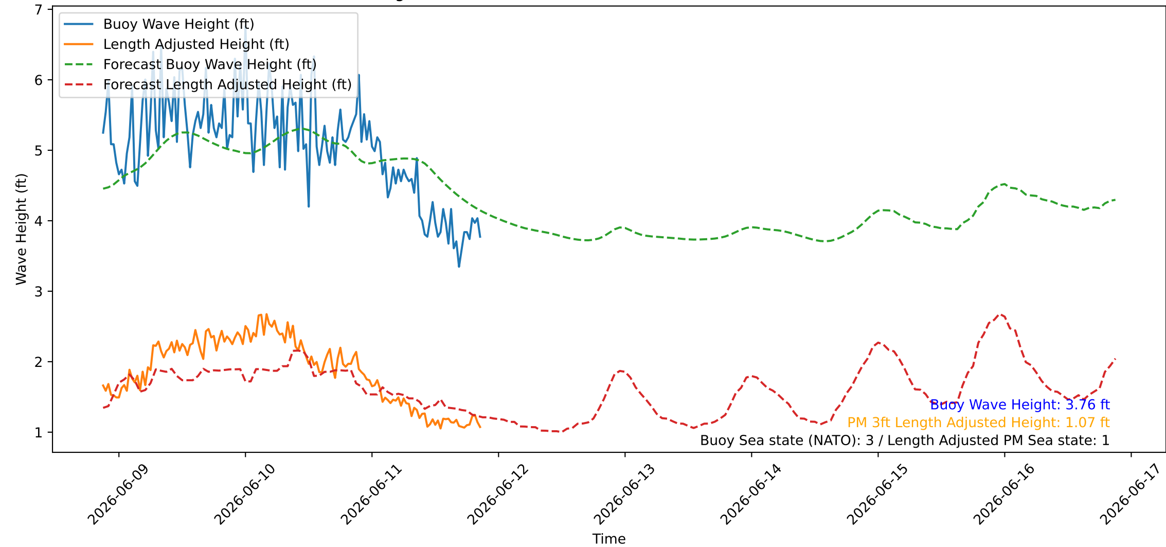
Wave Heights over Time for Oceanside Harbor at 2026-06-11 21:00:27
