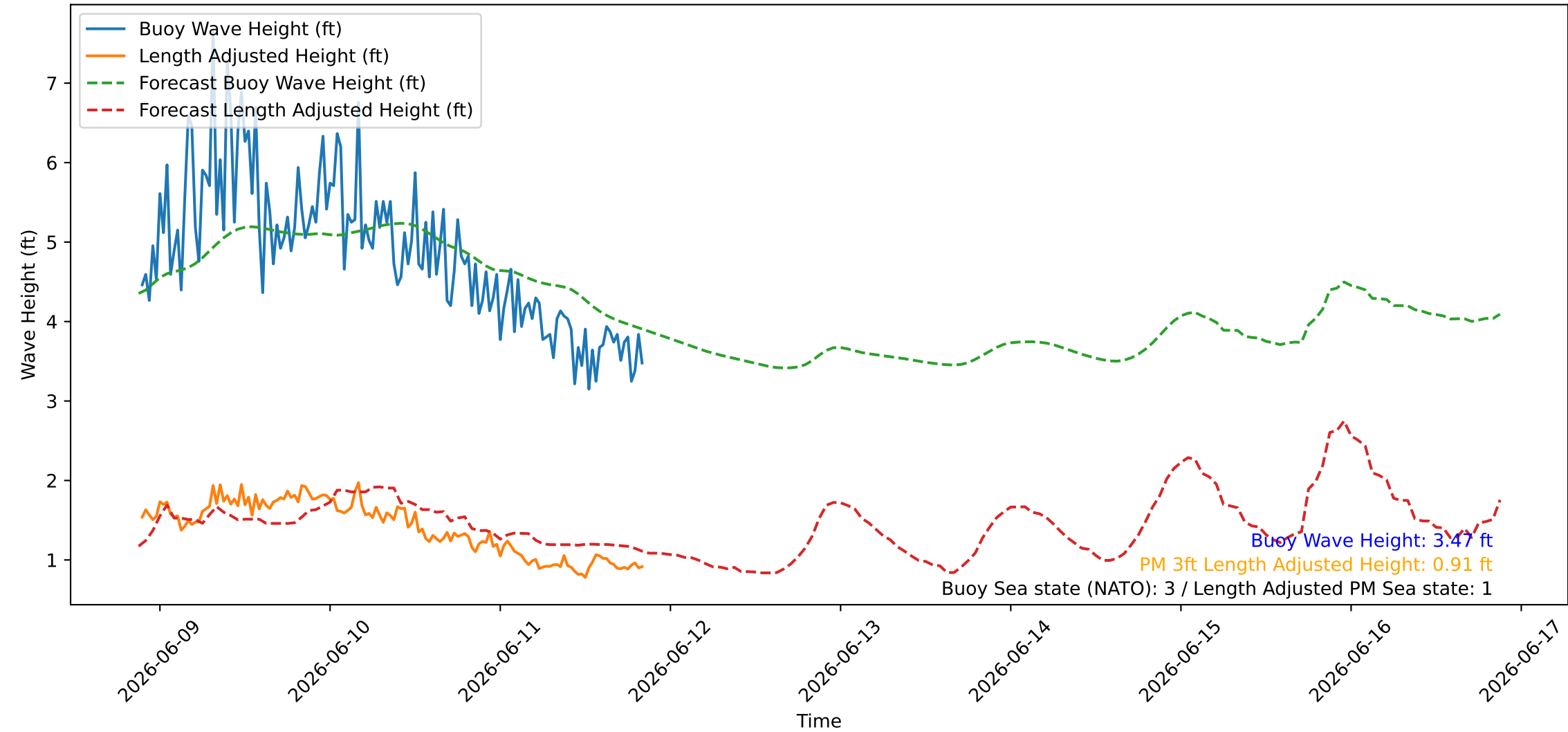
Wave Heights over Time for Red Beach at 2026-06-11 21:00:46
