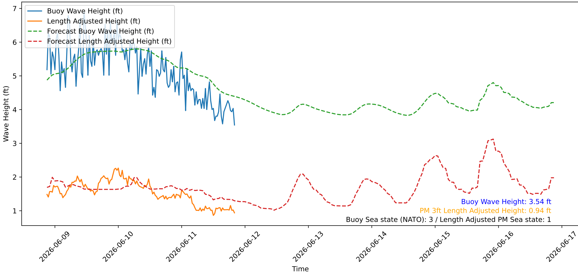
Wave Heights over Time for Green Beach at 2026-06-11 21:01:09
