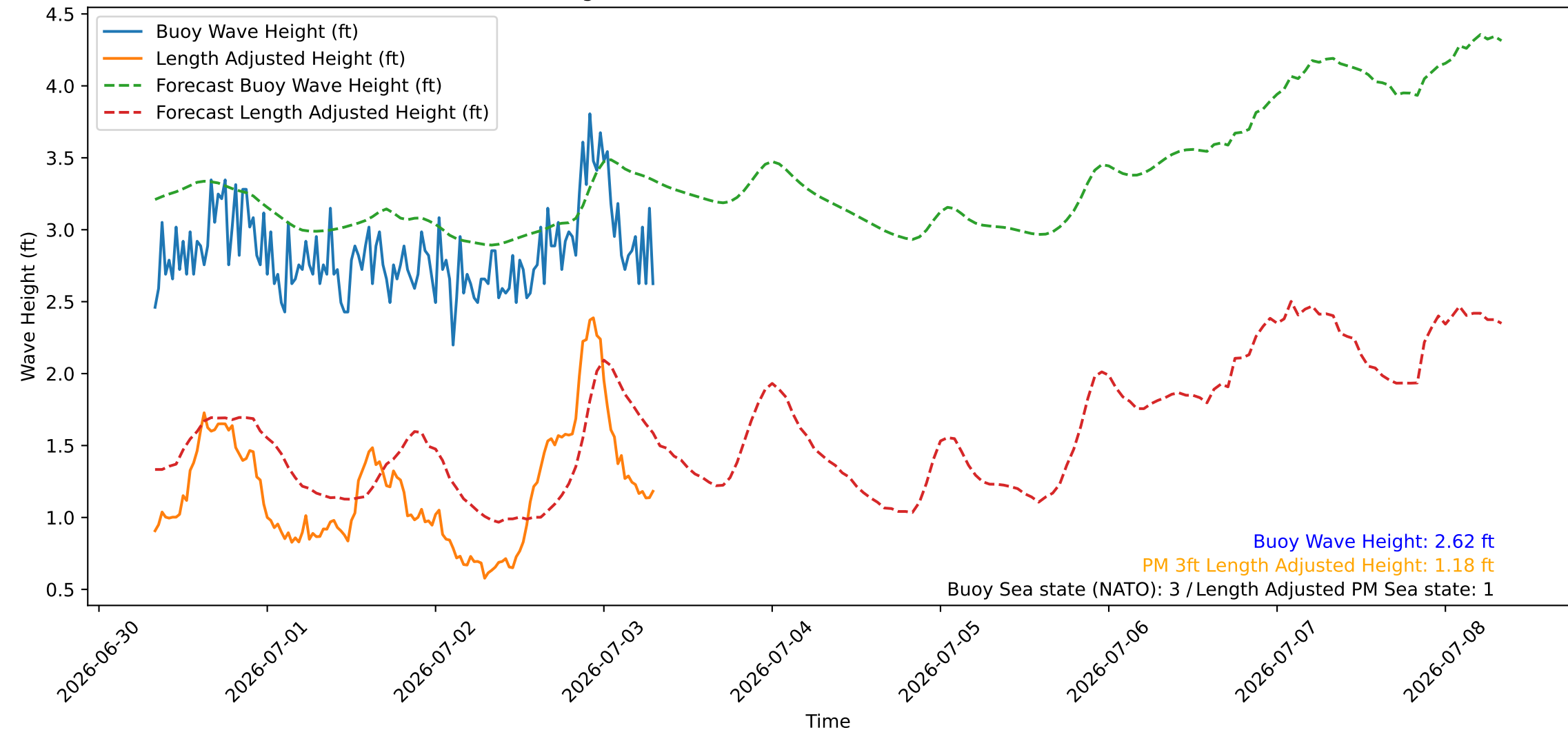
Wave Heights over Time for Red Beach at 2026-07-03 07:40:45
