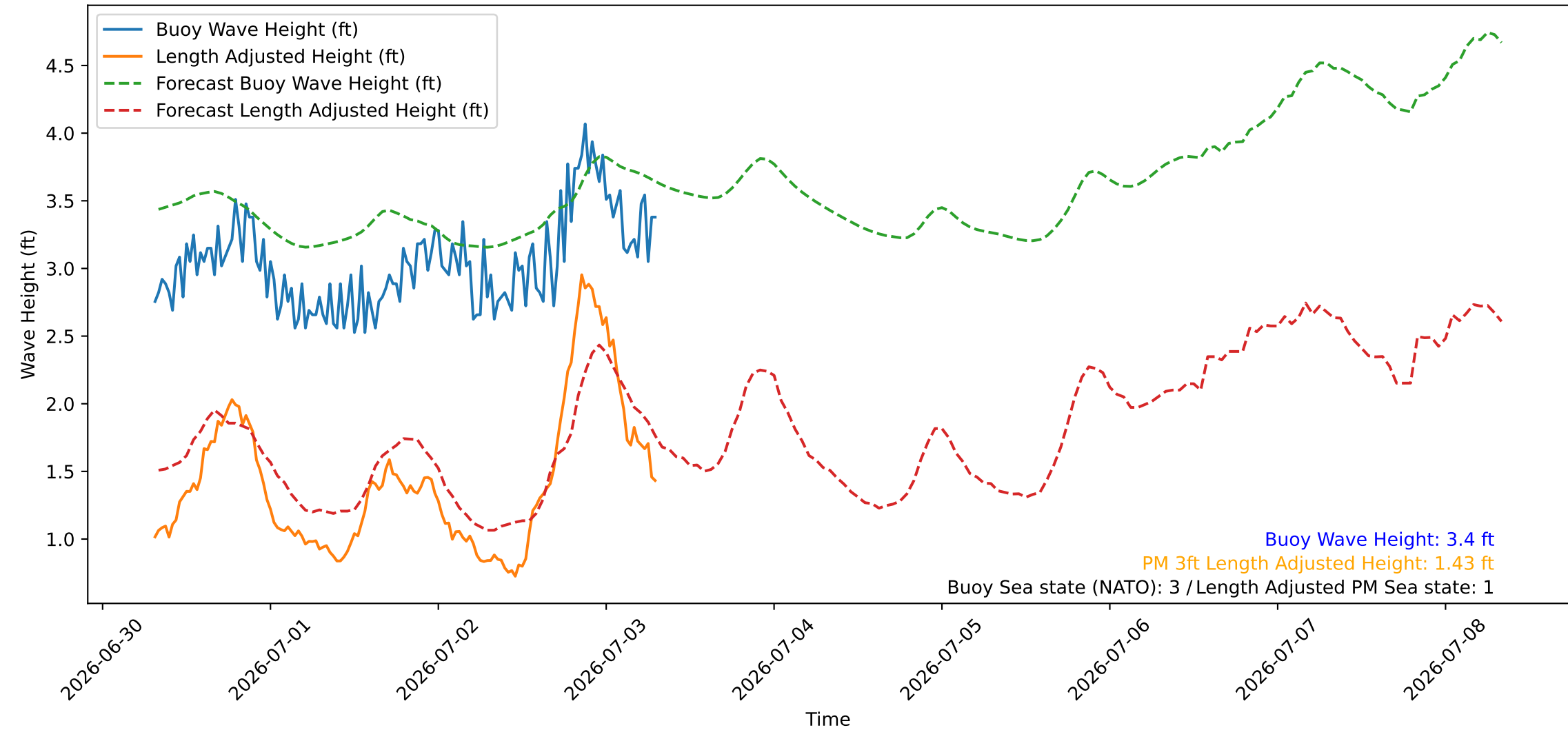
Wave Heights over Time for Green Beach at 2026-07-03 07:41:07
