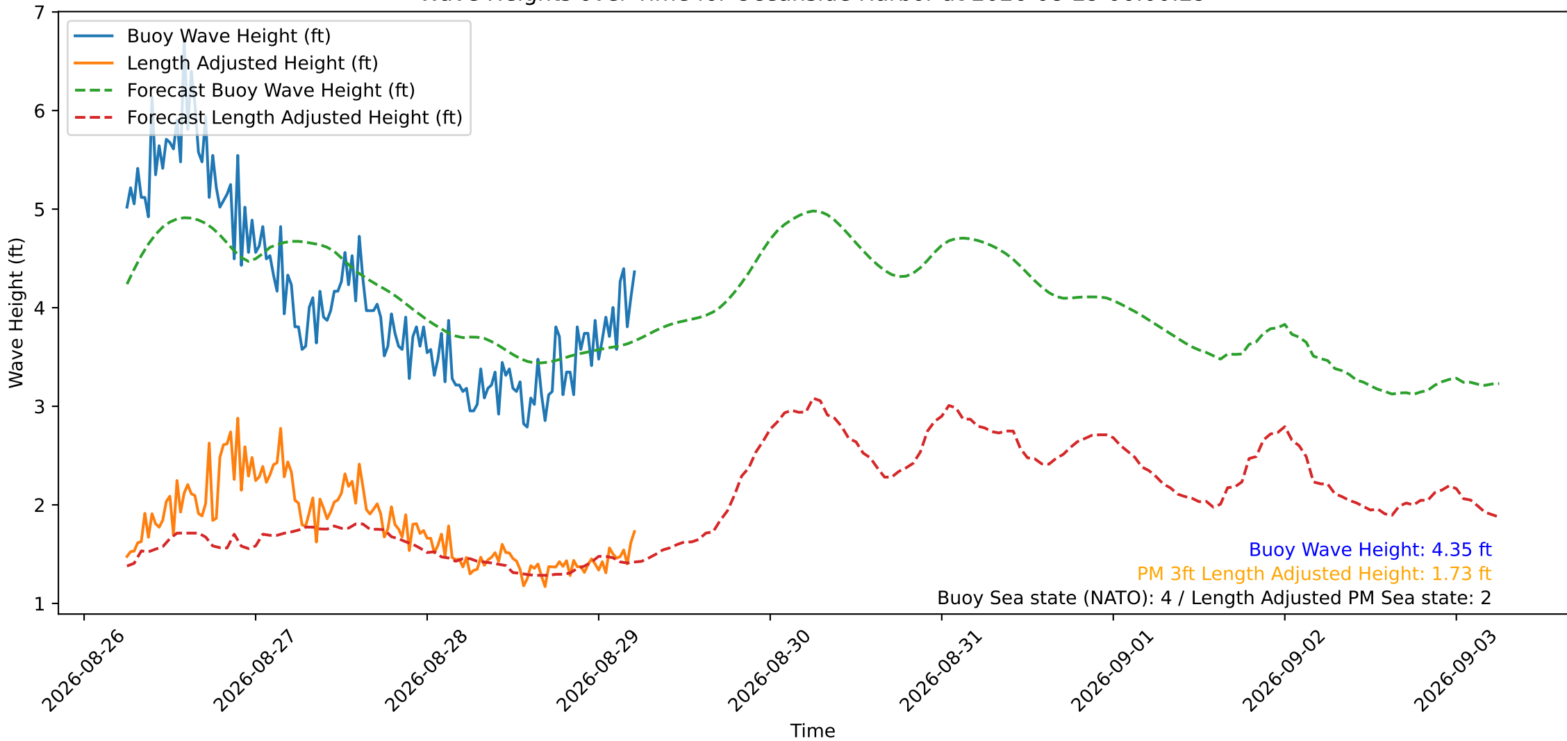
Wave Heights over Time for Oceanside Harbor at 2026-08-29 06:00:29
