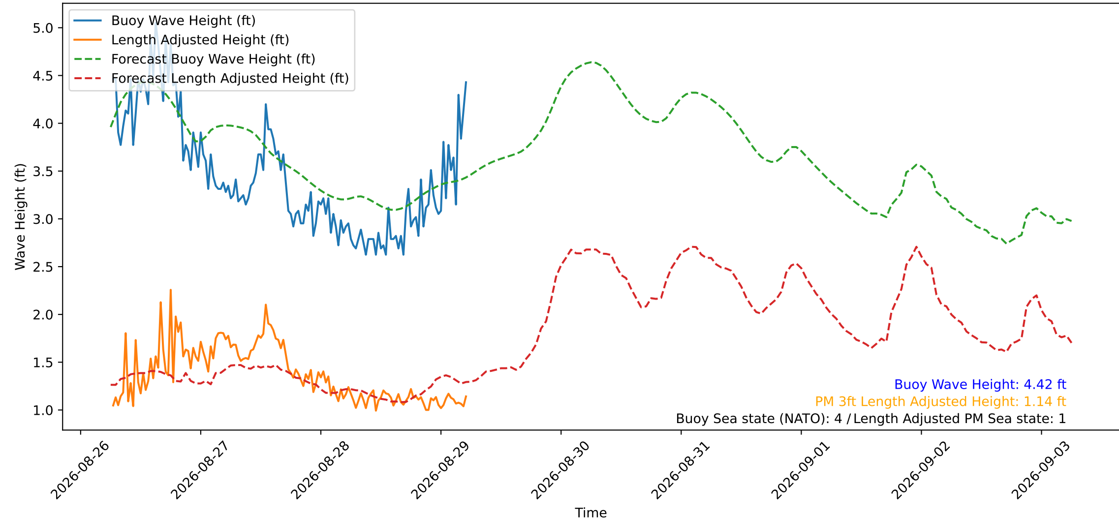
Wave Heights over Time for Red Beach at 2026-08-29 06:00:49
