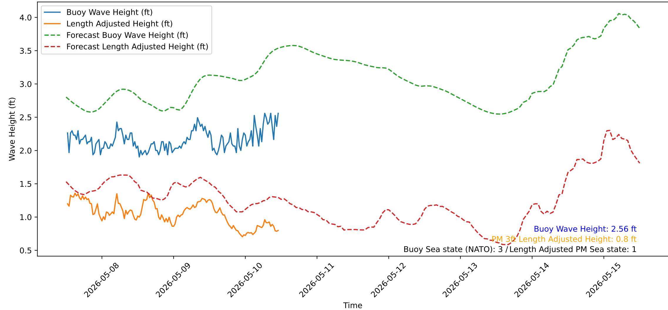
Wave Heights over Time for Red Beach at 2026-05-10 12:10:51
