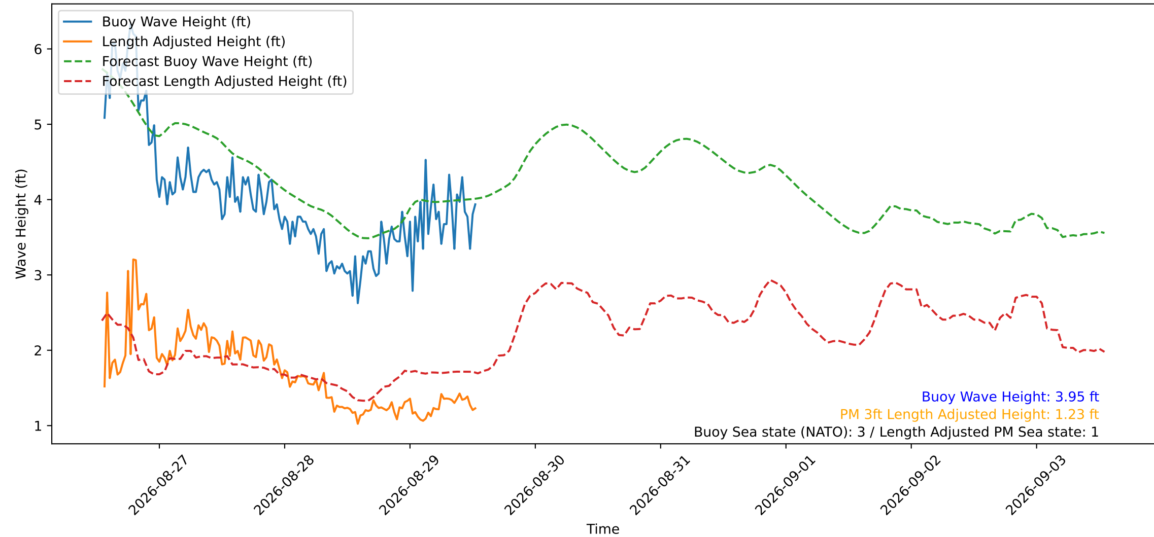
Wave Heights over Time for Green Beach at 2026-08-29 13:11:12
