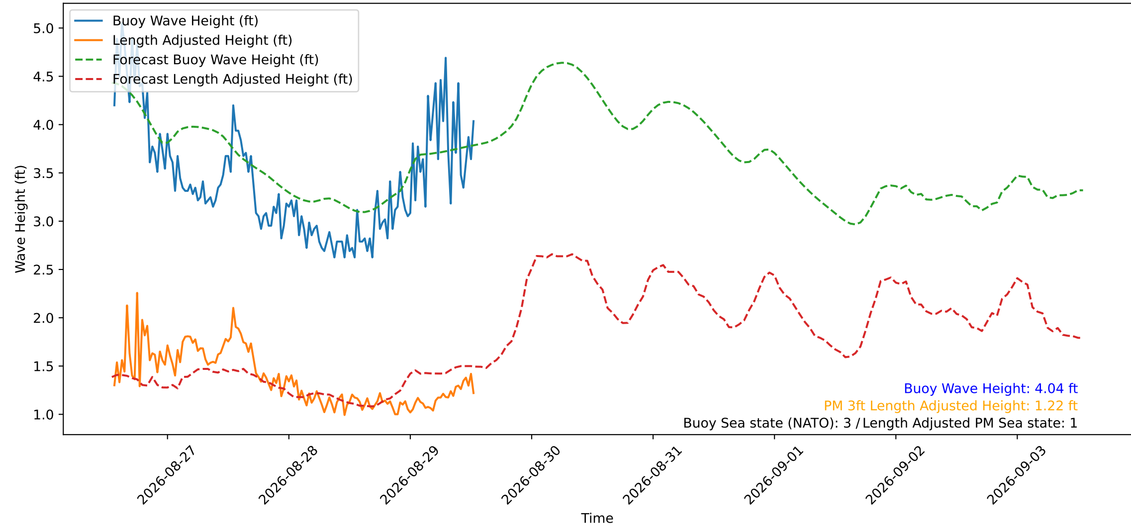
Wave Heights over Time for Red Beach at 2026-08-29 13:10:49
