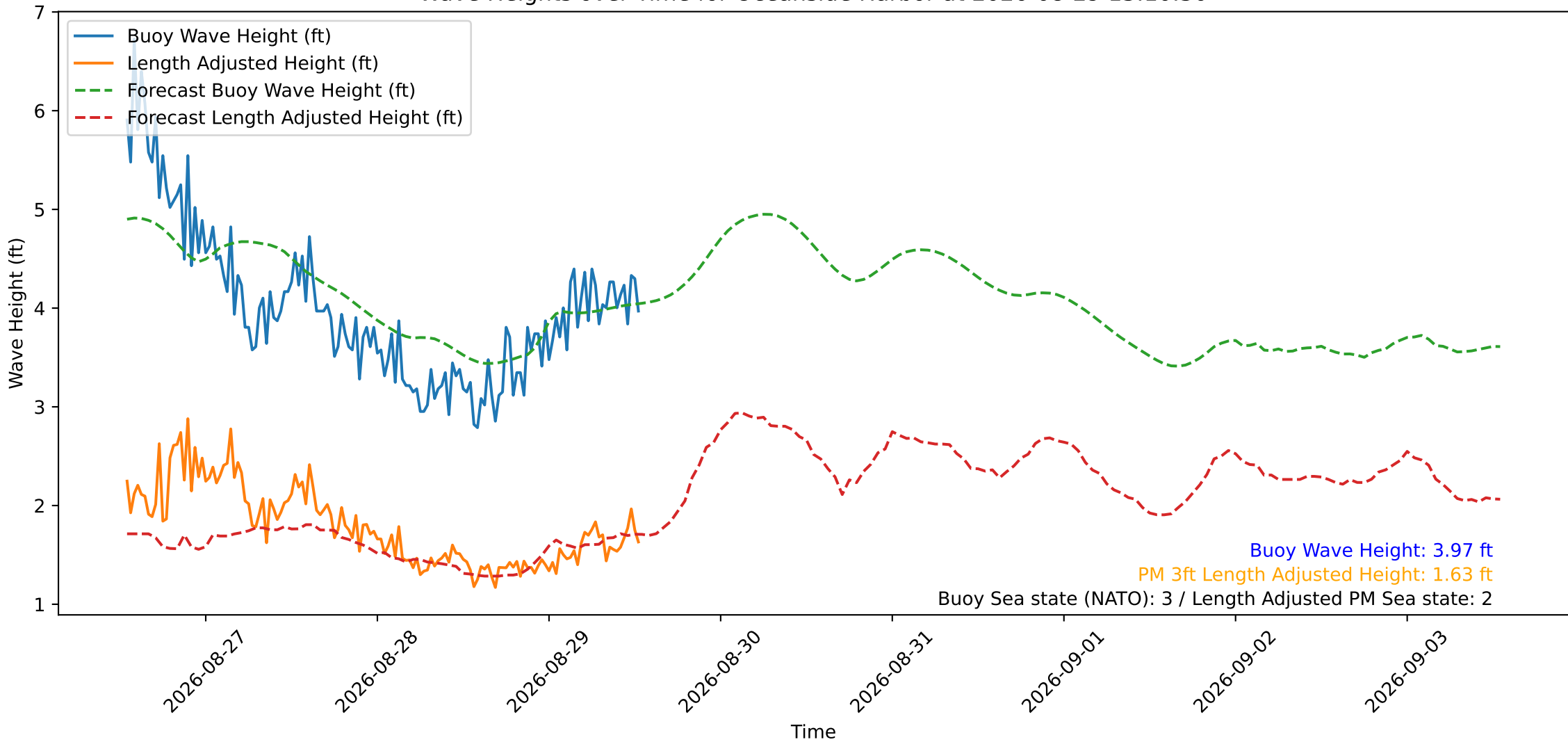
Wave Heights over Time for Oceanside Harbor at 2026-08-29 13:10:30
