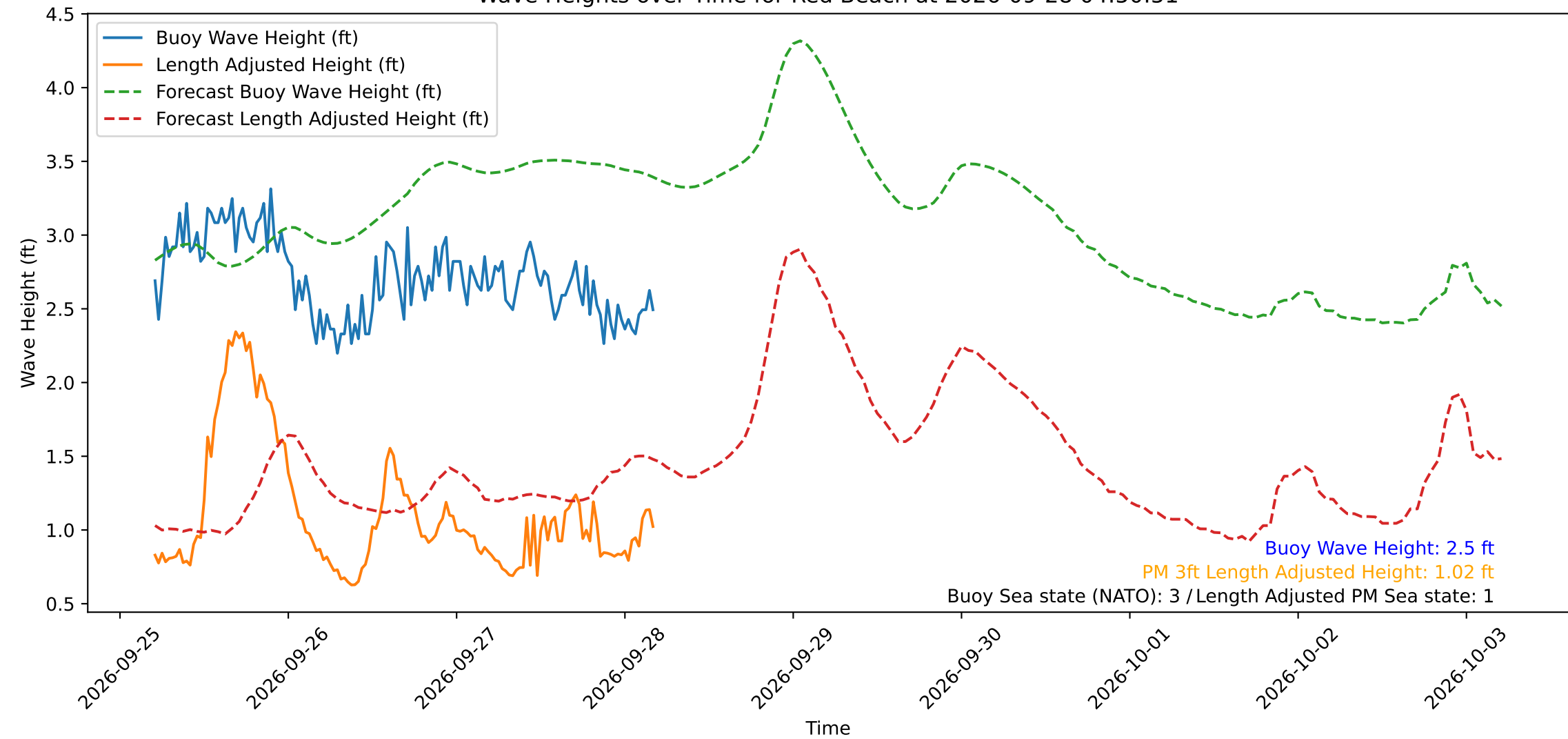
Wave Heights over Time for Red Beach at 2026-09-28 04:50:51
