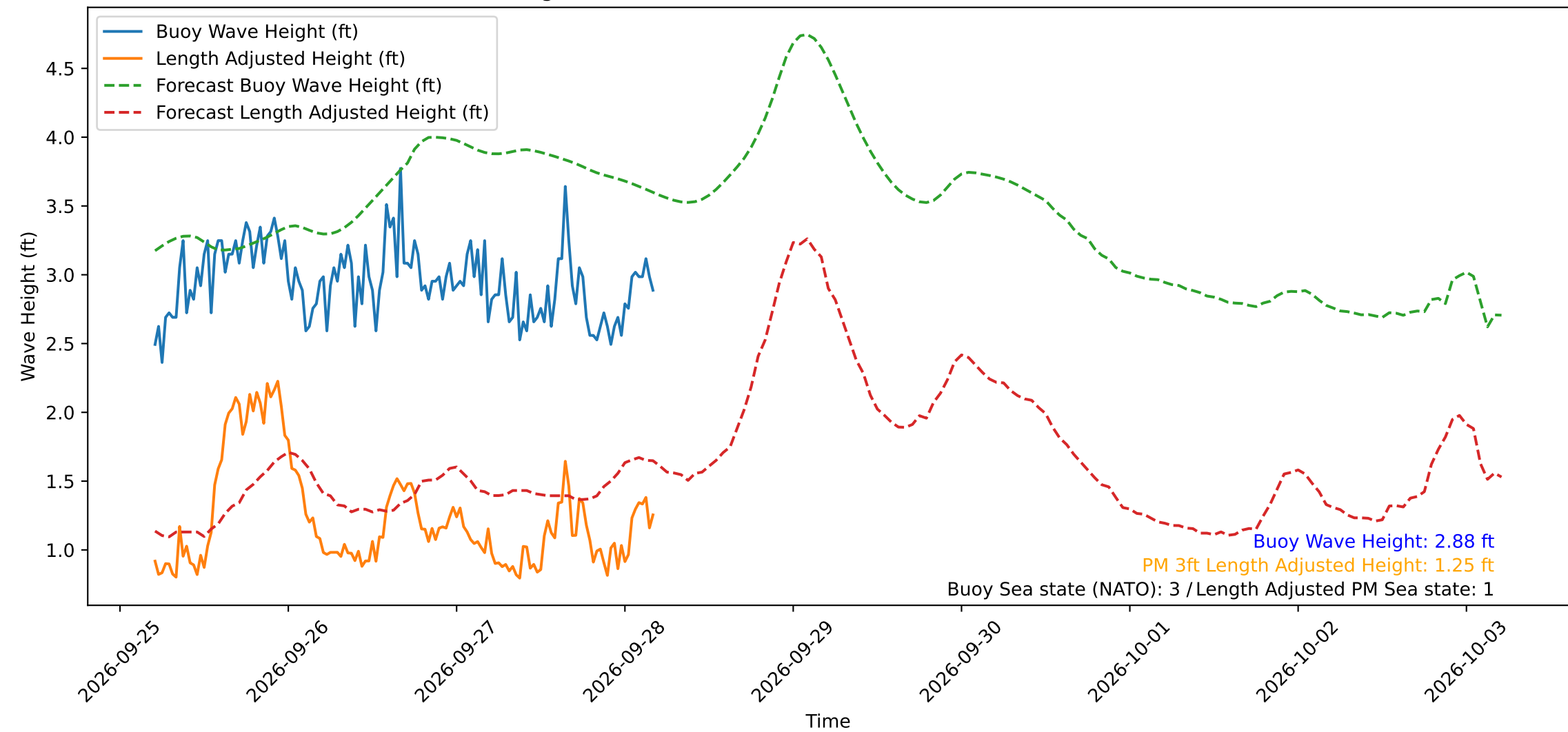
Wave Heights over Time for Oceanside Harbor at 2026-09-28 04:50:30
