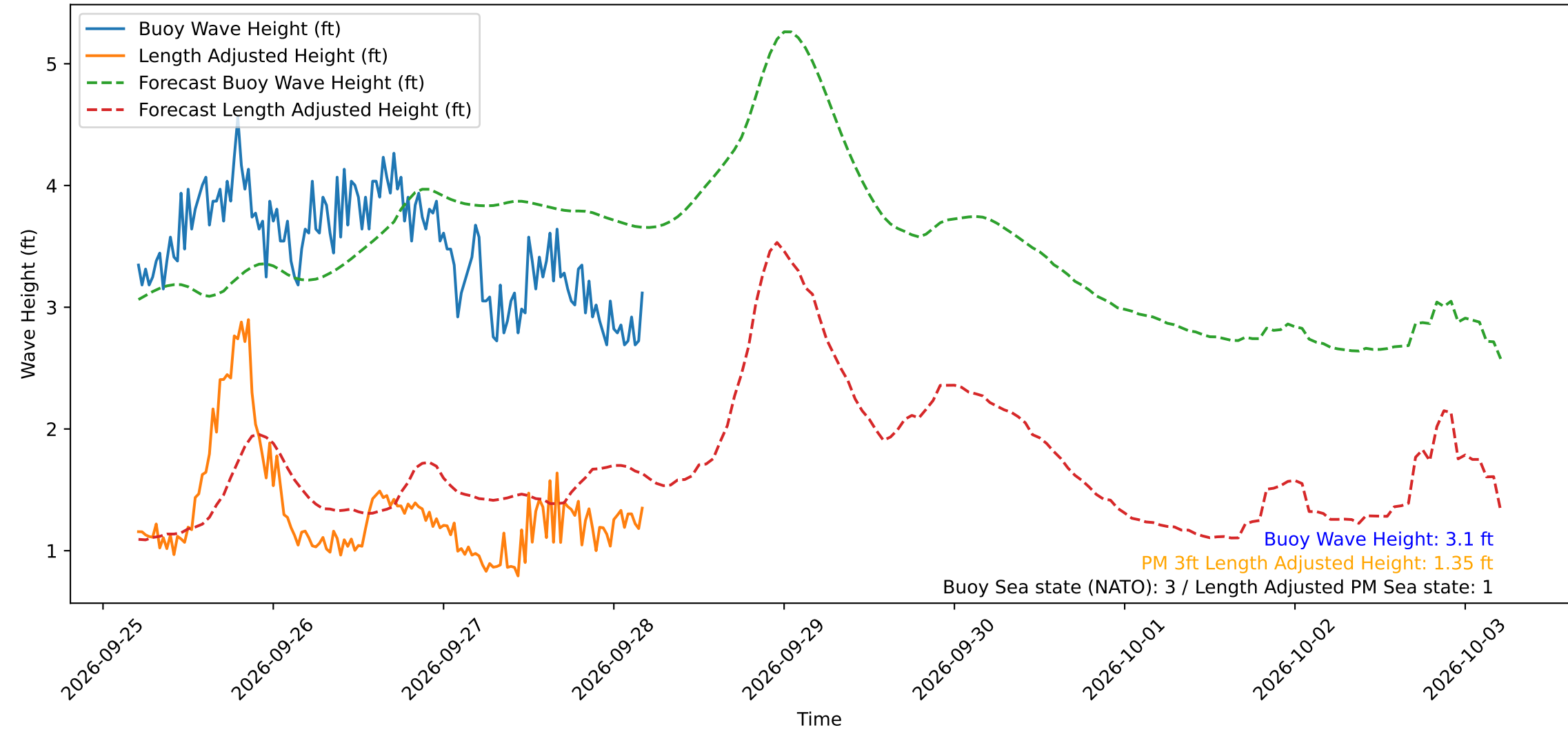
Wave Heights over Time for Green Beach at 2026-09-28 04:51:15
