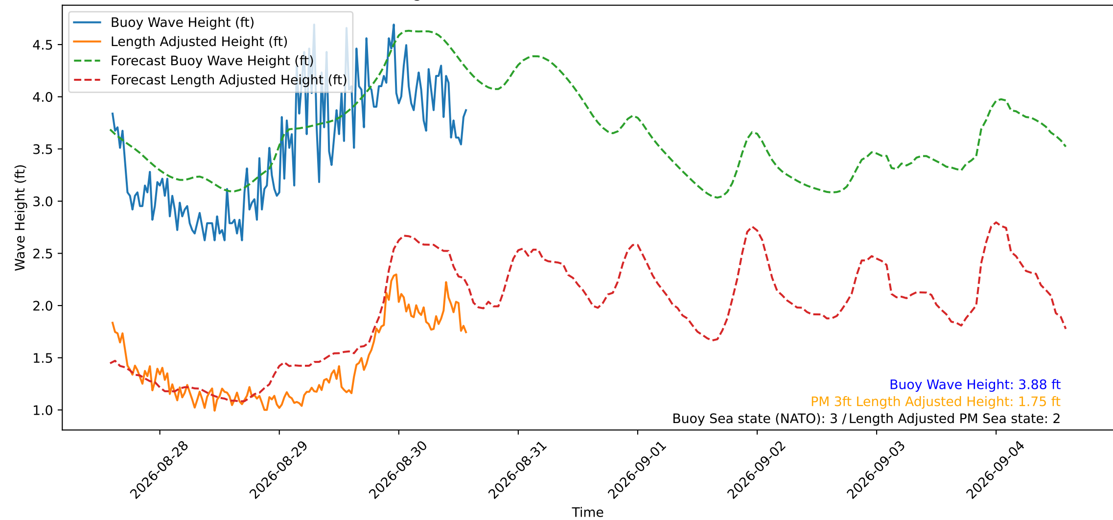
Wave Heights over Time for Red Beach at 2026-08-30 14:20:51
