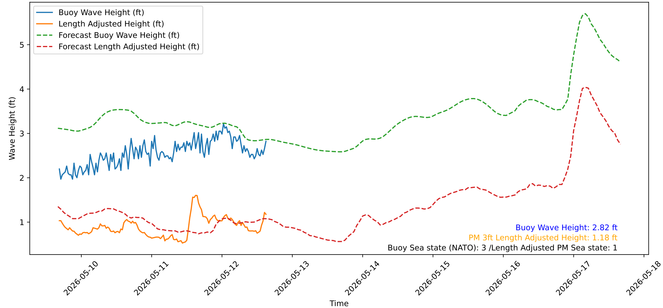
Wave Heights over Time for Red Beach at 2026-05-12 16:20:52
