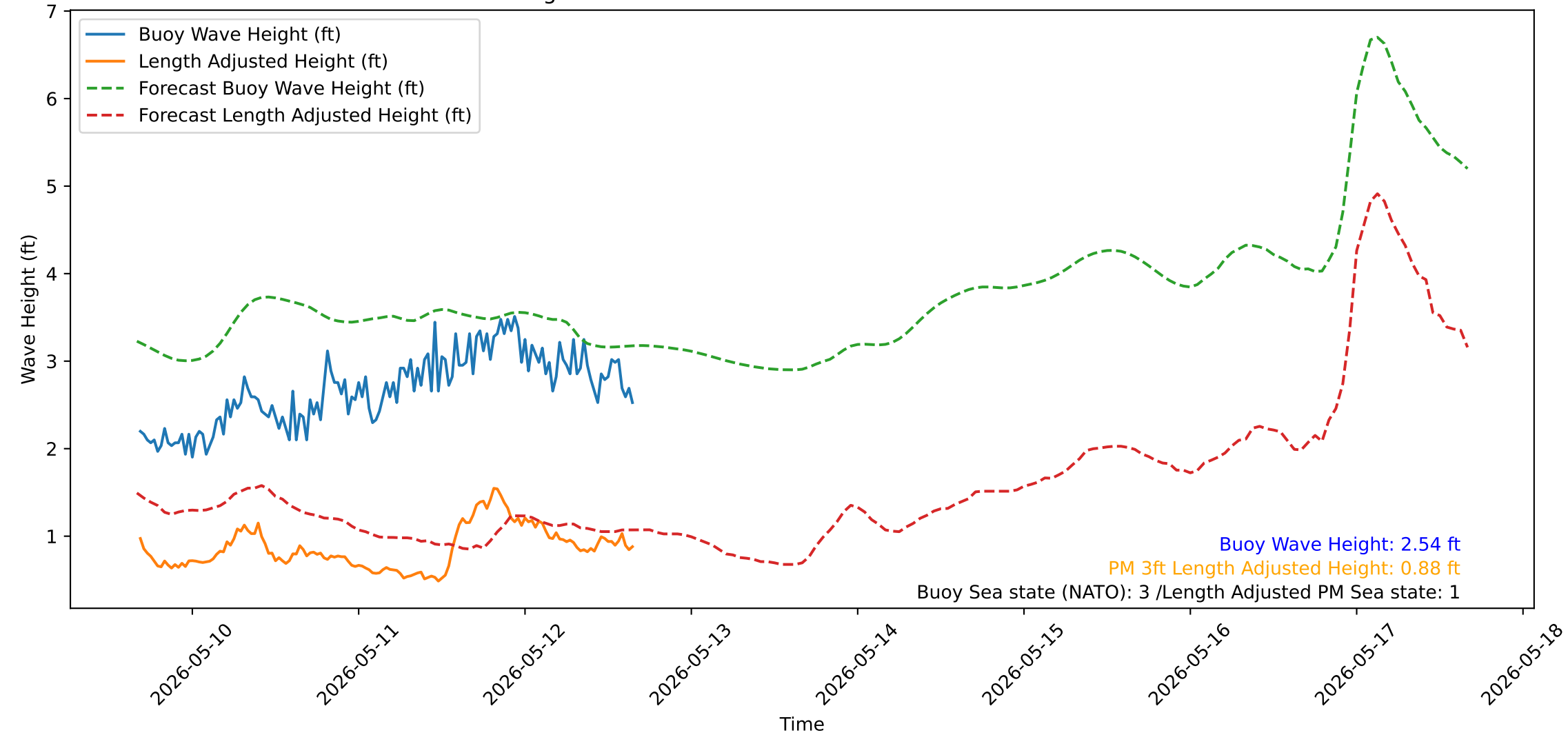
Wave Heights over Time for Green Beach at 2026-05-12 16:21:14
