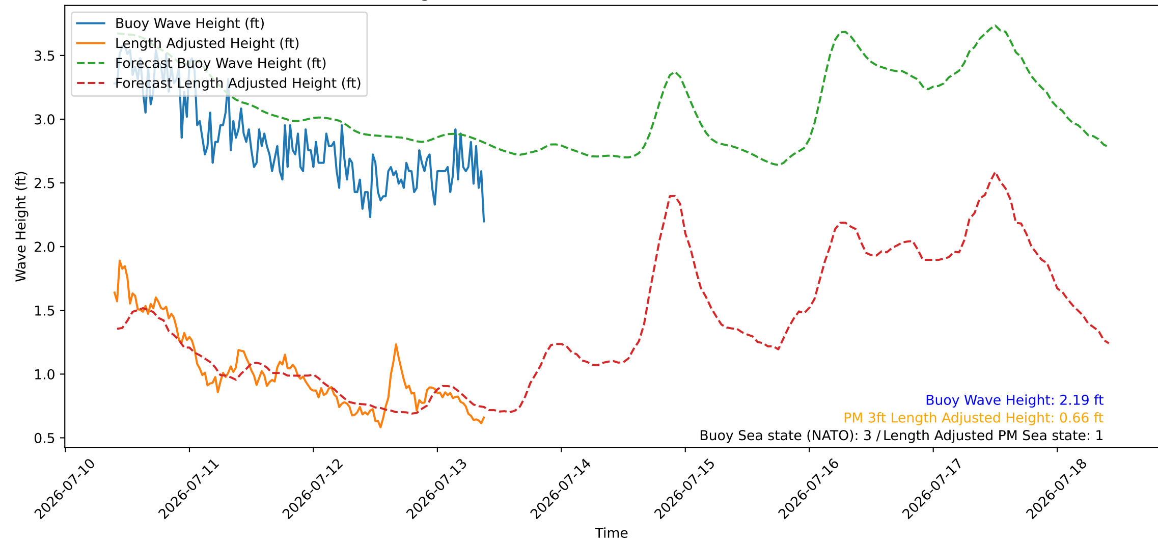
Wave Heights over Time for Green Beach at 2026-07-13 09:41:09
