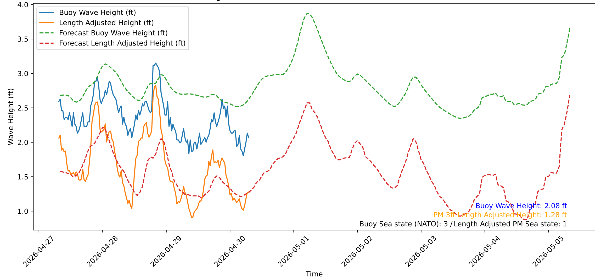
Wave Heights over Time for Green Beach at 2026-04-30 07:41:13
