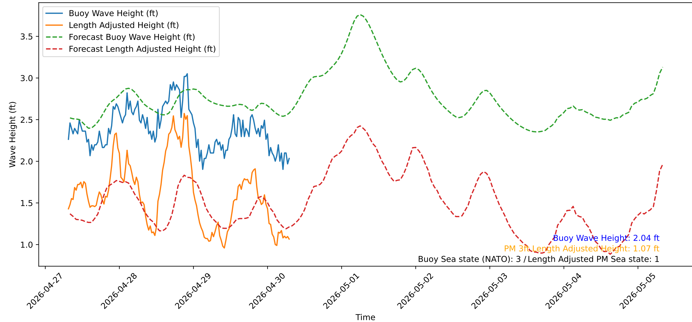
Wave Heights over Time for Oceanside Harbor at 2026-04-30 07:40:31
