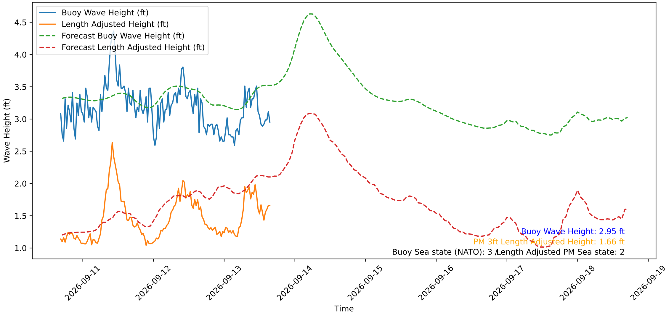
Wave Heights over Time for Oceanside Harbor at 2026-09-13 16:30:29
