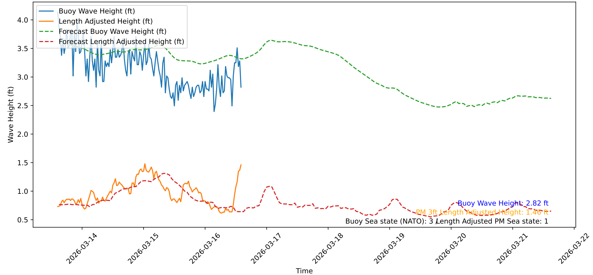
Wave Heights over Time for Oceanside Harbor at 2026-03-16 14:40:49
