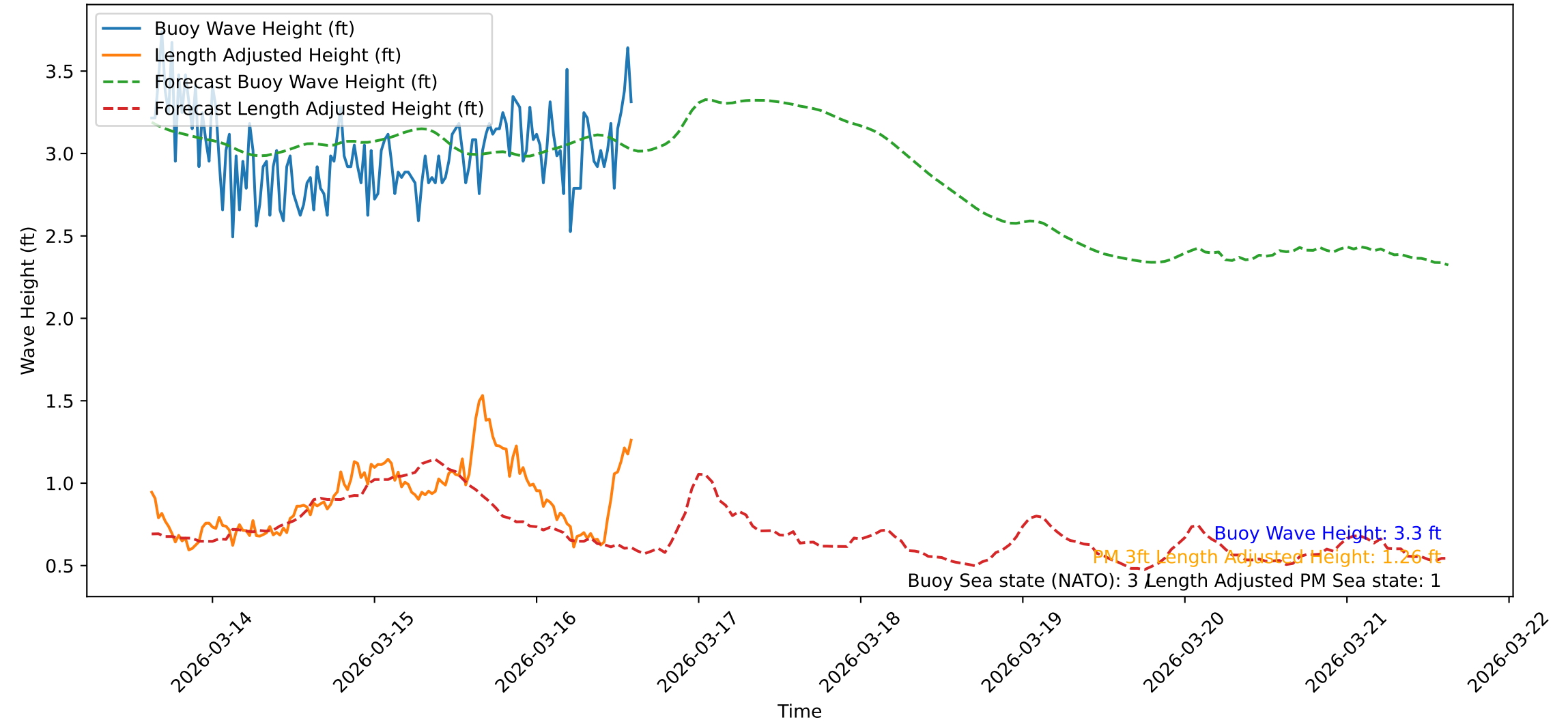
Wave Heights over Time for Red Beach at 2026-03-16 14:41:15
