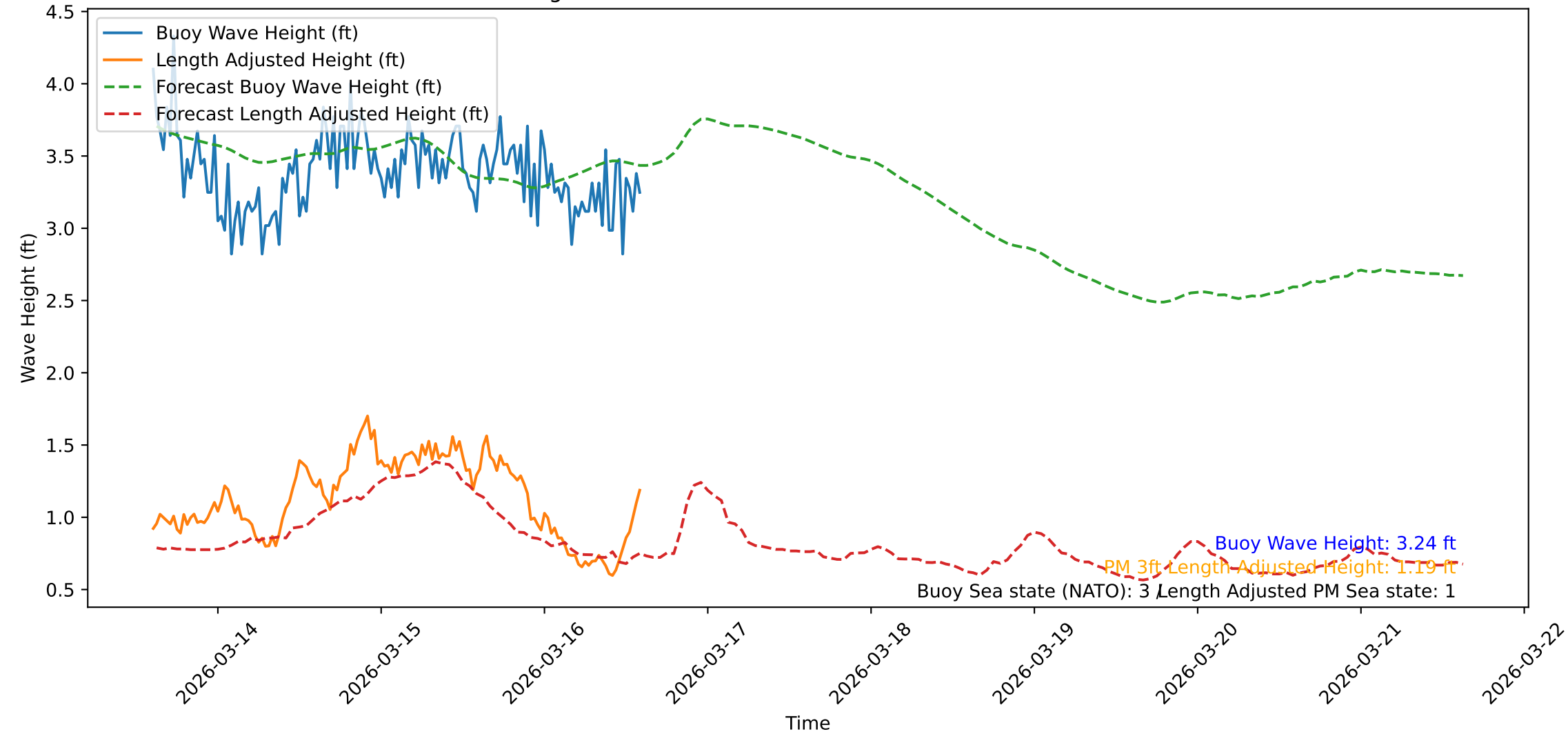
Wave Heights over Time for Green Beach at 2026-03-16 14:41:56
