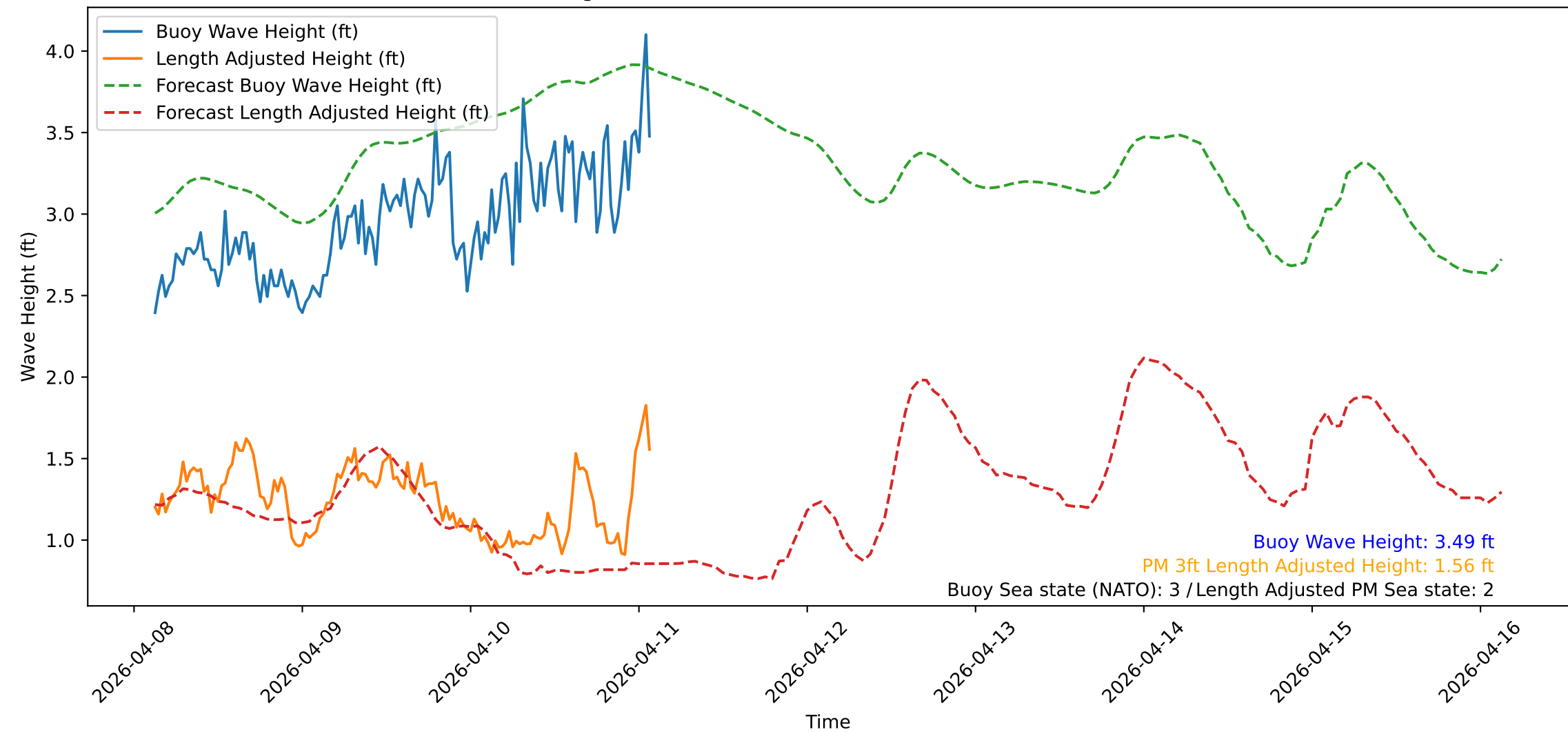
Wave Heights over Time for Red Beach at 2026-04-11 02:30:51
