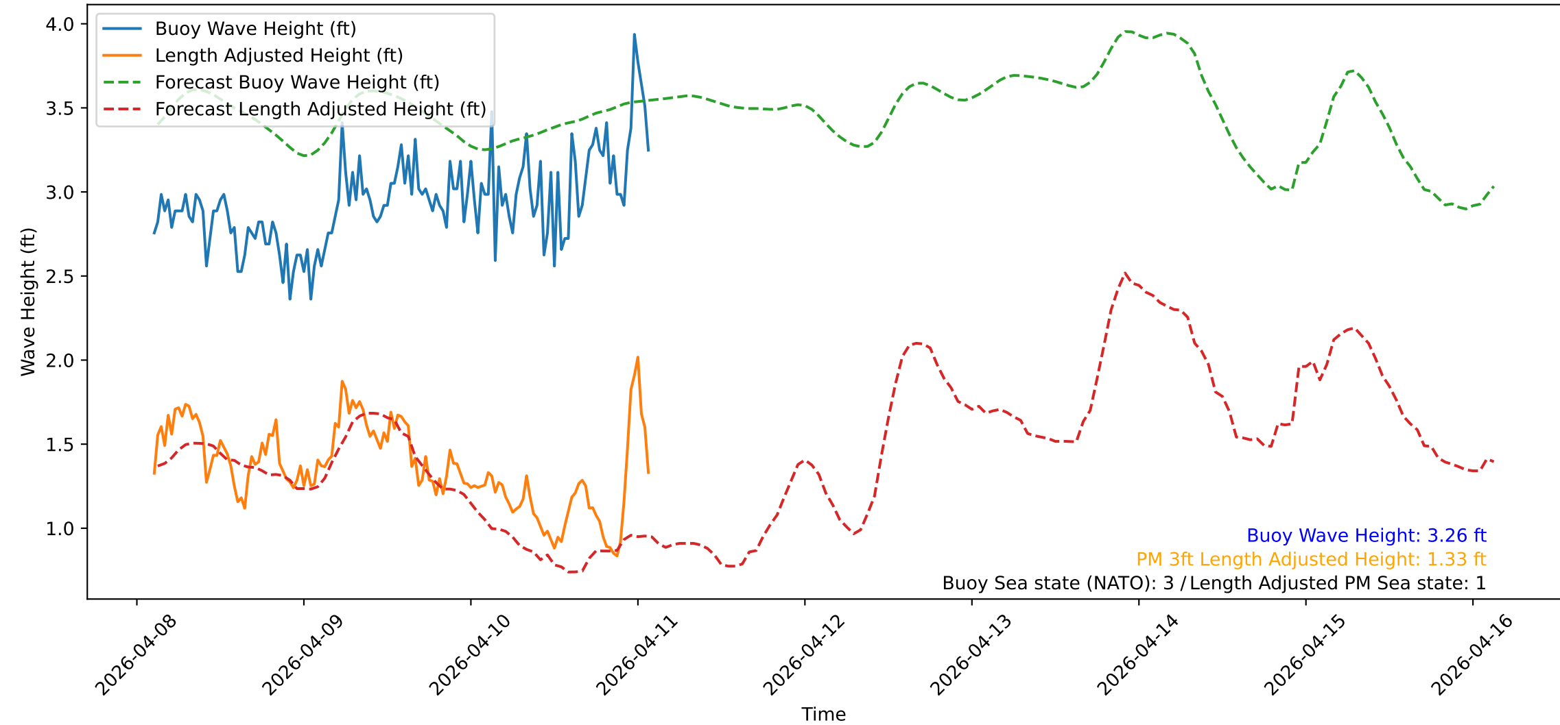
Wave Heights over Time for Green Beach at 2026-04-11 02:31:13
