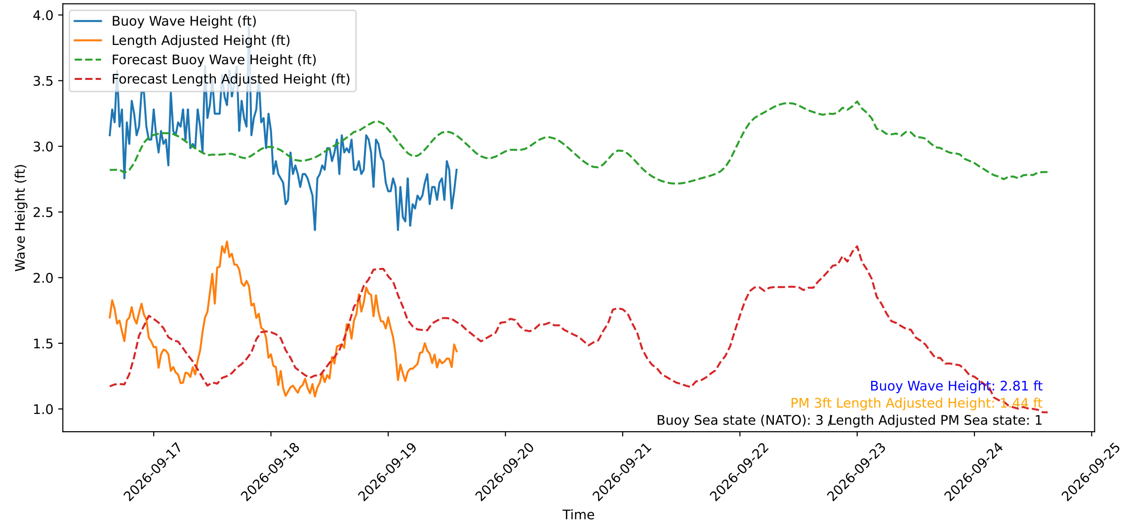
Wave Heights over Time for Oceanside Harbor at 2026-09-19 15:00:30
