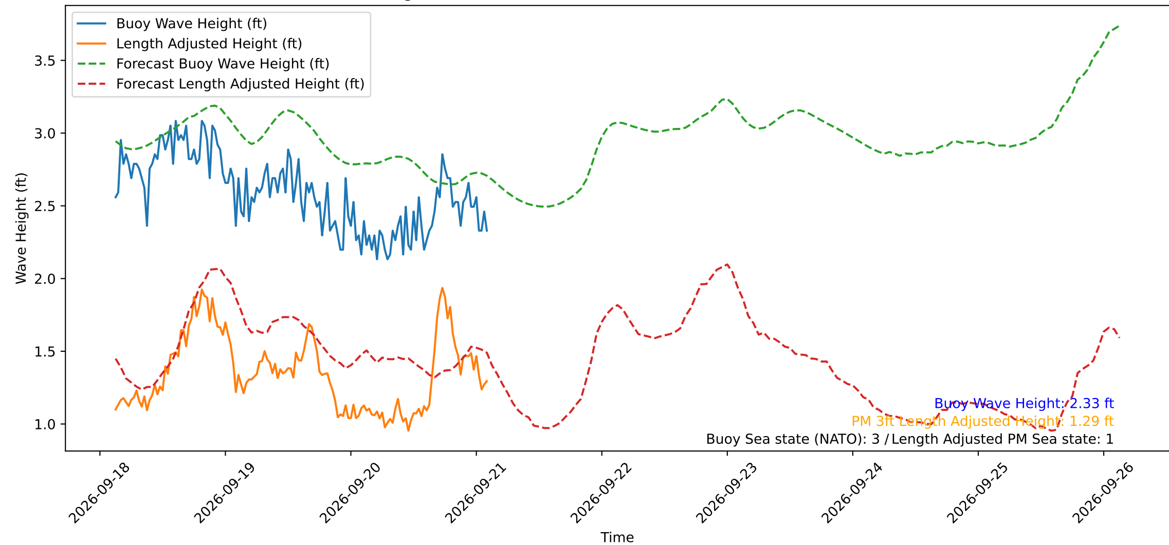
Wave Heights over Time for Oceanside Harbor at 2026-09-21 02:50:30
