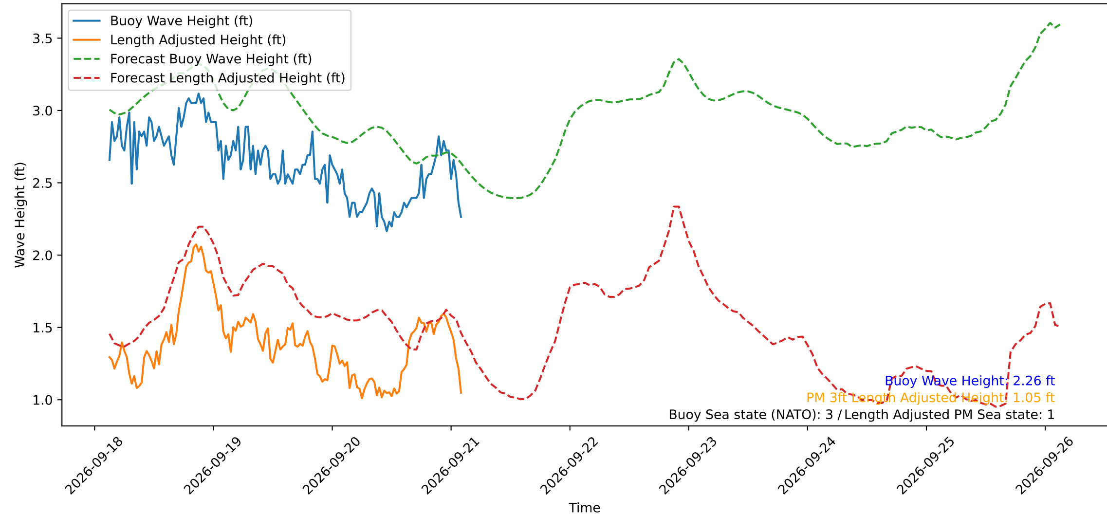
Wave Heights over Time for Green Beach at 2026-09-21 02:51:16
