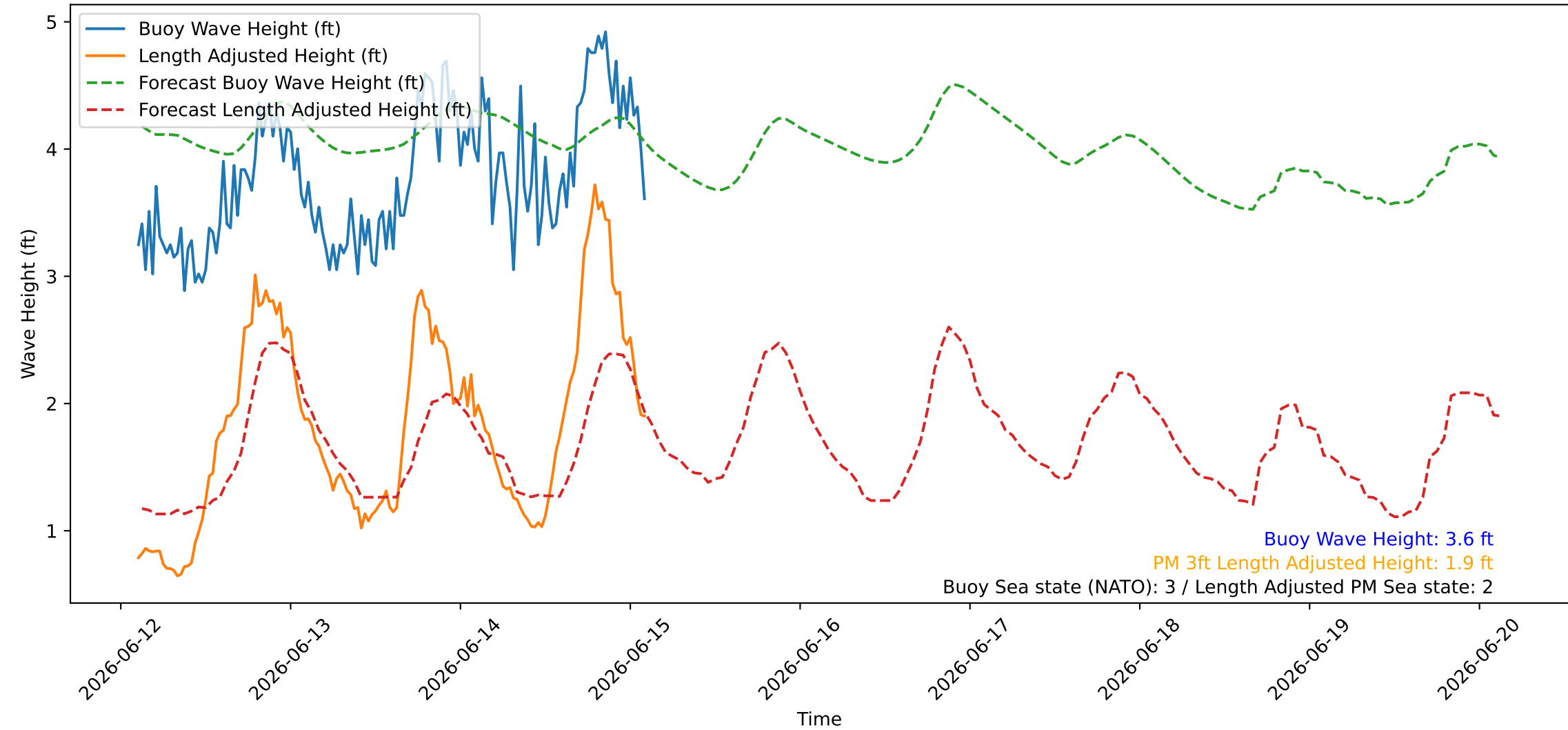
Wave Heights over Time for Green Beach at 2026-06-15 02:41:07
