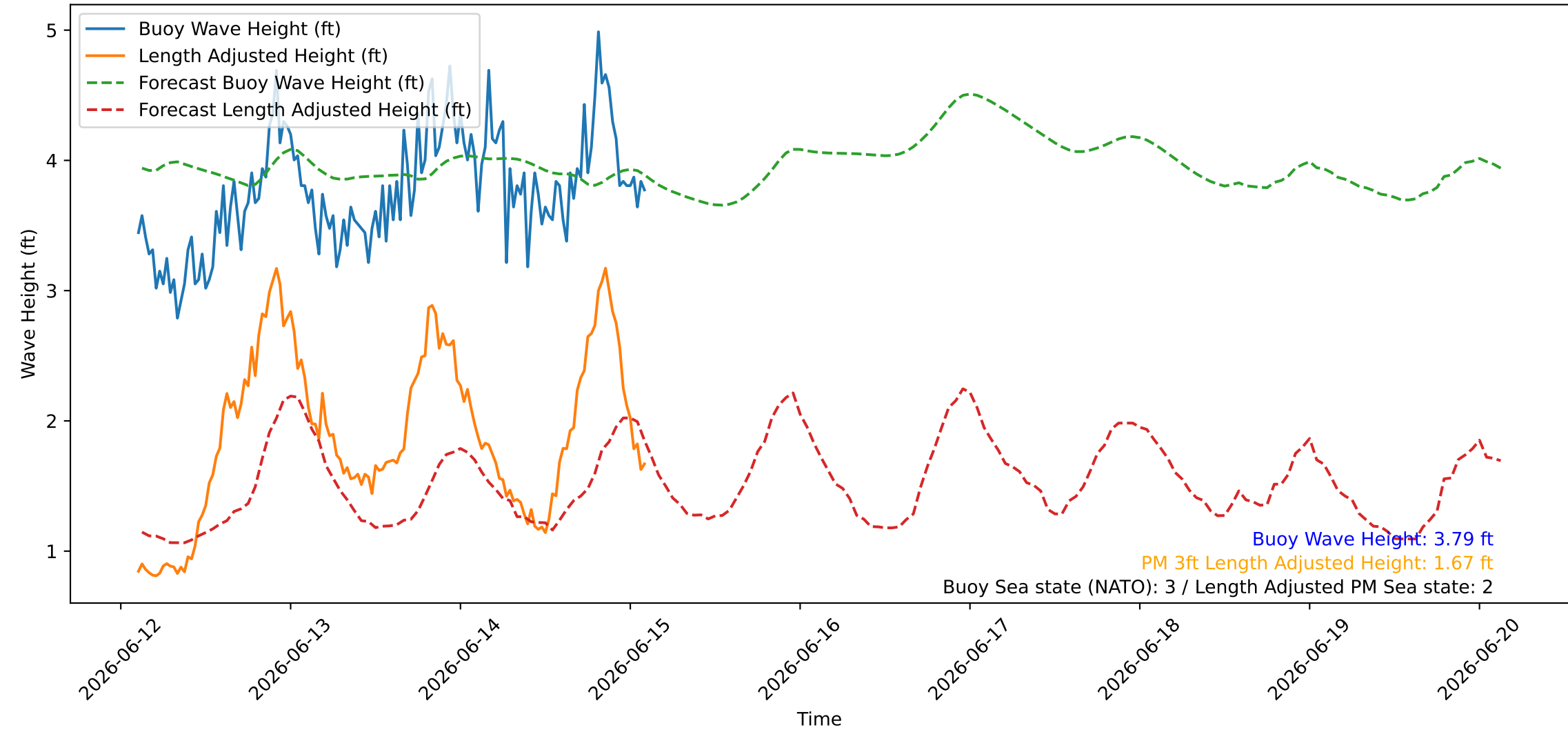
Wave Heights over Time for Oceanside Harbor at 2026-06-15 02:40:26
