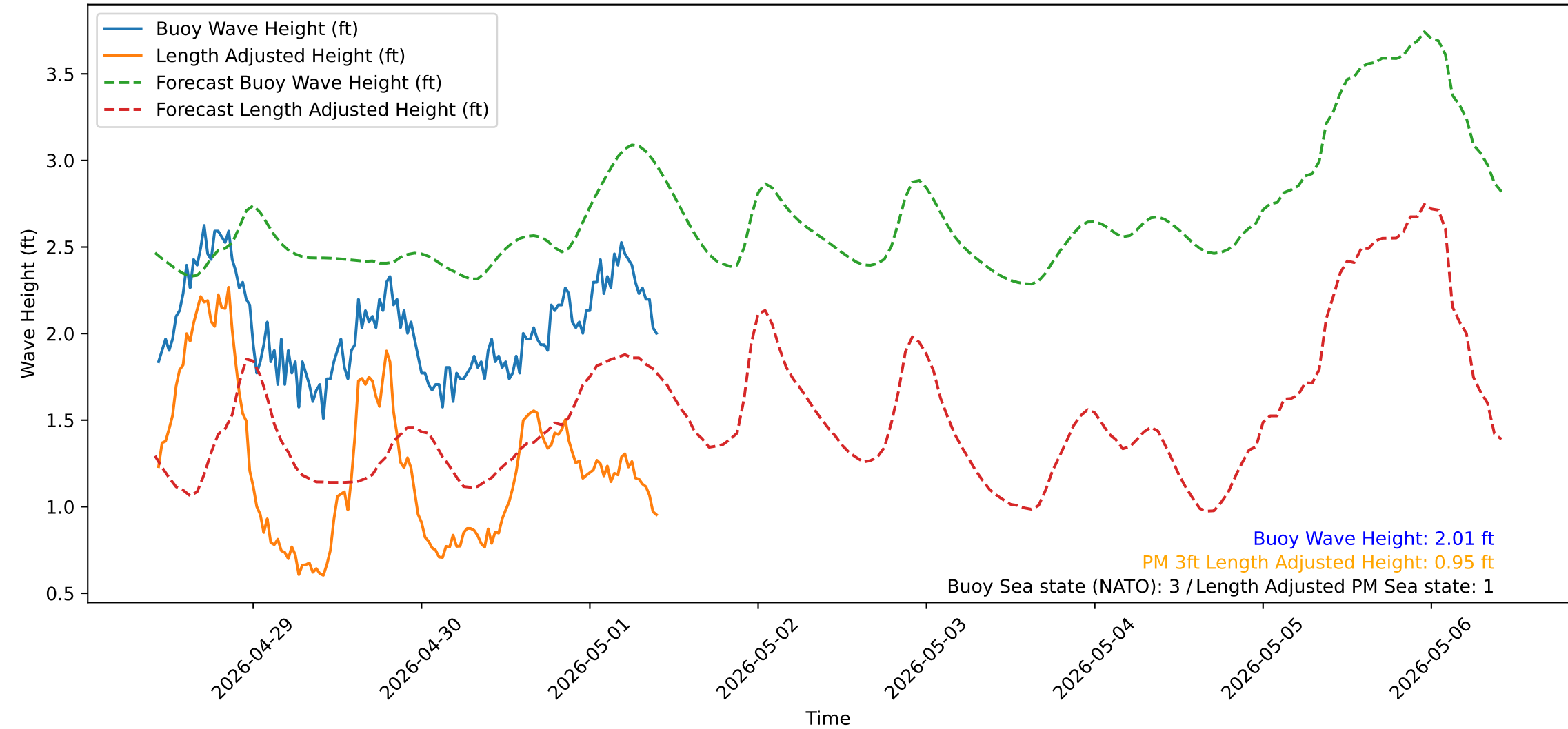
Wave Heights over Time for Red Beach at 2026-05-01 10:20:52
