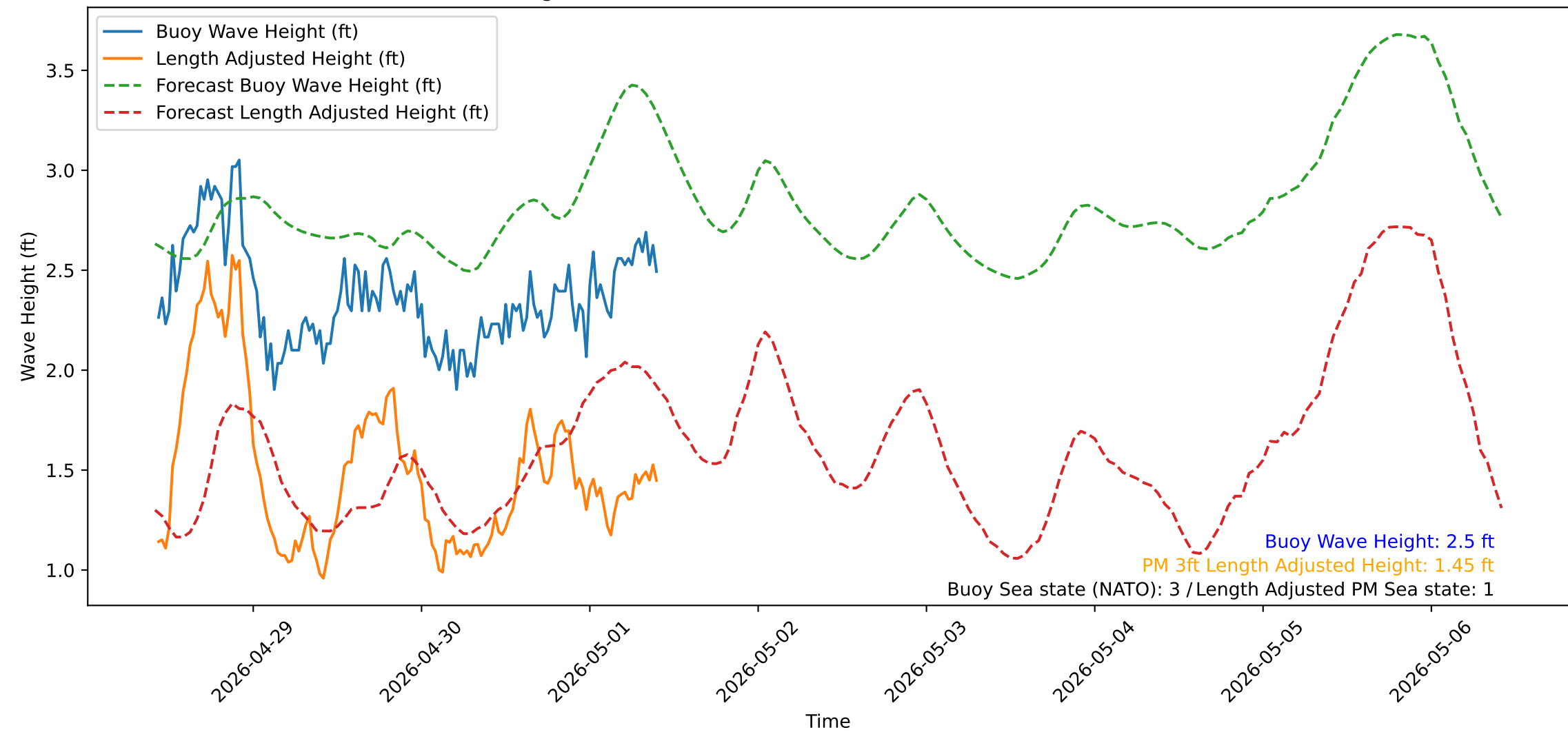
Wave Heights over Time for Oceanside Harbor at 2026-05-01 10:20:31
