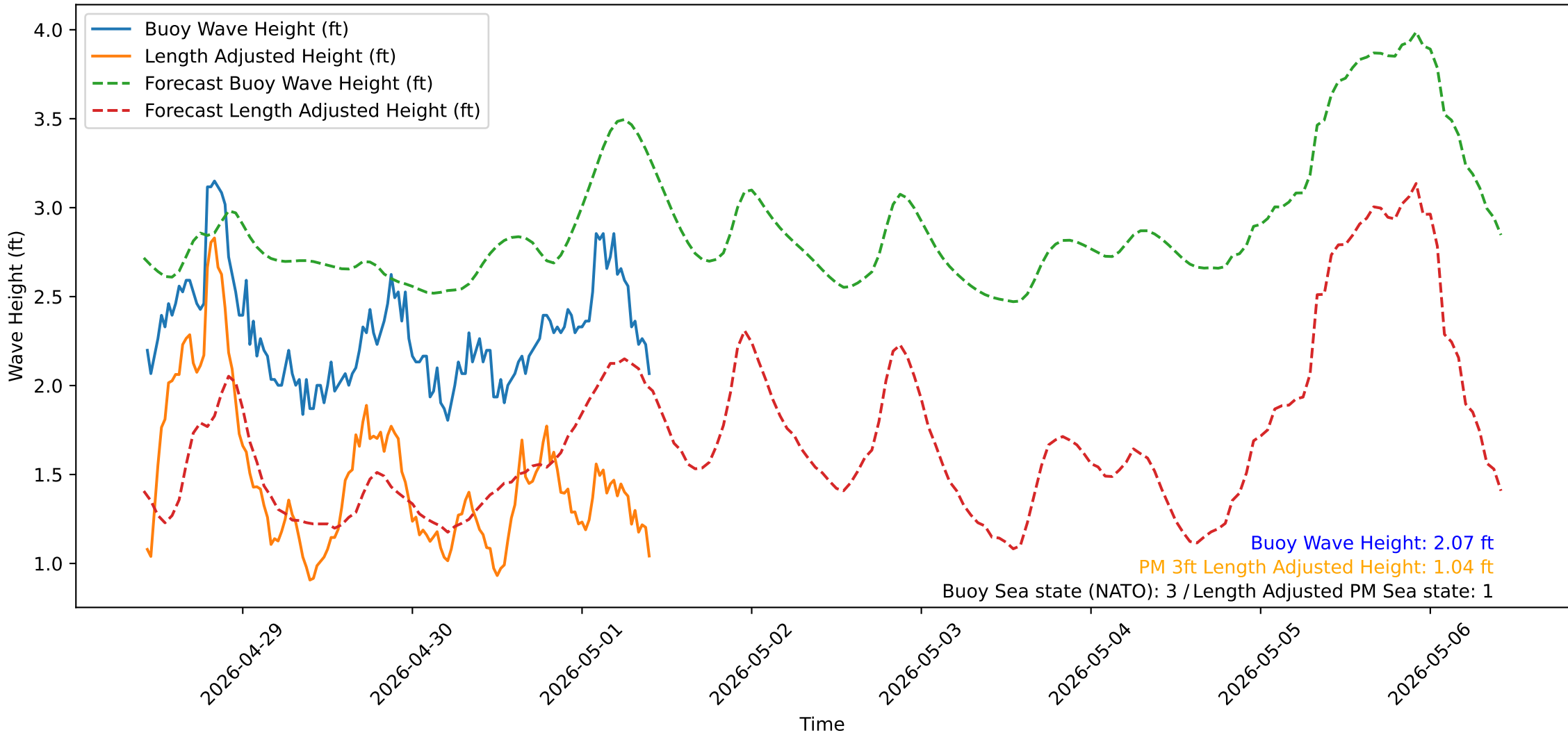
Wave Heights over Time for Green Beach at 2026-05-01 10:21:14
