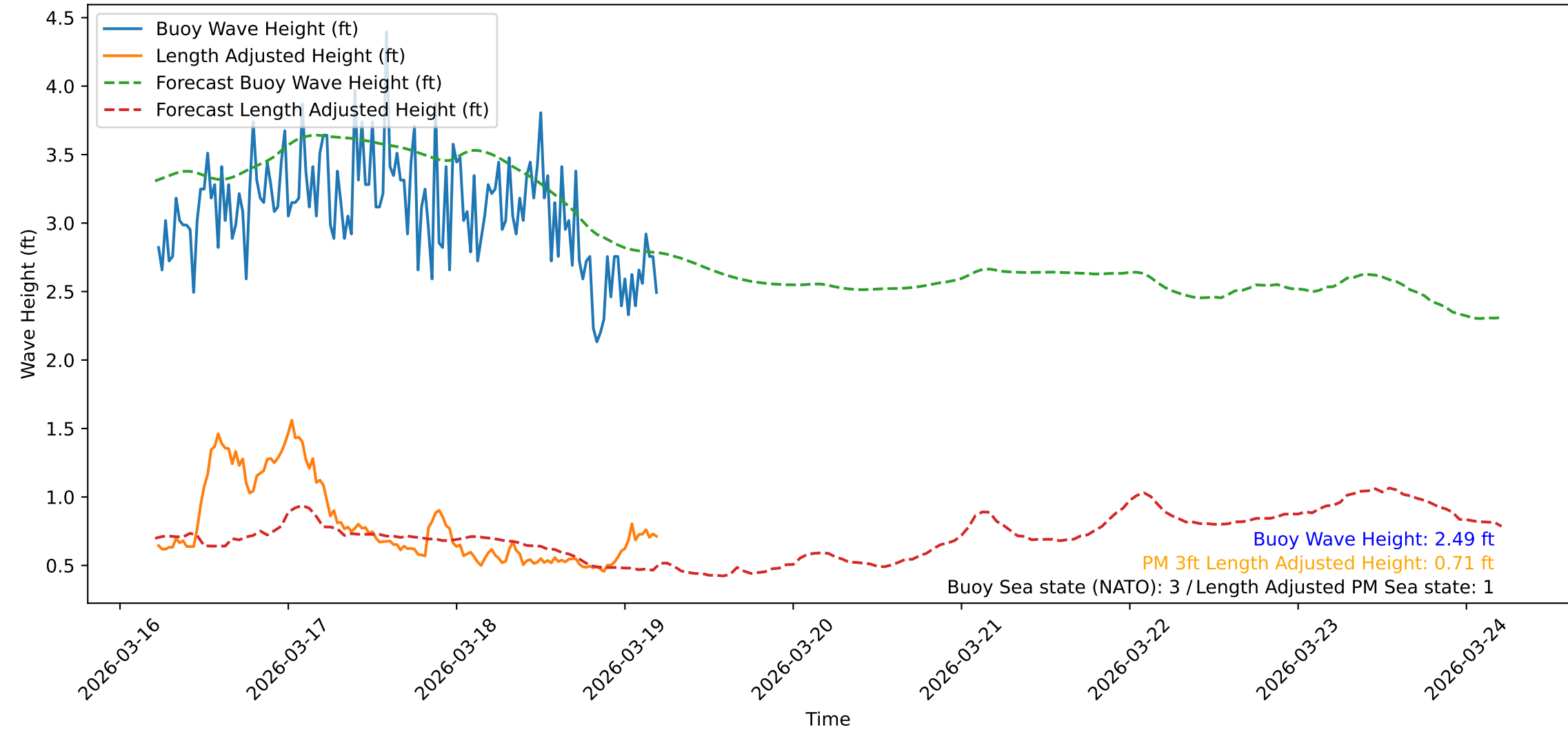
Wave Heights over Time for Oceanside Harbor at 2026-03-19 05:20:32
