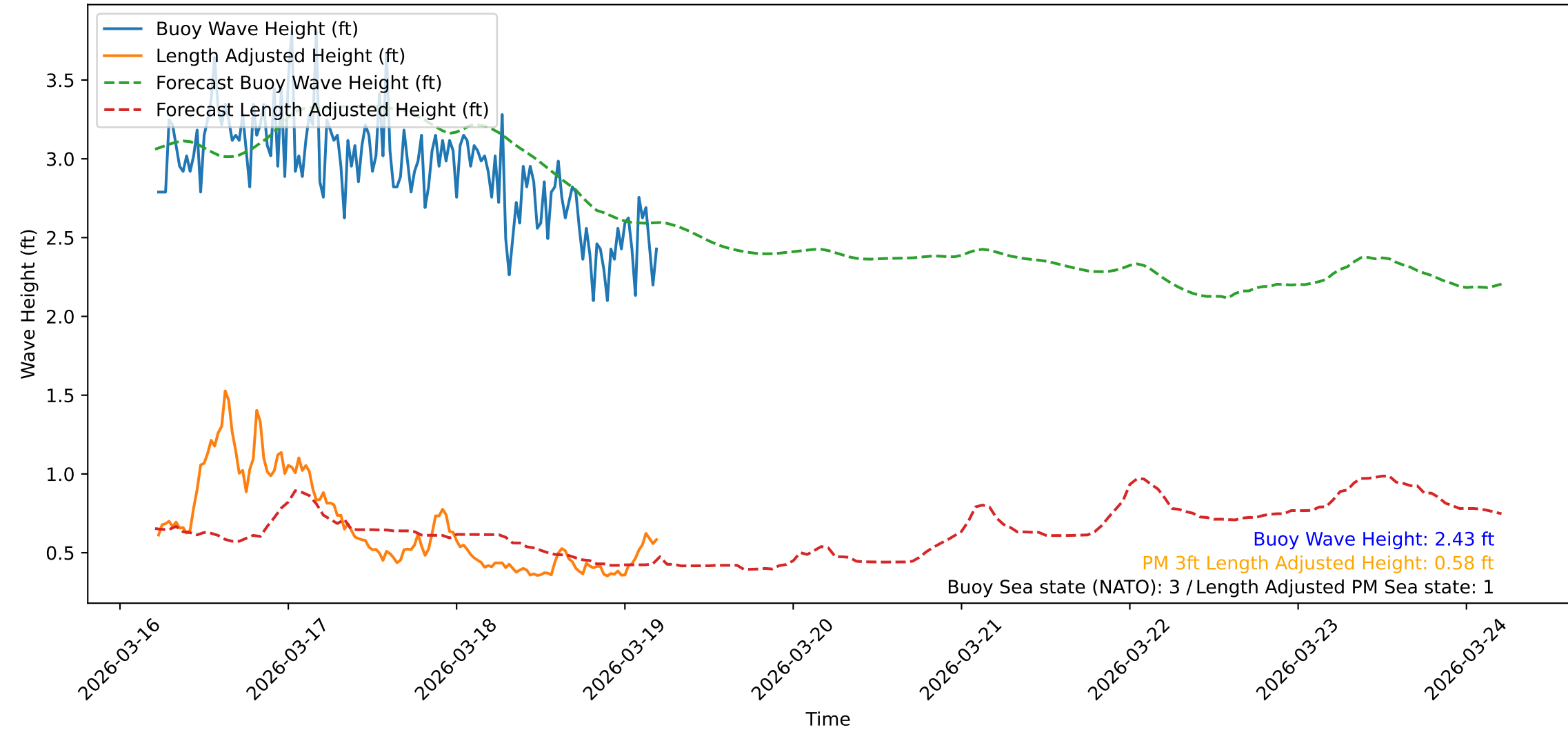
Wave Heights over Time for Red Beach at 2026-03-19 05:20:48
