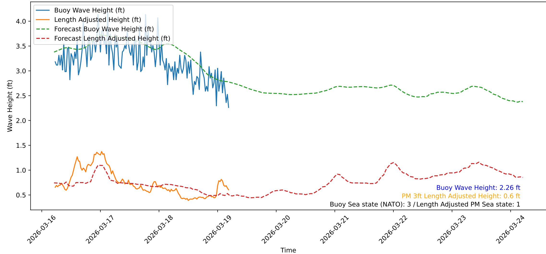
Wave Heights over Time for Green Beach at 2026-03-19 05:21:10
