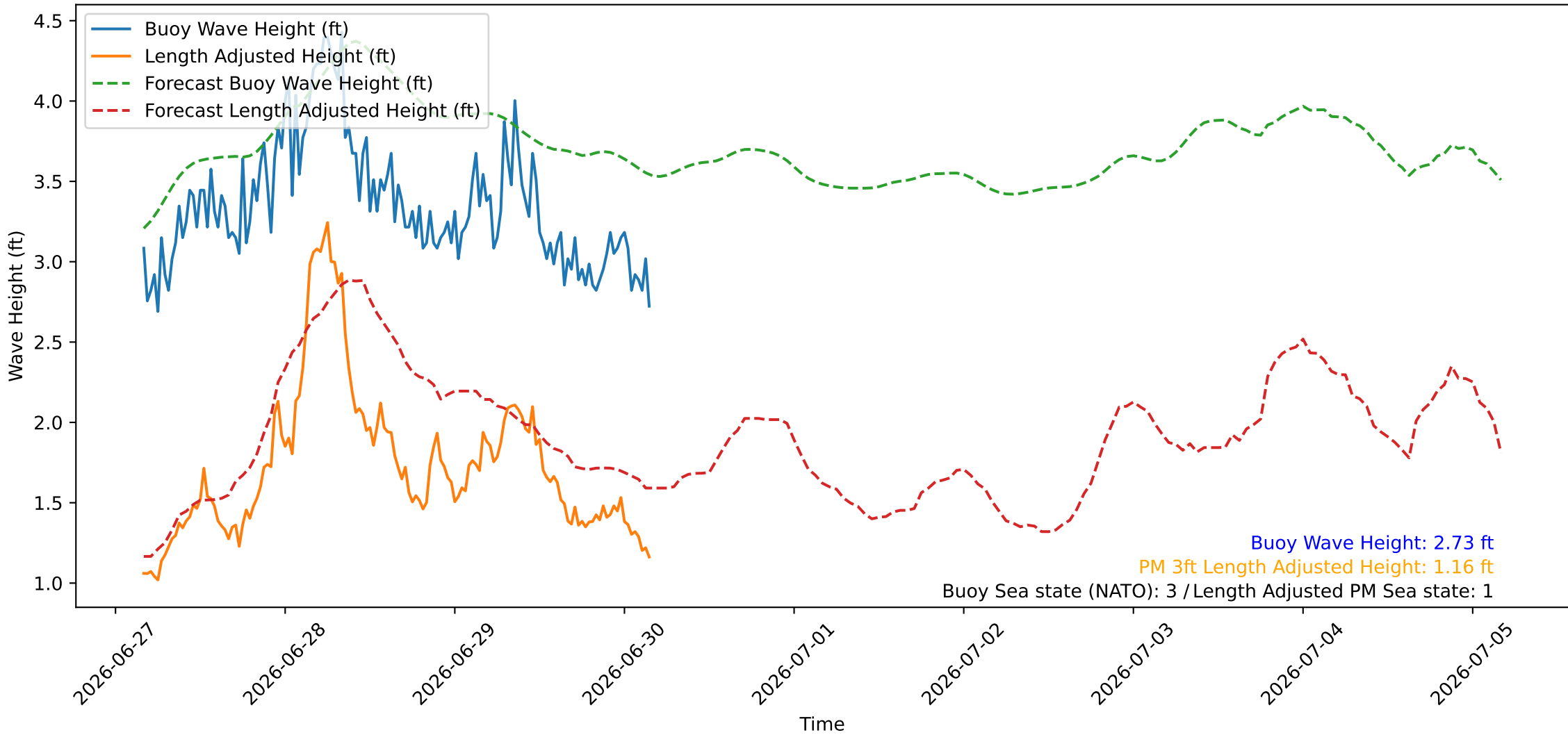
Wave Heights over Time for Oceanside Harbor at 2026-06-30 04:10:26
