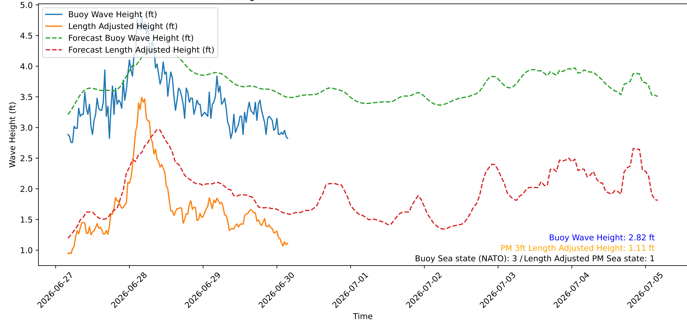
Wave Heights over Time for Green Beach at 2026-06-30 04:11:08
