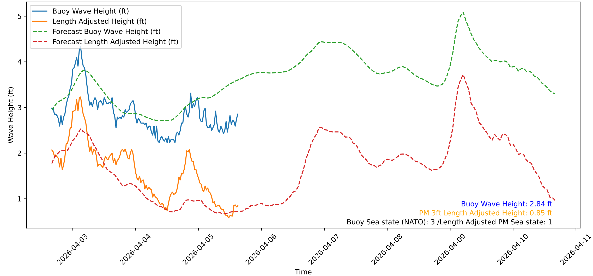
Wave Heights over Time for Green Beach at 2026-04-05 15:51:14
