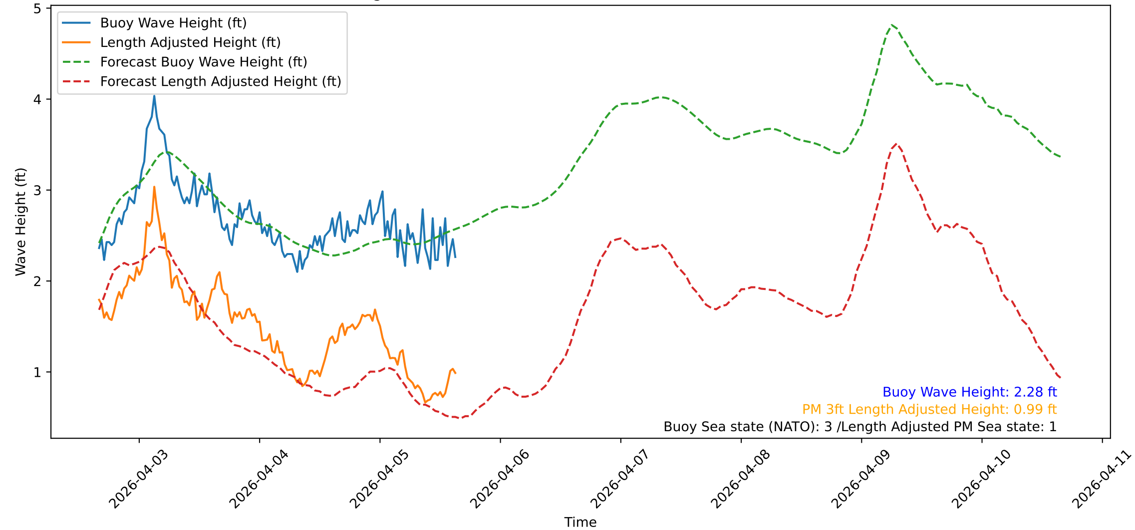
Wave Heights over Time for Oceanside Harbor at 2026-04-05 15:50:33
