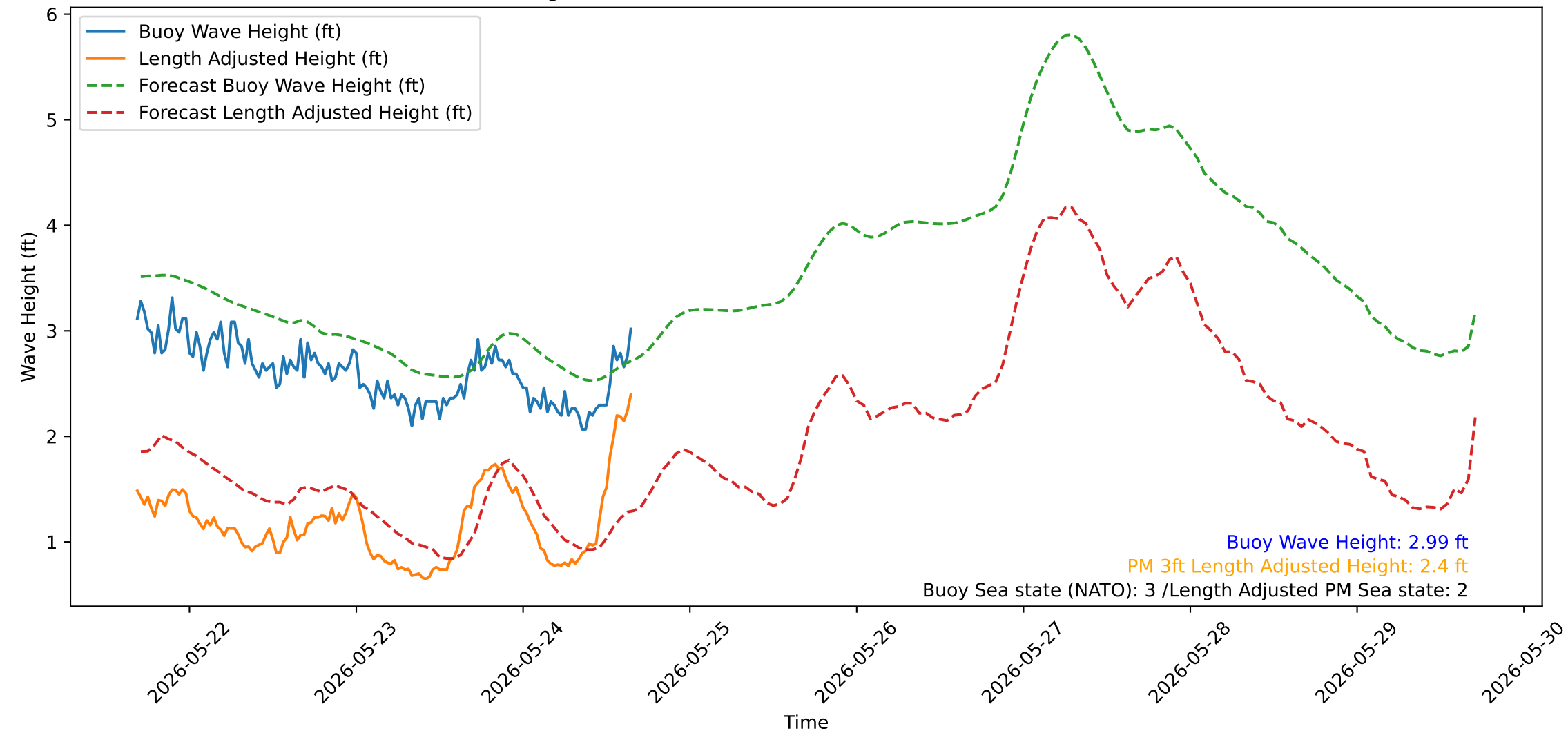
Wave Heights over Time for Green Beach at 2026-05-24 16:31:14
