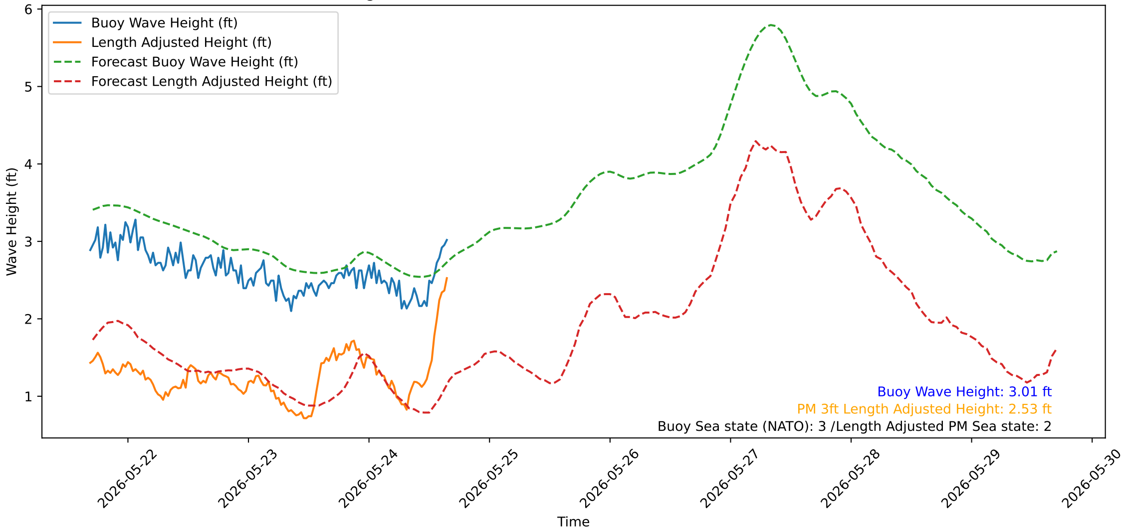
Wave Heights over Time for Oceanside Harbor at 2026-05-24 16:30:31
