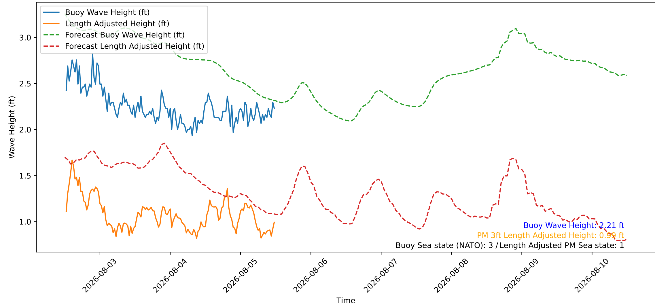
Wave Heights over Time for Green Beach at 2026-08-05 12:21:10
