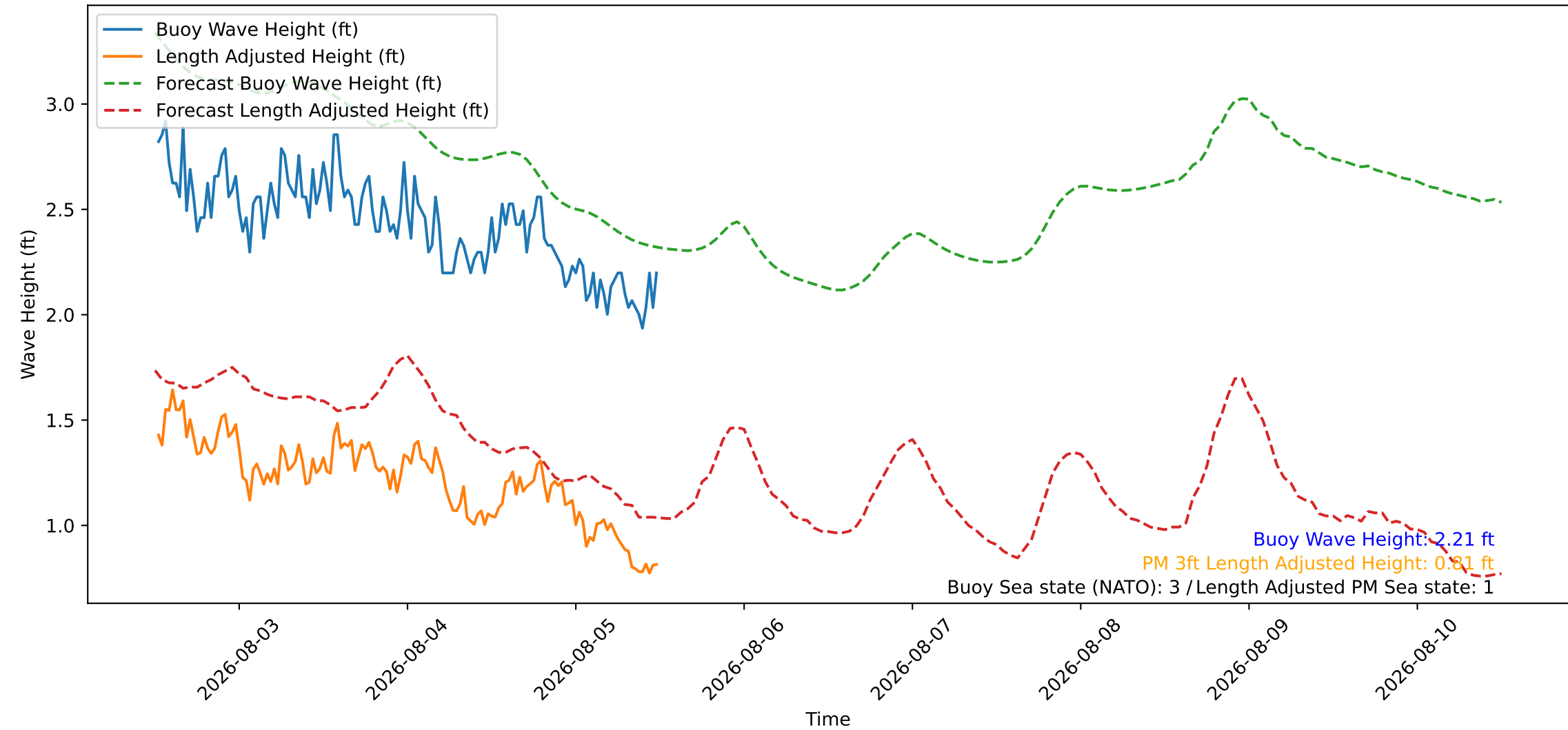
Wave Heights over Time for Oceanside Harbor at 2026-08-05 12:20:27
