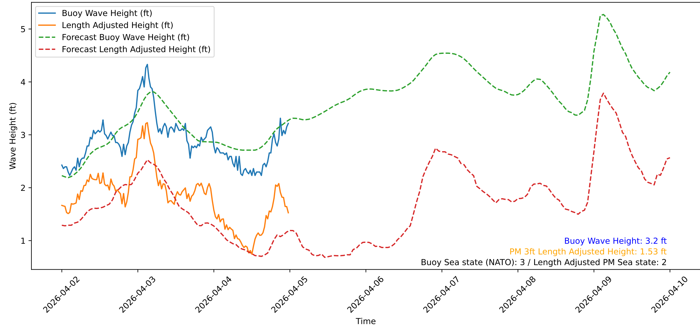
Wave Heights over Time for Green Beach at 2026-04-05 00:11:11
