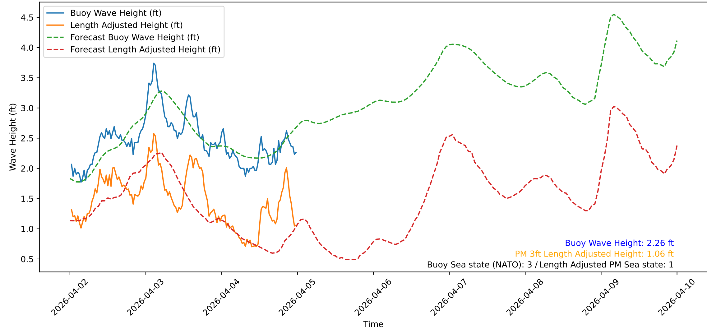
Wave Heights over Time for Red Beach at 2026-04-05 00:10:49
