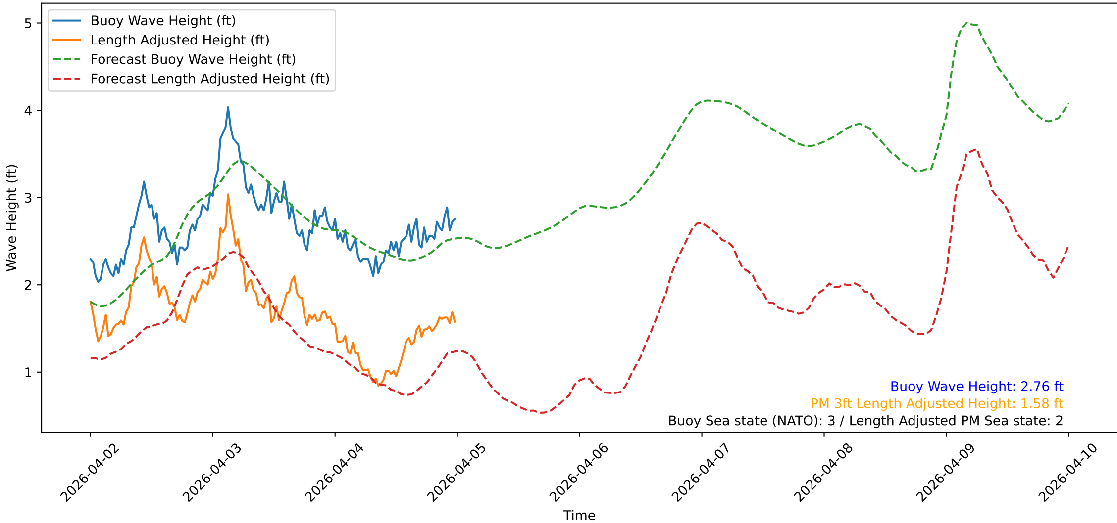
Wave Heights over Time for Oceanside Harbor at 2026-04-05 00:10:32
