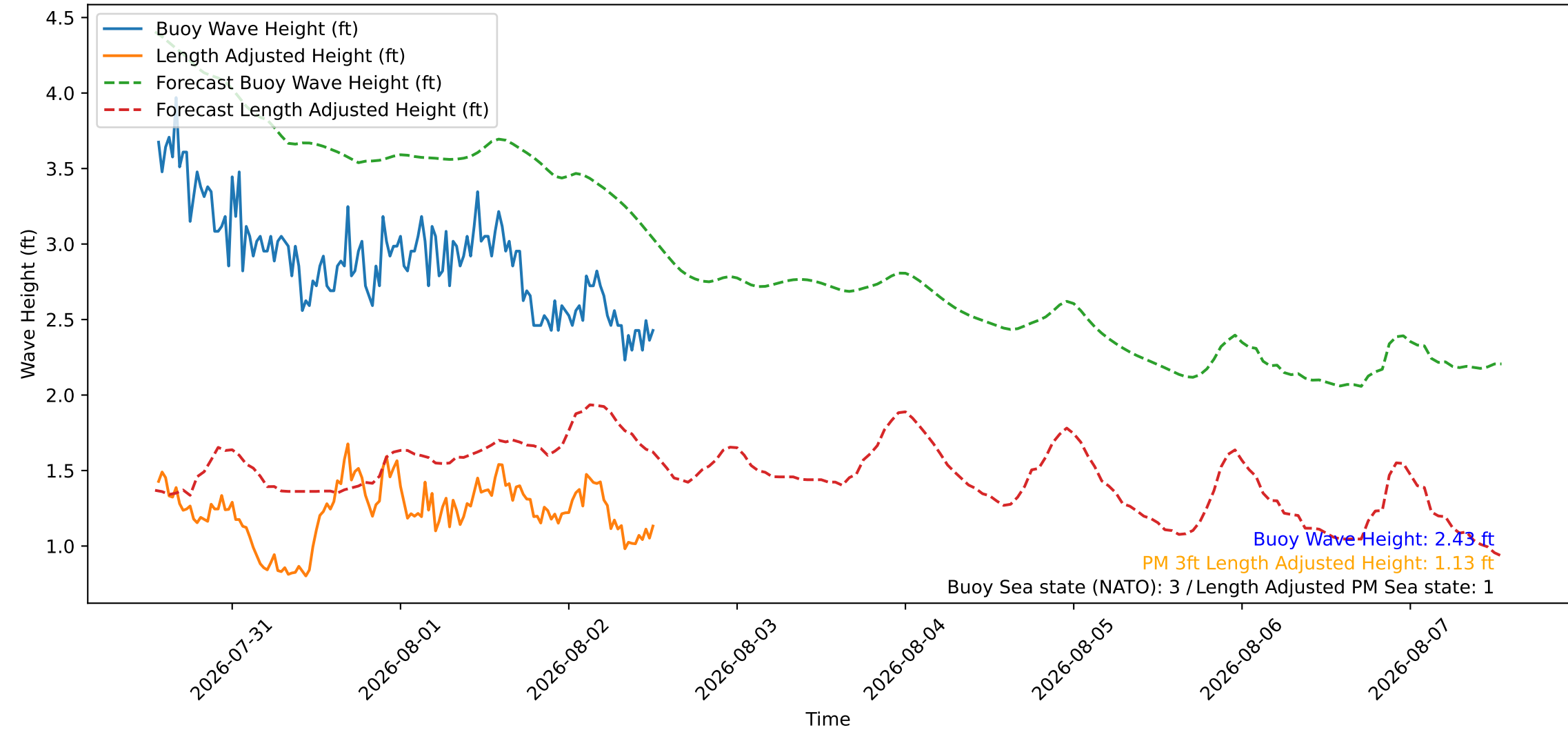
Wave Heights over Time for Red Beach at 2026-08-02 13:20:46
