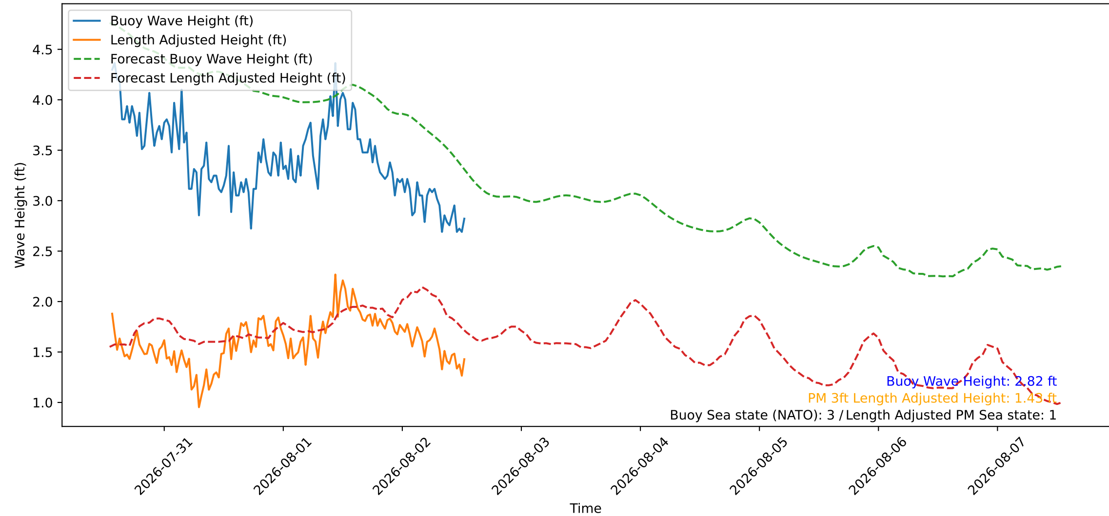
Wave Heights over Time for Oceanside Harbor at 2026-08-02 13:20:26
