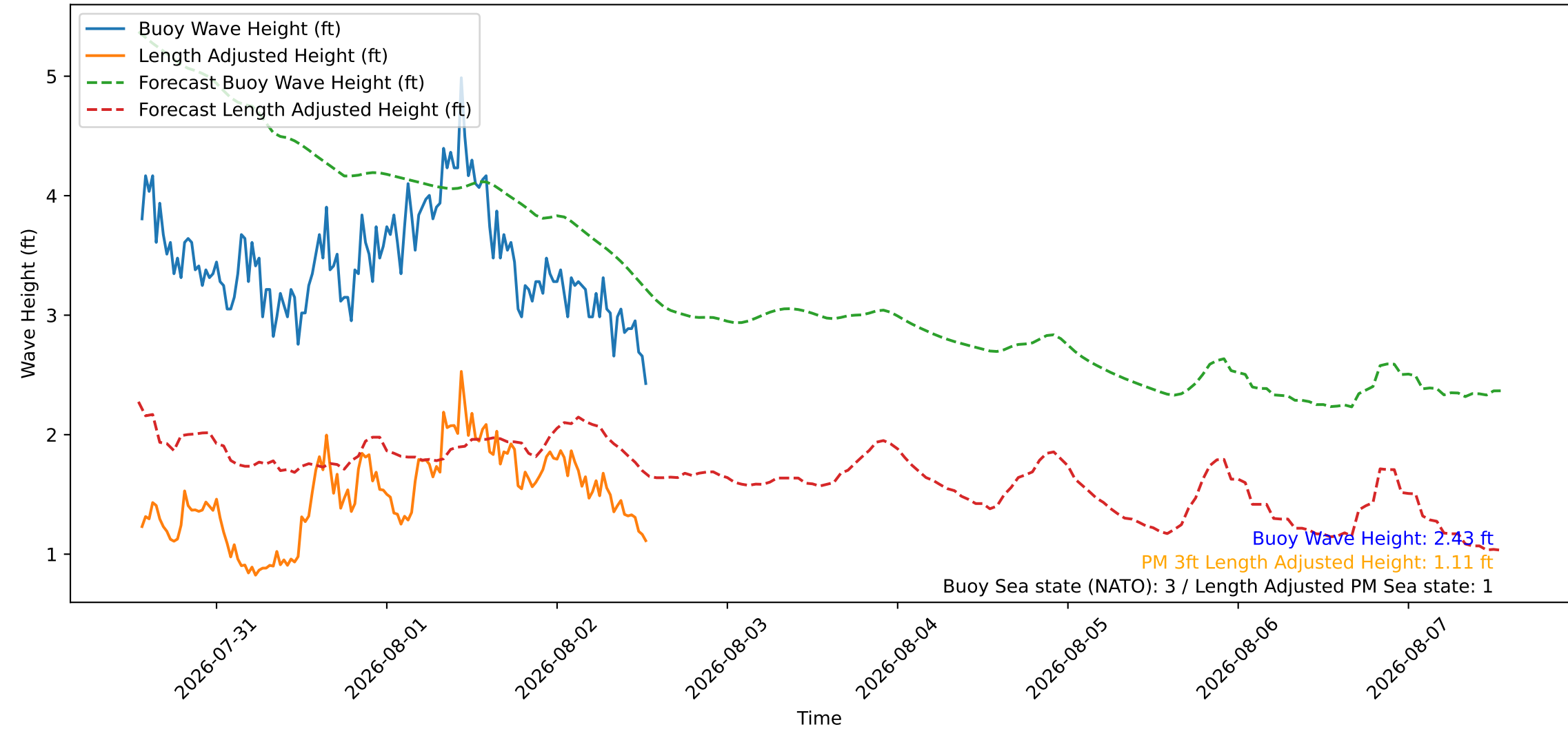
Wave Heights over Time for Green Beach at 2026-08-02 13:21:08
