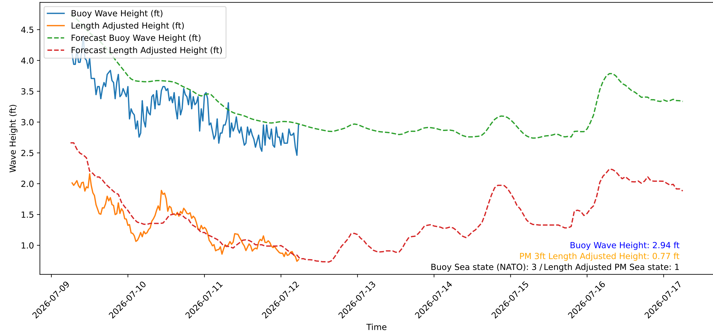
Wave Heights over Time for Green Beach at 2026-07-12 06:21:10
