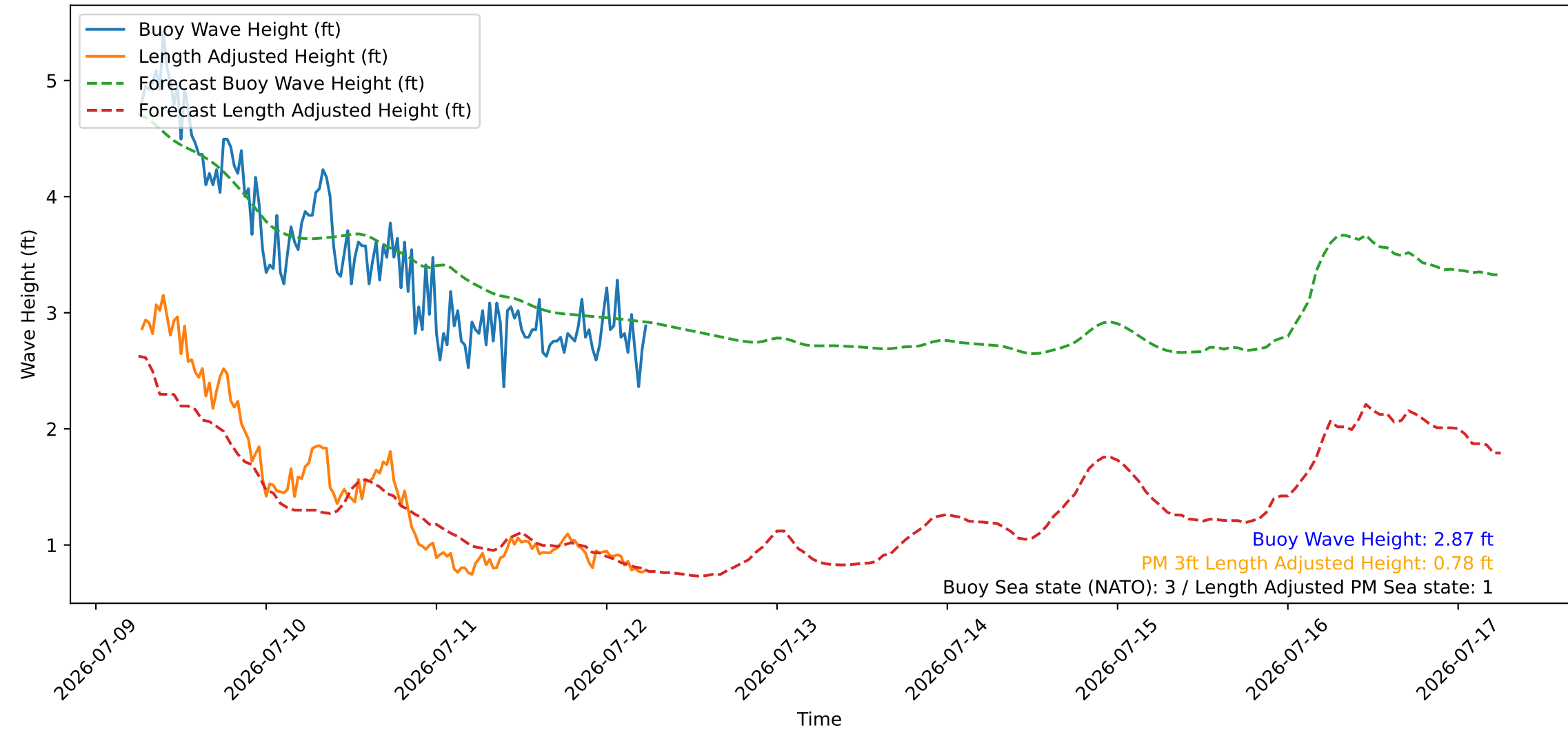
Wave Heights over Time for Oceanside Harbor at 2026-07-12 06:20:27
