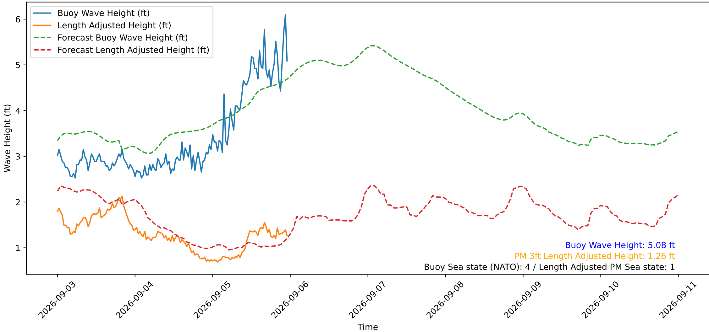
Wave Heights over Time for Red Beach at 2026-09-05 23:40:49
