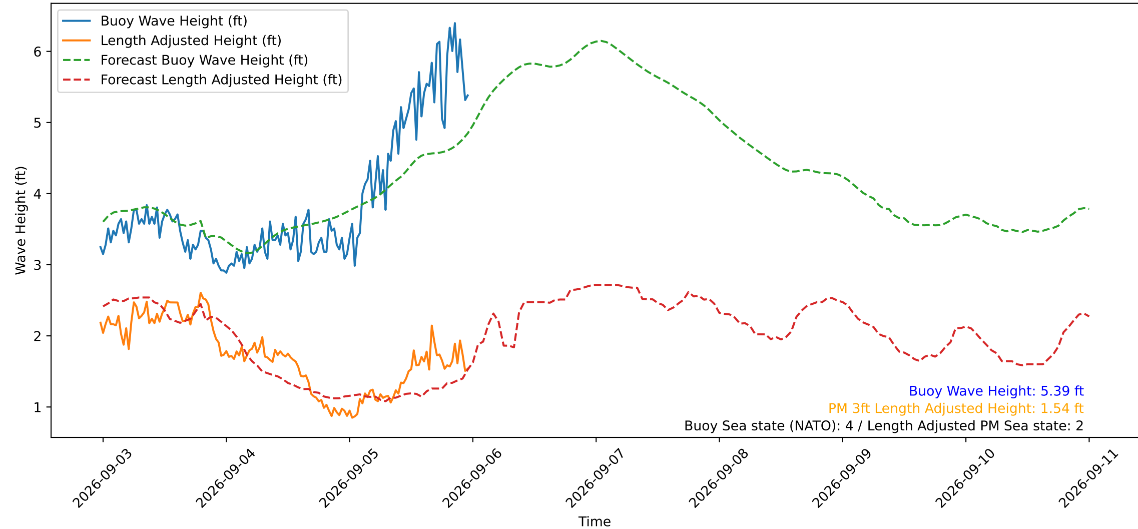
Wave Heights over Time for Oceanside Harbor at 2026-09-05 23:40:29
