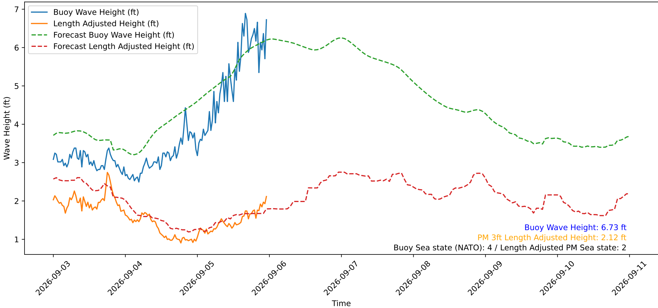
Wave Heights over Time for Green Beach at 2026-09-05 23:41:12
