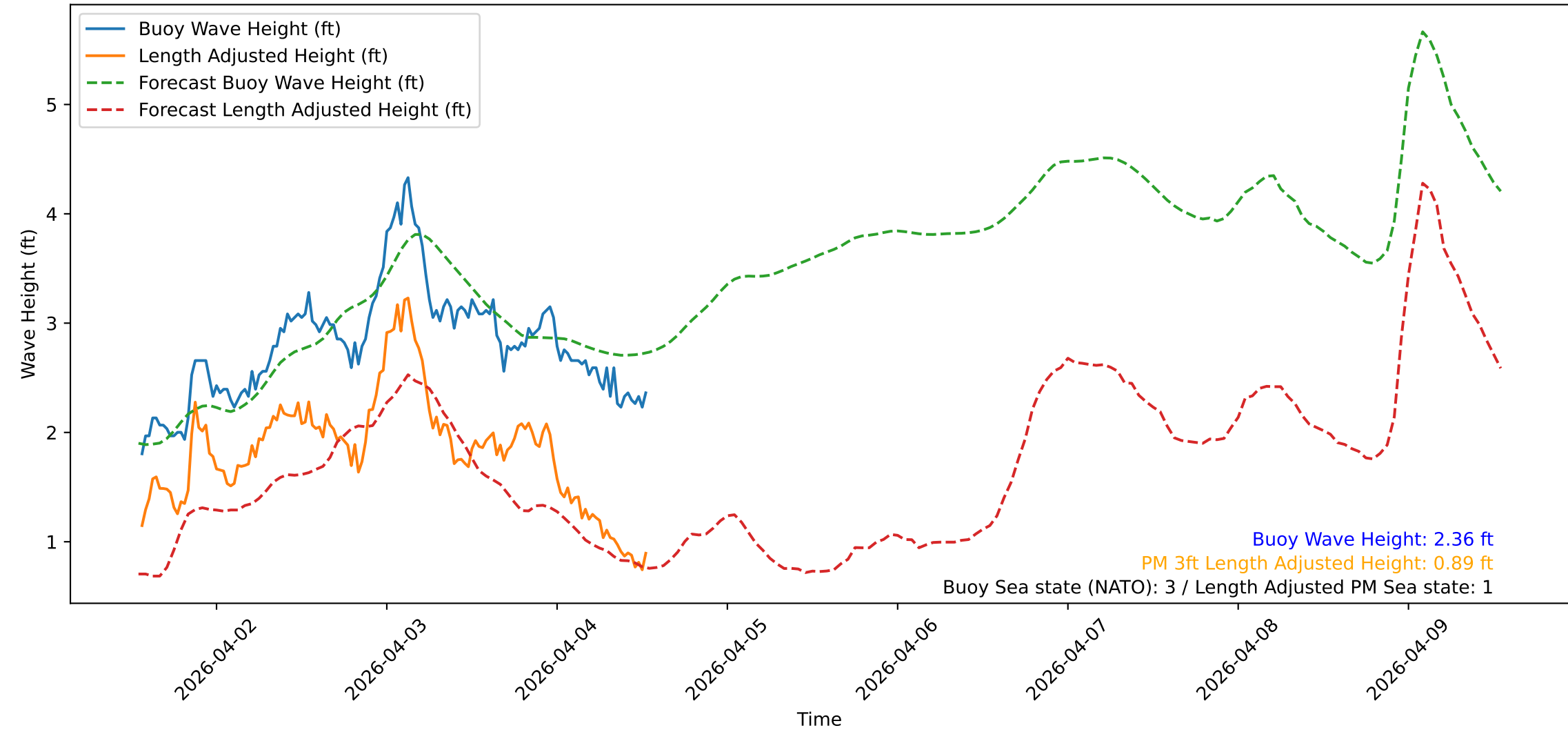
Wave Heights over Time for Green Beach at 2026-04-04 13:21:10
