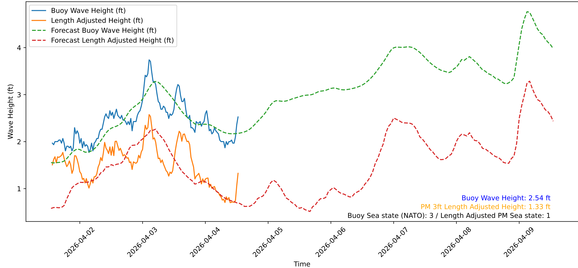
Wave Heights over Time for Red Beach at 2026-04-04 13:20:48
