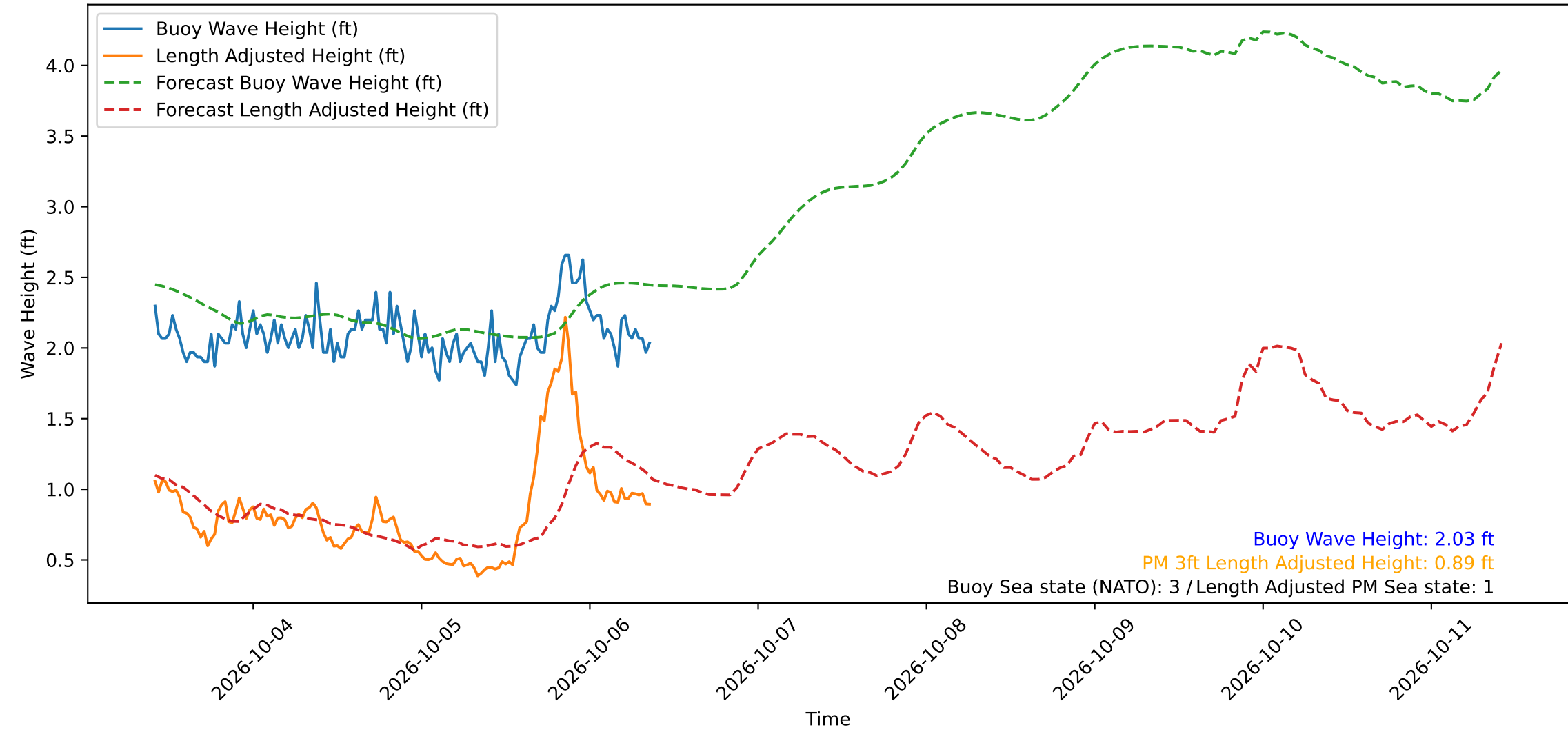
Wave Heights over Time for Red Beach at 2026-10-06 09:30:50
