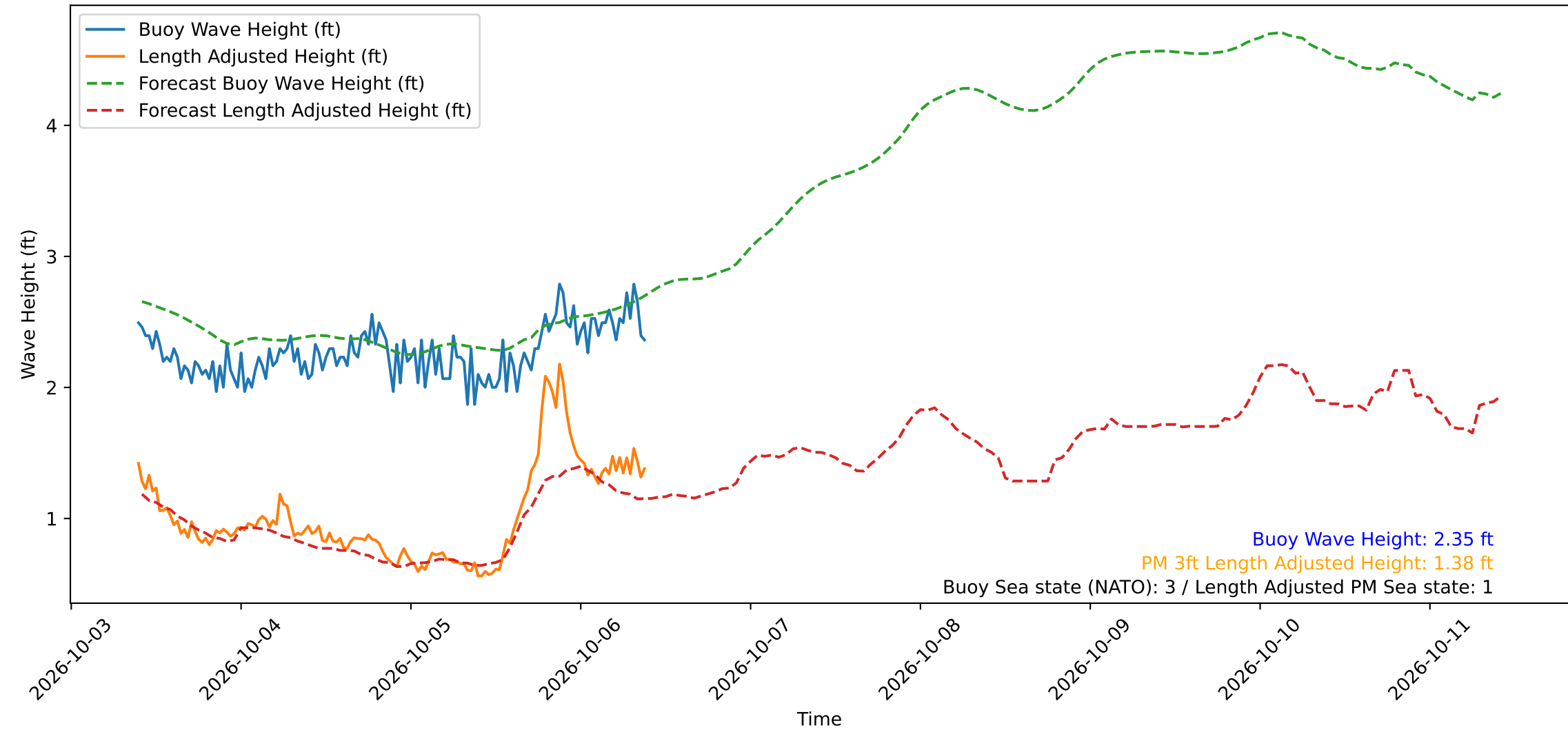
Wave Heights over Time for Oceanside Harbor at 2026-10-06 09:30:31
