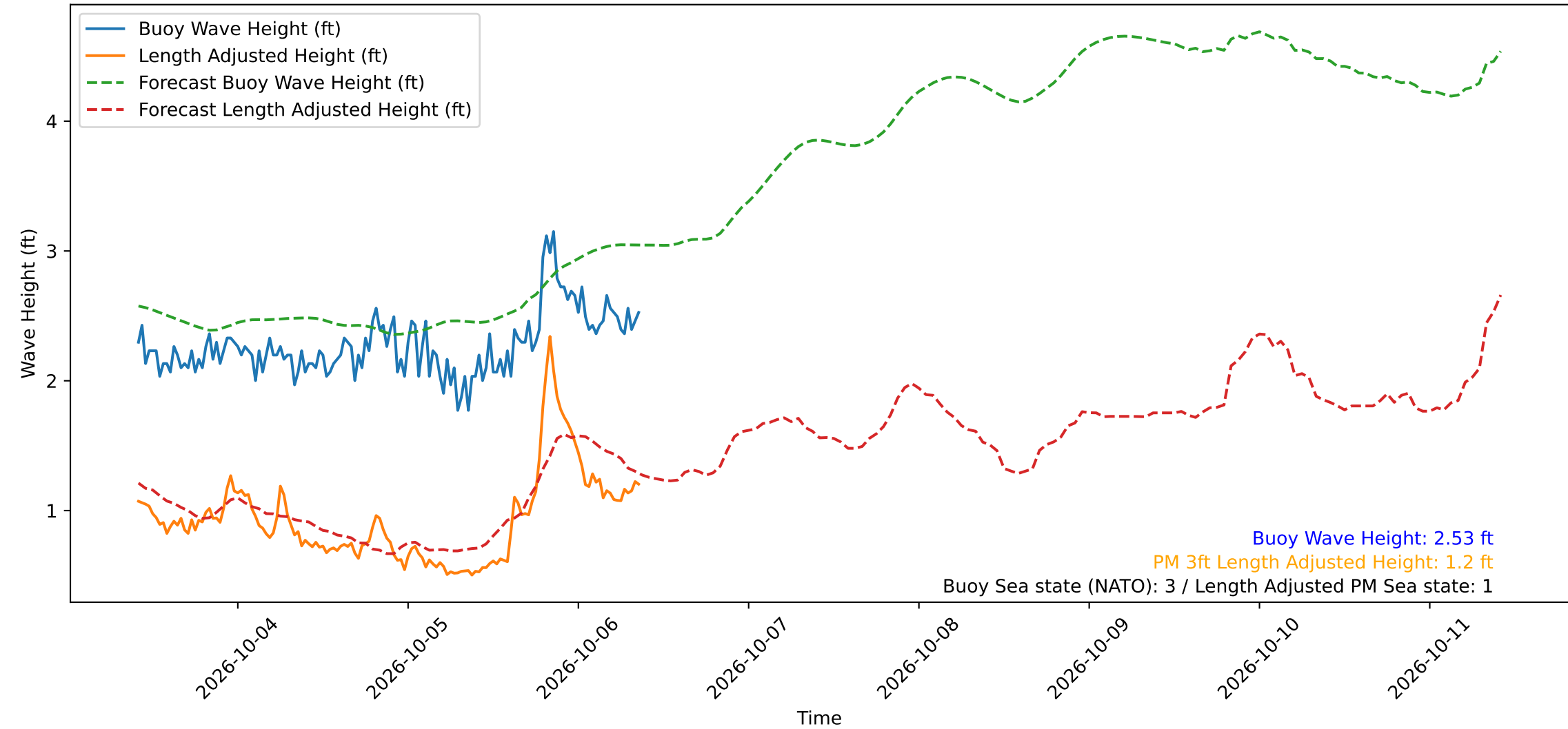
Wave Heights over Time for Green Beach at 2026-10-06 09:31:13
